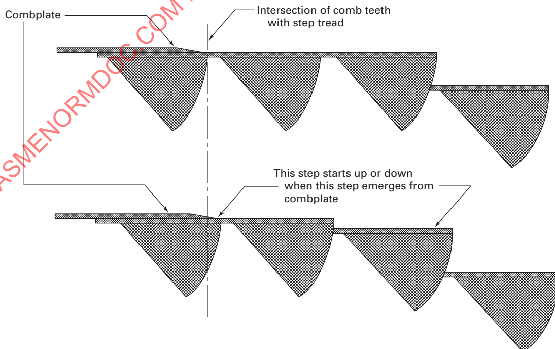
Fig. 7.9.3 Example of Two Flat Steps
