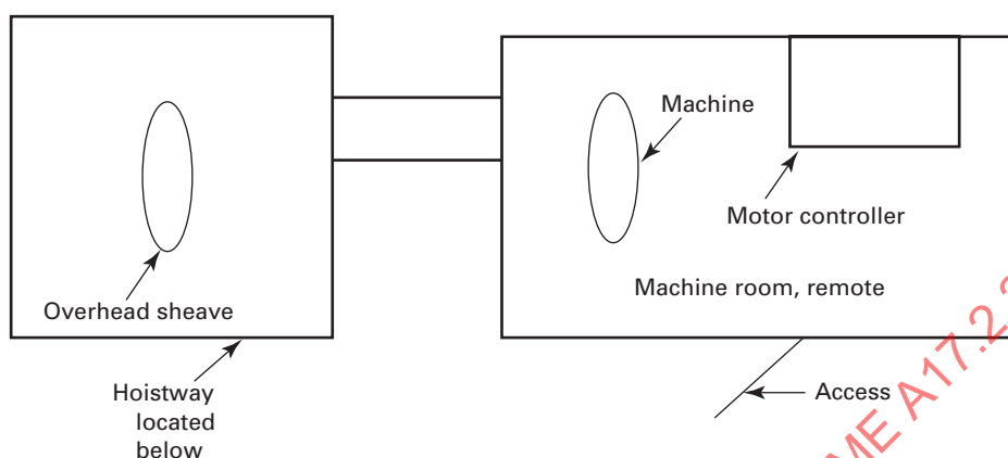
Fig. 11.21-6 Configuration F
