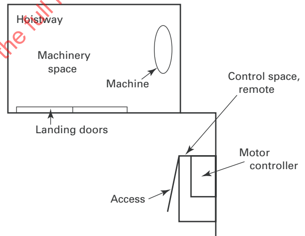
Fig. 11.21-3 Configuration C
