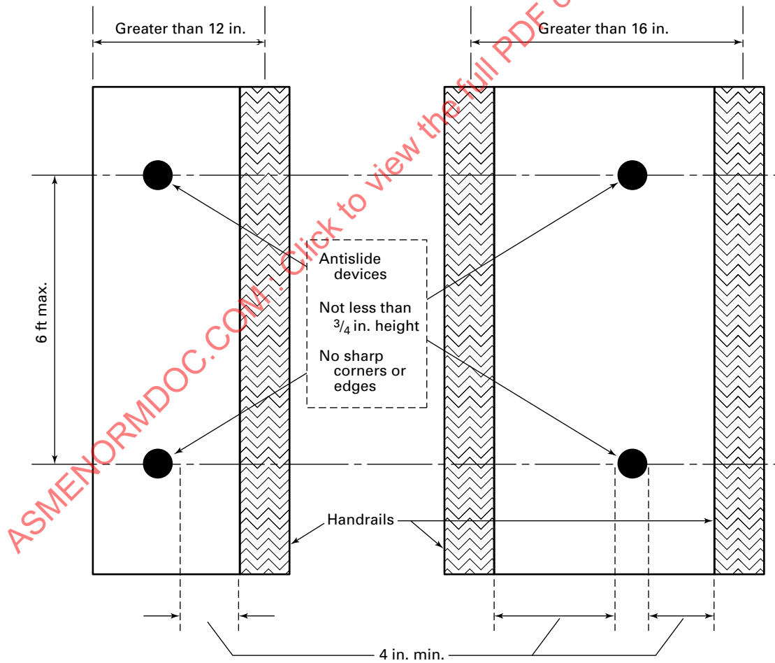
Figure 7.8.1(b) High-Deck Balustrade Antislip Devices
