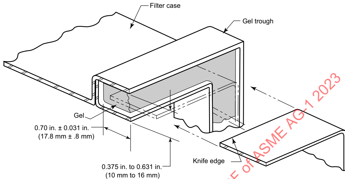
Figure FC-4142-1 Gel Seal Filter Corner — Isometric
