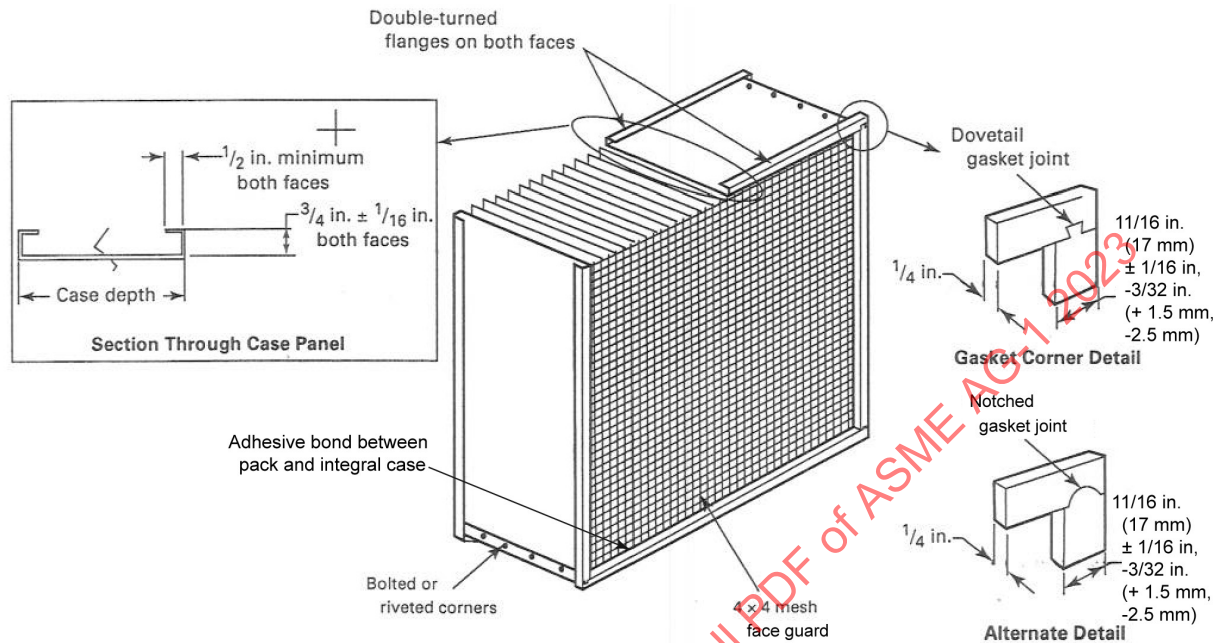
Figure FM-4110-1 Type A Metal Case Separator Filter
