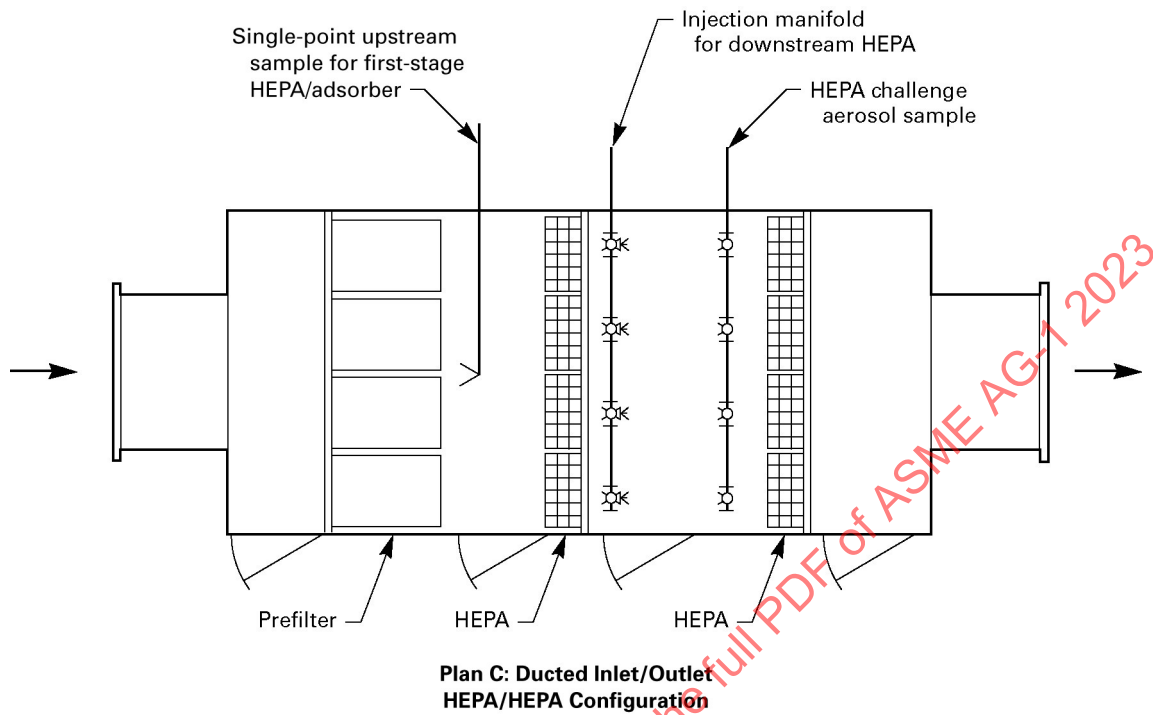
Figure HA-C-1230-3 Common Configurations Requiring Test Manifolds (Plan C)
