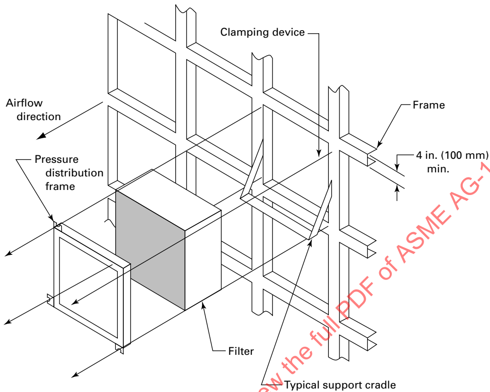
Figure FG-4110-1 Typical Filter Mounting Frame
