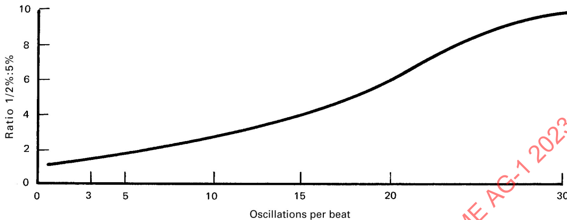
Figure AA-4356.4-1 Oscillations per Beat
