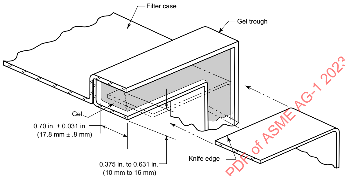
Figure FM-4142-1 Gel Seal Filter Corner — Isometric
