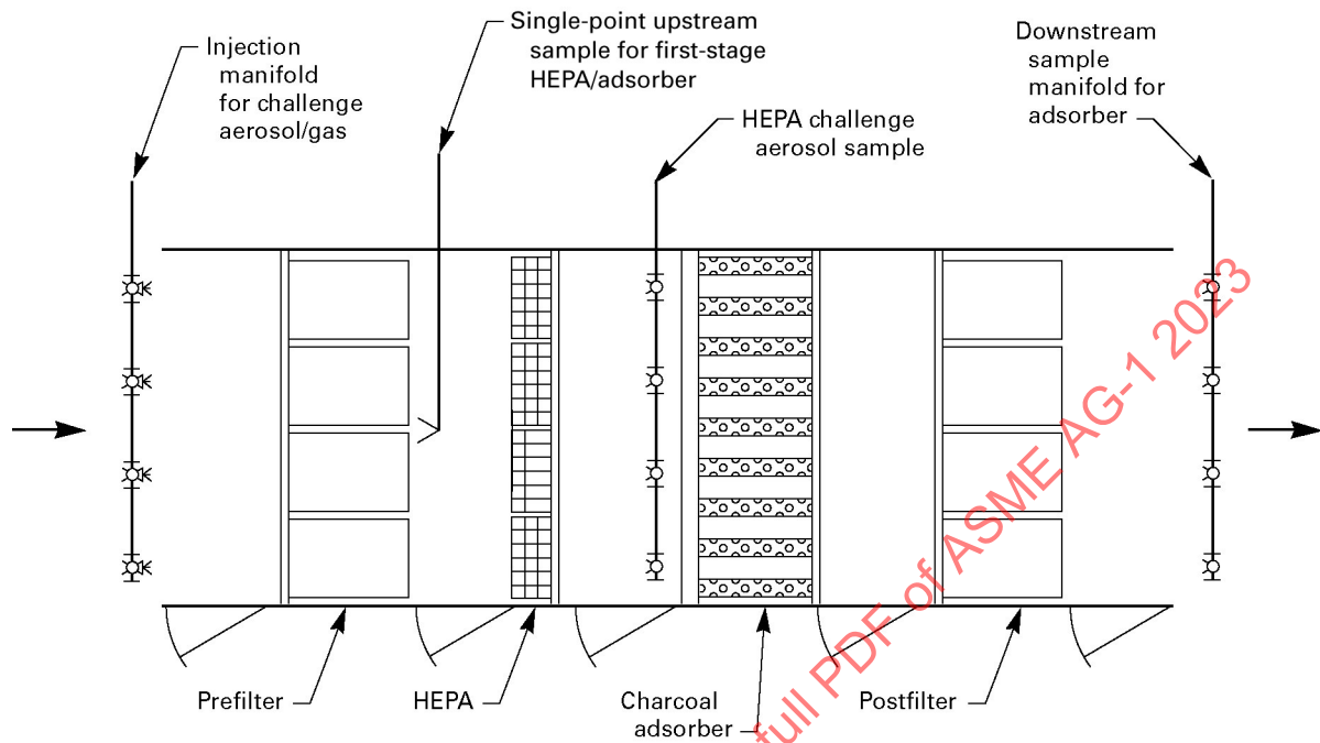
Plan B: Unducted Inlet/Outlet HEPA/Adsorber Configuration
