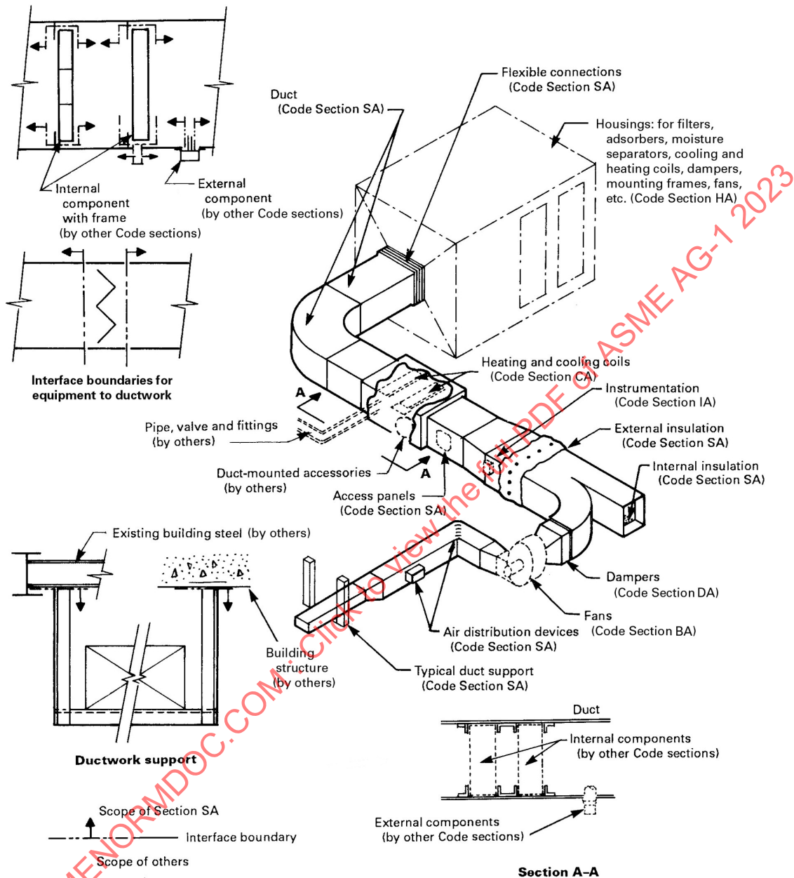
Figure SA-1300-1 Ductwork and Ductwork Support — Interface Boundary
