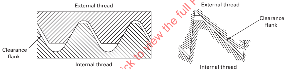
Fig. 6 Clearance Flank
