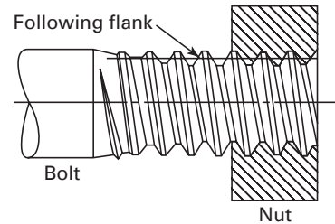
Fig. 16 Following Flank
