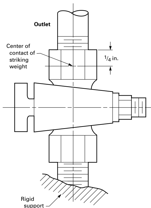
Fig. 1 Test Device
