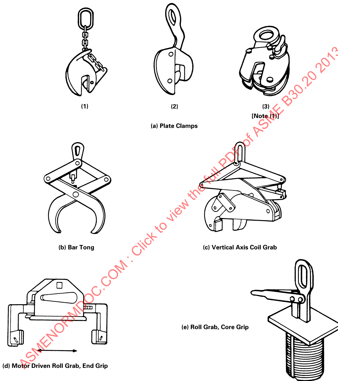
Fig. 20-0.3-1 Pressure-Gripping Lifters: Friction-Type Lifters
