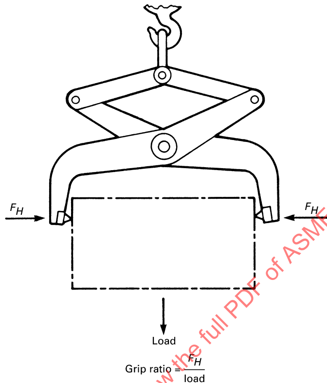
Fig. 20-0.3-2 Grip Ratio
