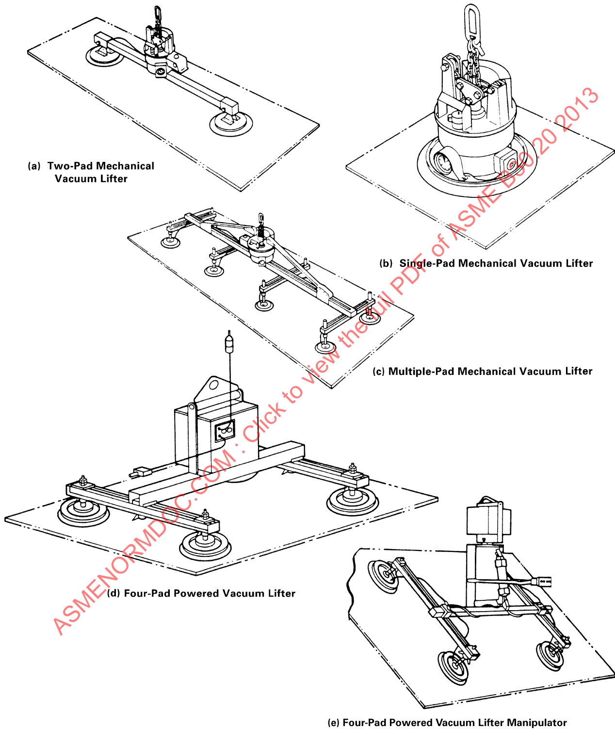
Fig. 20-0.4-1 Vacuum Lifters
