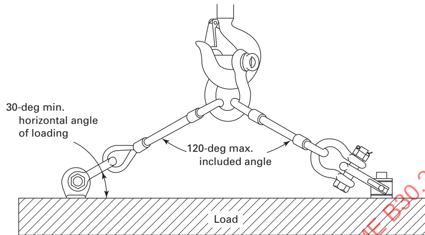
Fig. 26-1.9.1-1 Angle of Loading (Shackles)
