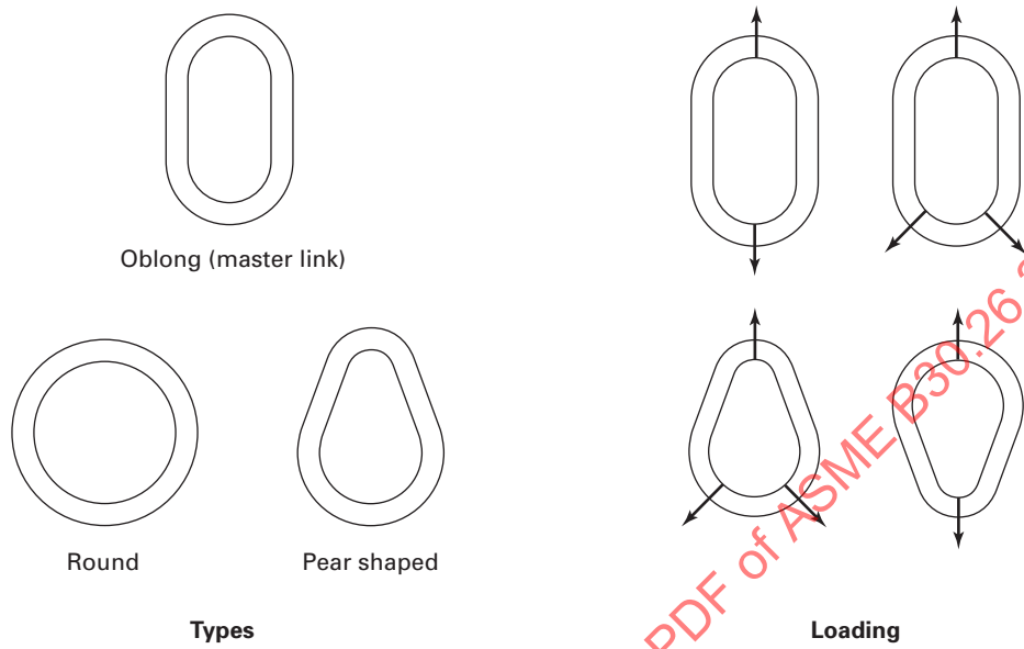
Fig. 26-4.1.1-1 Links and Rings
