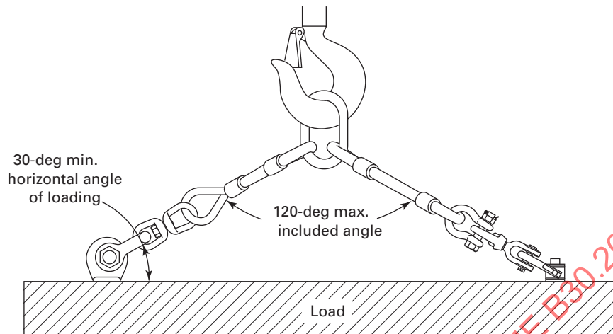
Fig. 26-4.9.1-1 Angle of Loading (Links, Rings, and Swivels)
