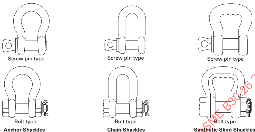
Fig. 26-1.1.1-1 Shackle Types
