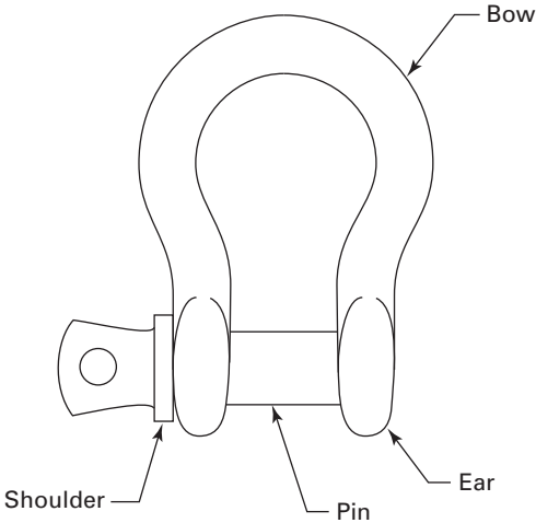
Fig. 26-1.9.4-1 Typical Shackle Components
