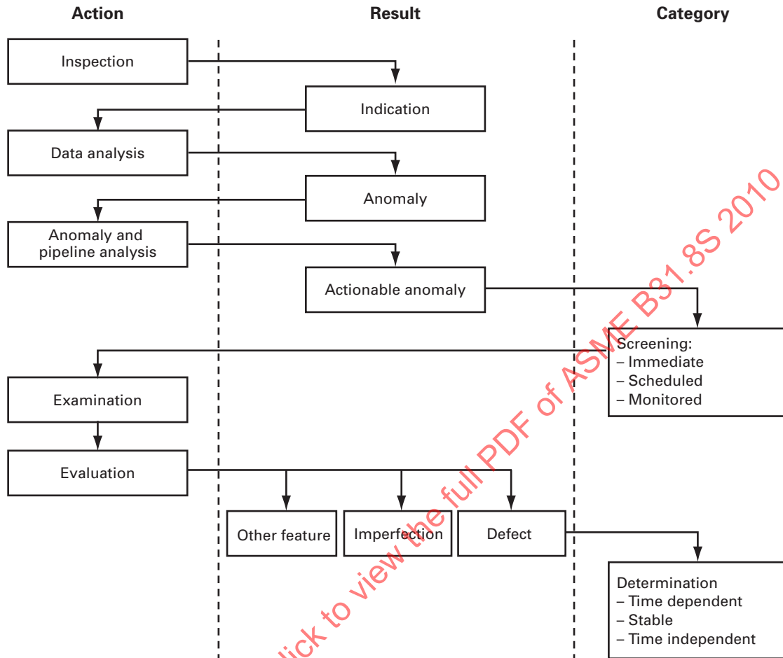
Fig. 5 Hierarchy of Terminology for Integrity Assessment
