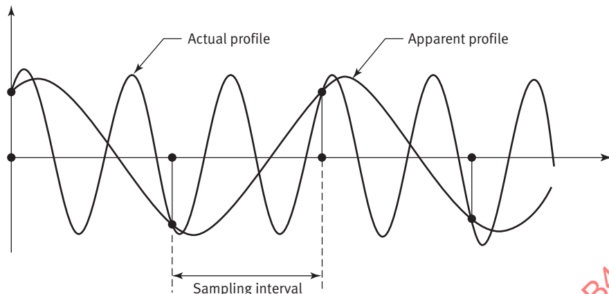
Fig. 3-4 Aliasing
