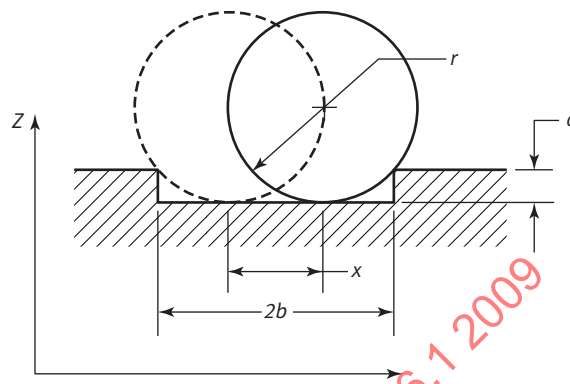
Fig. 7-3 The Stylus Tip Contact Distance, x
