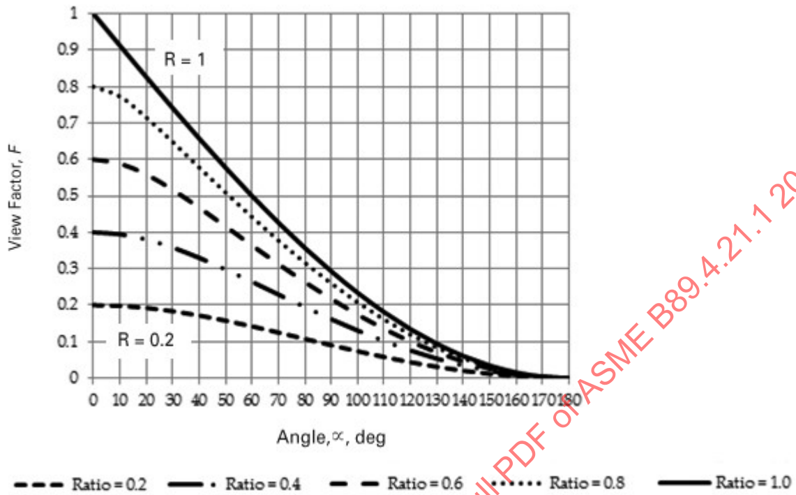
Figure D-6-3 Values of F_{1-2} for Assumed Values of the Ratio and Angle
