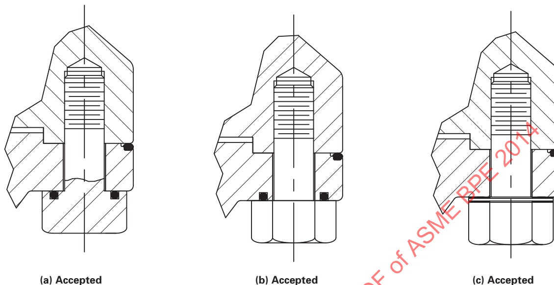
Fig. SD-3.5.2-3 Fastener Seal Arrangements
