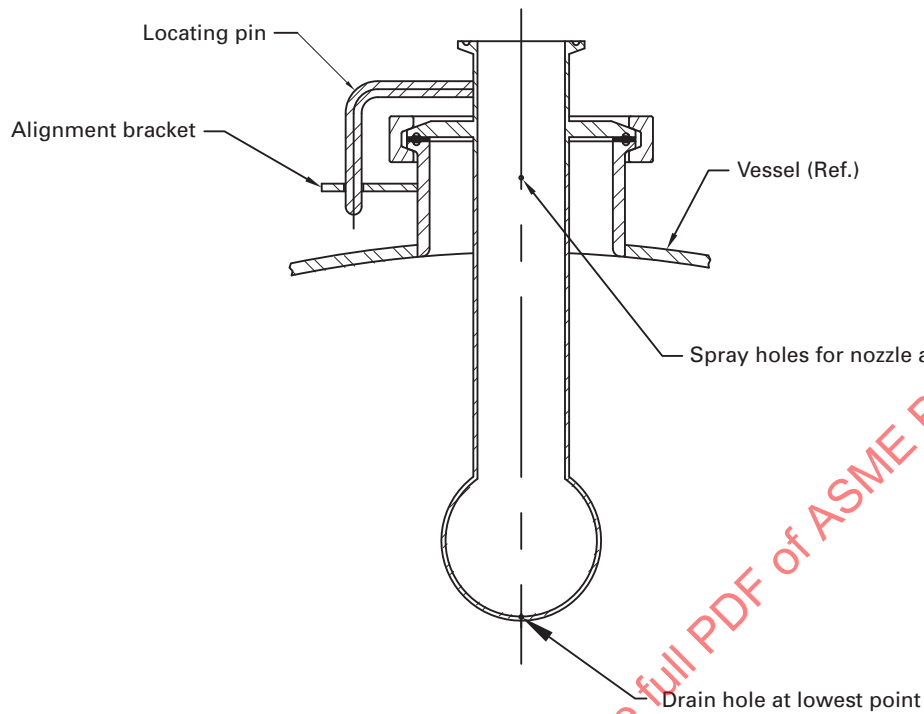
Fig. SD-3.9.2.1-1 Static Spray Device
