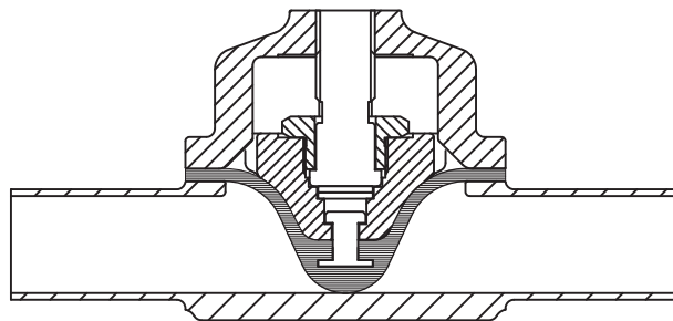
Fig. SG-2.3.1.2-3 Weirless Diaphragm Valve
