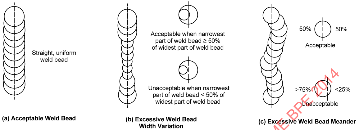
Fig. MJ-8.4-4 Acceptable and Unacceptable Weld Bead Width and Meander
