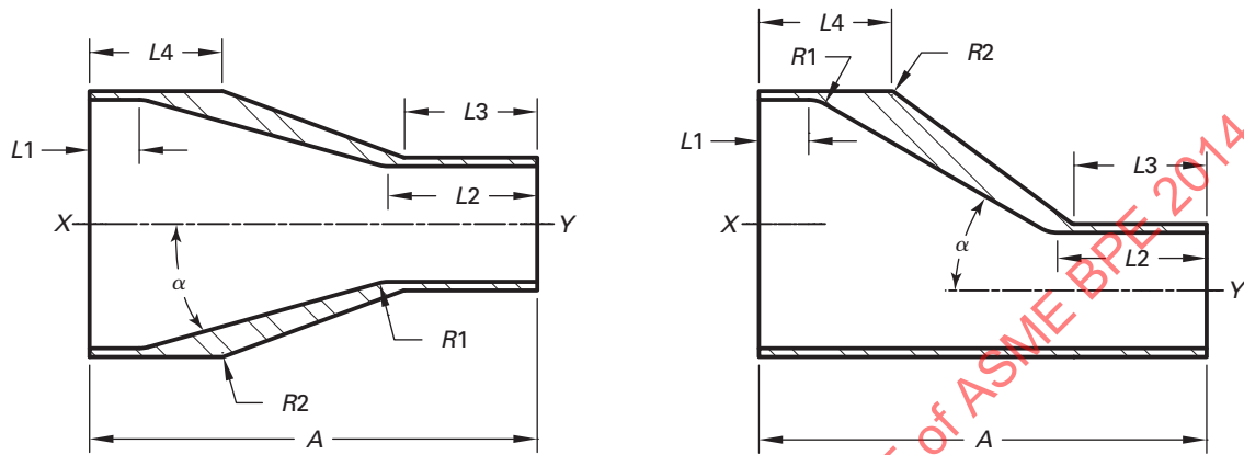
(14) Table DT-4.1.3-1 Automatic Tube Weld: Concentric and Eccentric Reducer
