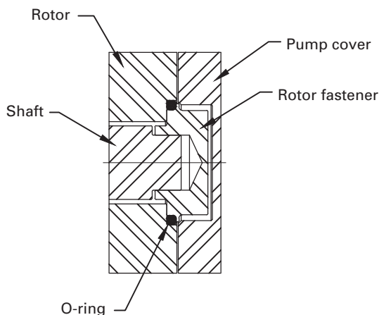
(14) Fig. SD-3.3.2.4-1 Rotary Lobe Pump Rotor Attachment
