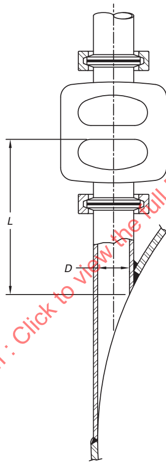
Fig. SD-3.4.2-5 Vessel Design Tangential Nozzles
