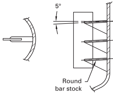
(a) Hygienic Design (Accepted: Sloped, Minimum Shadow, and Curved Surface)
