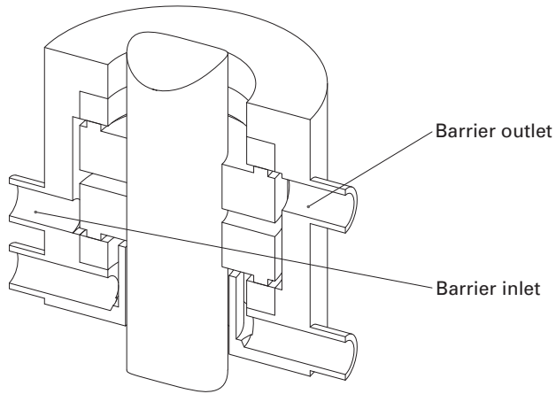
Fig. SG-2.3.2.4-12 Flush Plan 54 for Top Entry Agitator
