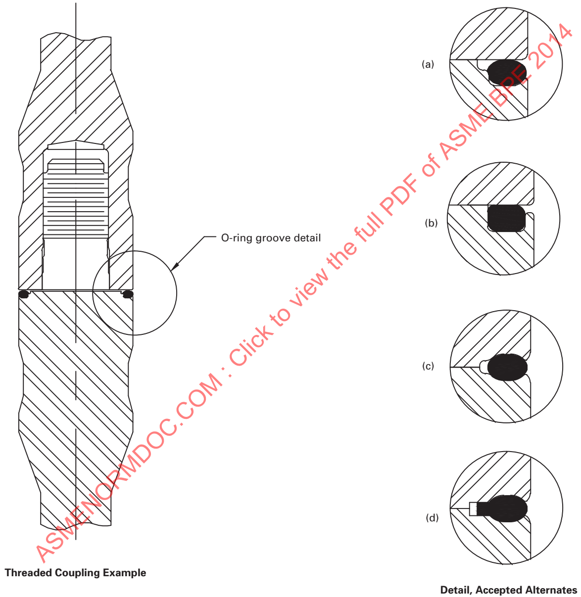
Fig. SD-3.5.2-2 Shaft Coupling Seal Arrangements
