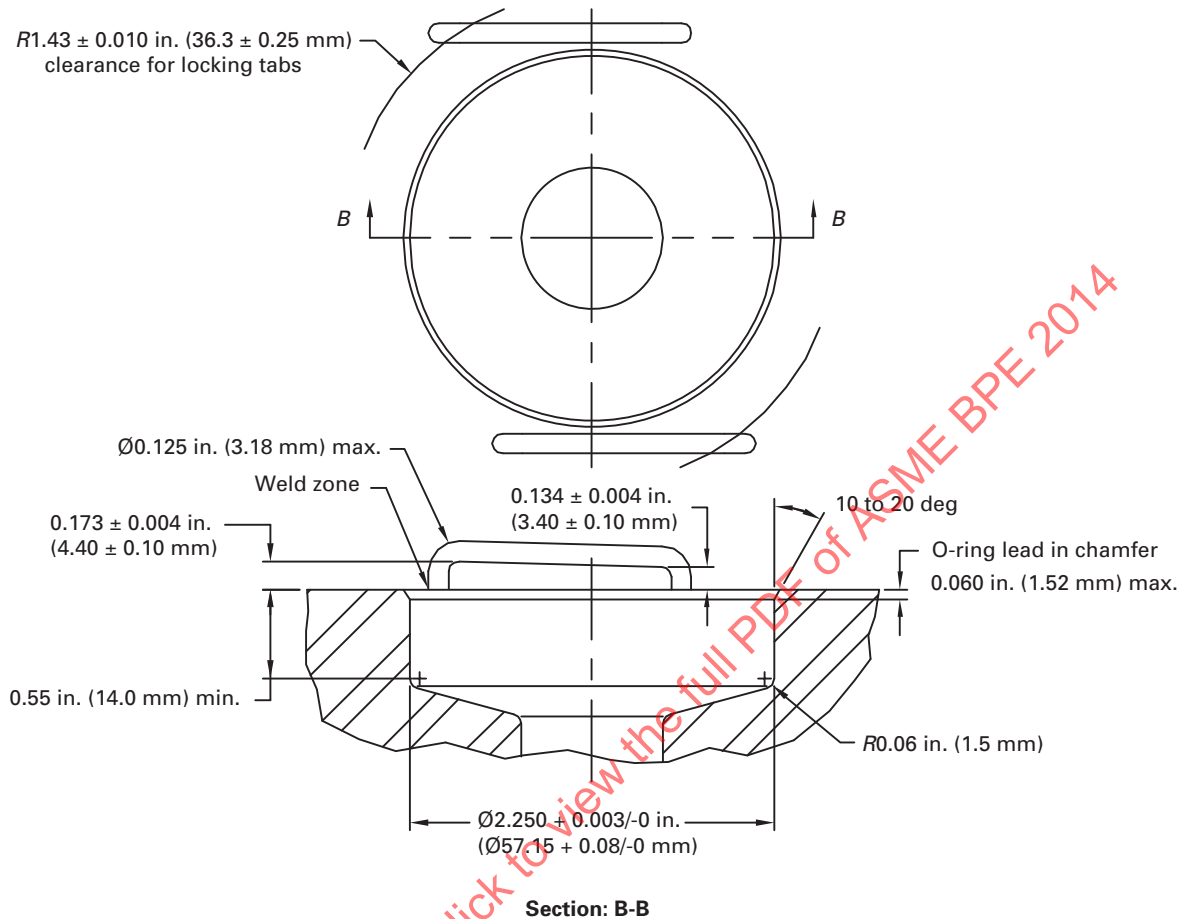
Fig. SD-3.8.1.1-2 Tapered Locking Tab Retainer — External
