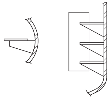
Fig. SD-3.4.3-1 Internal Support Members
