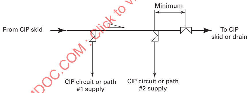
Fig. SD-5.3.3.5.1-2 Zero-Static Chain
