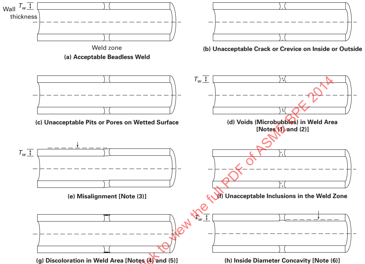
Fig. MJ-9.7.1-1 Acceptable and Unacceptable Weld Profiles for Beadless Welds
