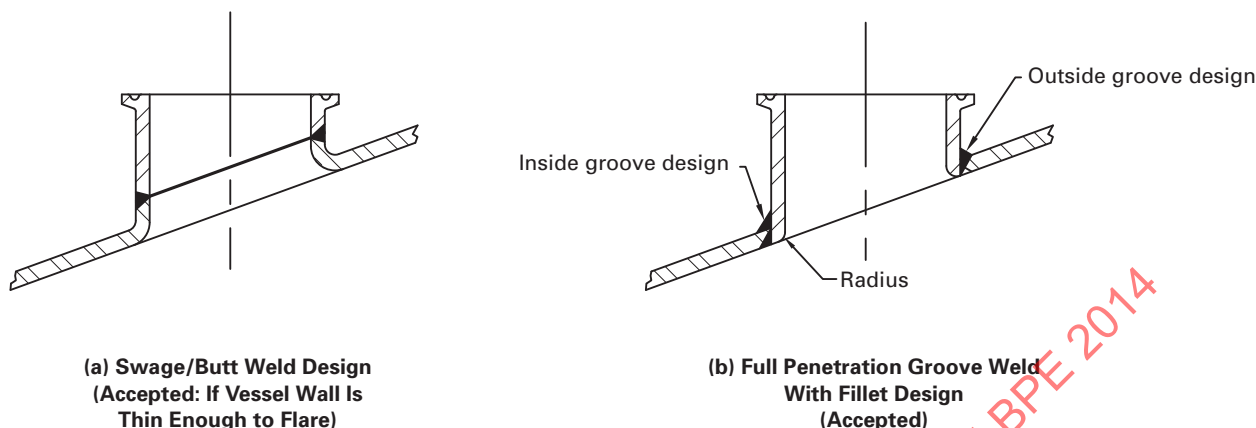
Fig. SD-3.4.2-7 Typical Nozzle Detail
