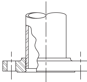
(g) Threaded
