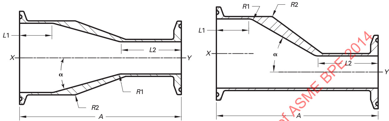
(14) Table DT-4.1.3-3 Hygienic Clamp Joint: Concentric and Eccentric Reducer
