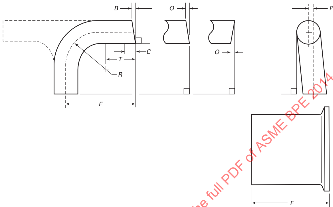
(14) Table DT-3-1 Final Tolerances for Mechanically Polished Fittings and Process Components
