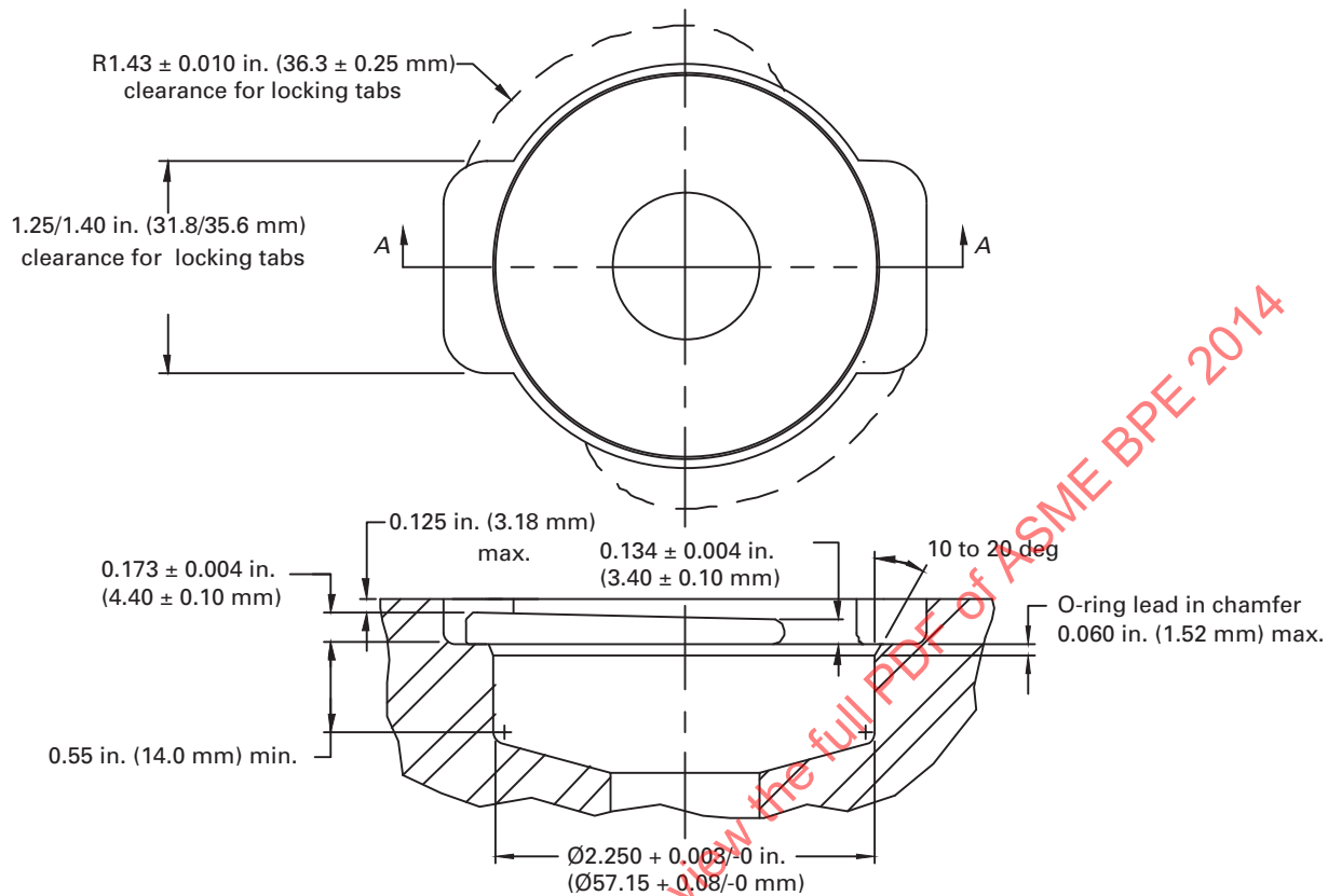
Fig. SD-3.8.1.1-1 Tapered Locking Tab Retainer — Recessed
