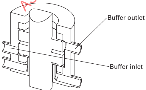
(14) Fig. SG-2.3.2.4-14 Flush Plan 55 for Top Entry Agitator
