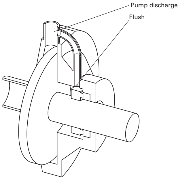
Fig. SG-2.3.2.4-4 Flush Plan 11
