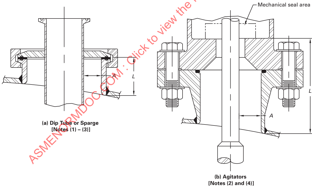
Fig. SD-3.4.2-4 Accepted Nozzle Penetrations
