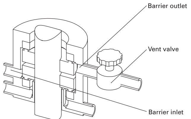
Fig. SG-2.3.2.4-16 Flush Plan 74 for Top Entry Agitator
