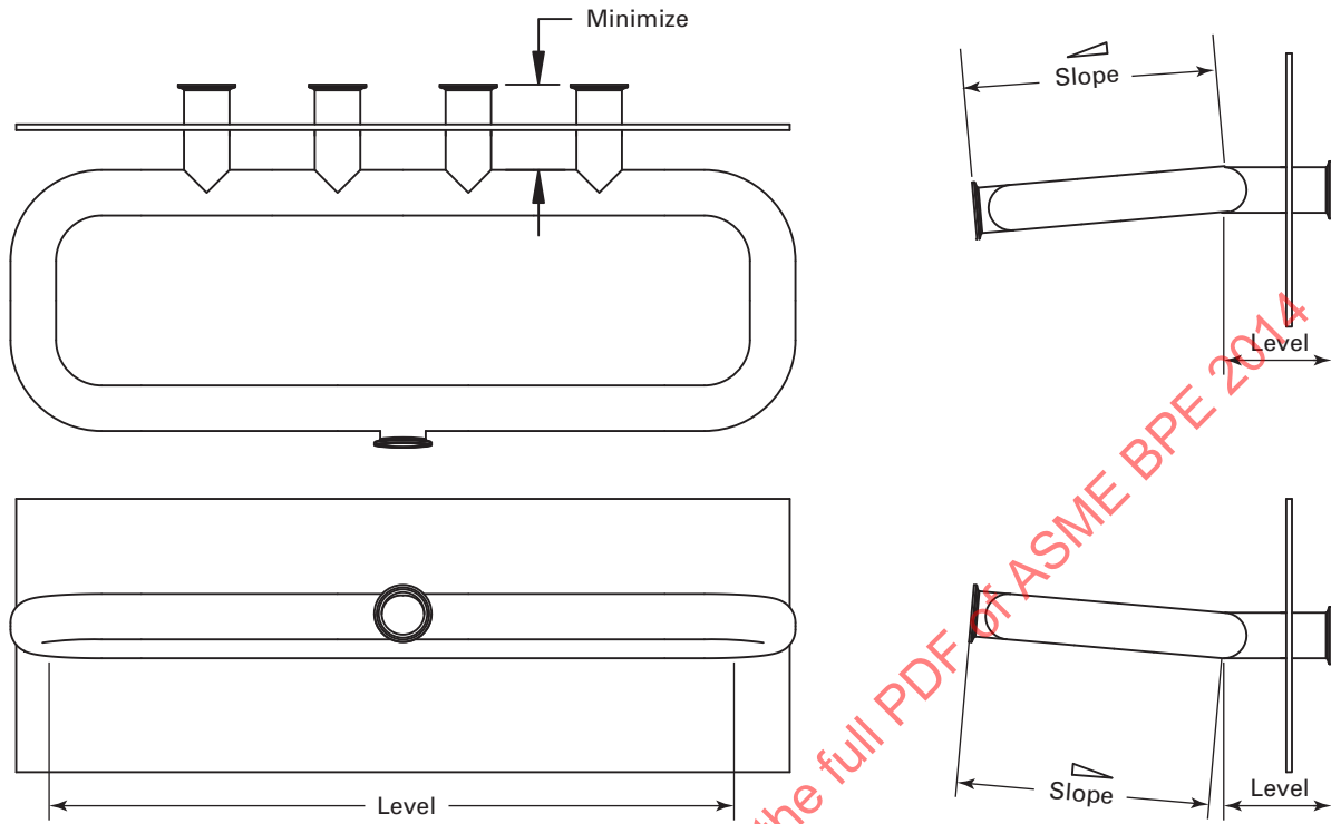
Fig. SD-3.7.1-1 Transfer Panel Looped Headers
