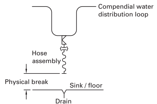
(e) Hose
