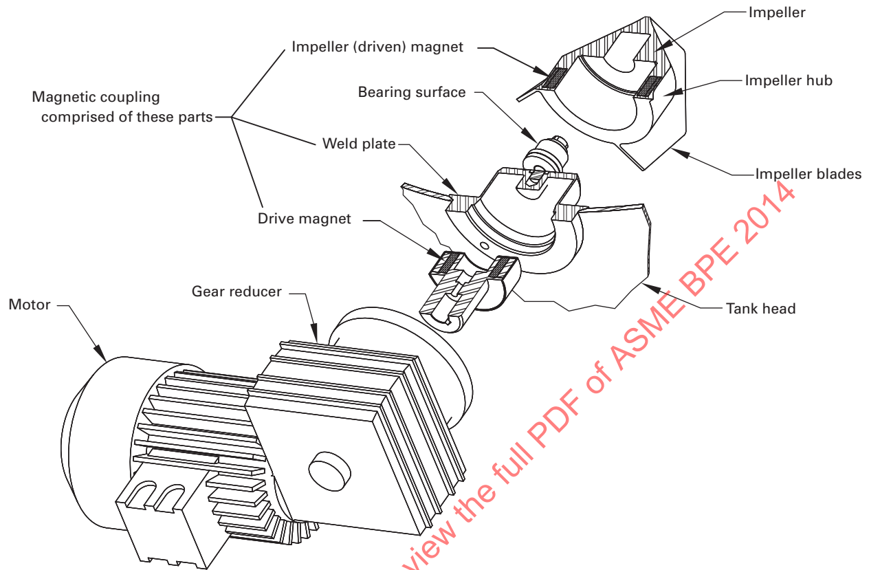
Fig. SD-3.5.5-2 Magnetically Coupled Mixer (Typical Bottom-Mount)
