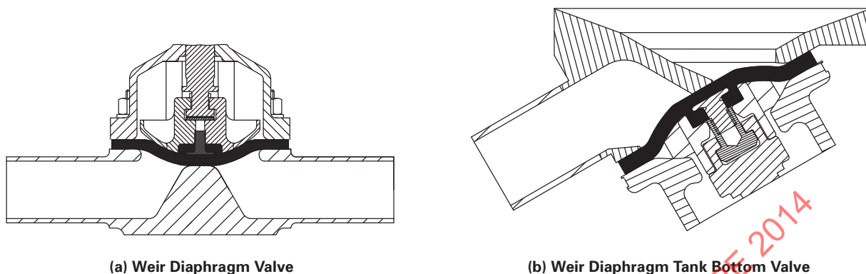
(a) Weir Diaphragm Valve
