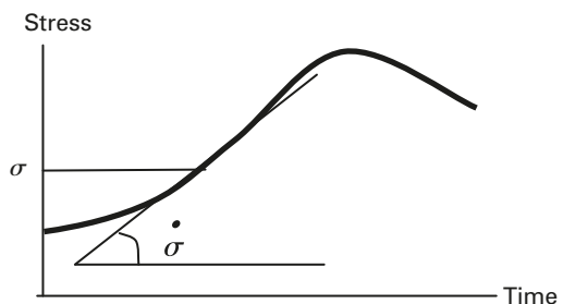
Figure 1 Stress History
