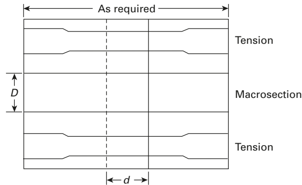
Figure 1 Bonding Specimen for Tension and Macrosection
