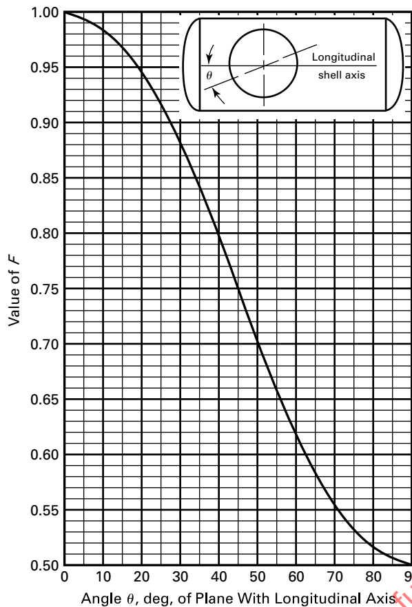
Figure PG-33.3 Chart for Determining Value of F
