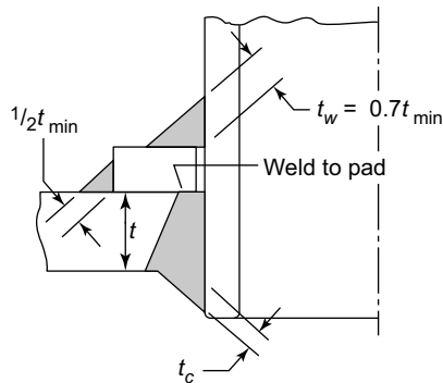
(h) Typical Flush-Type Nozzle
