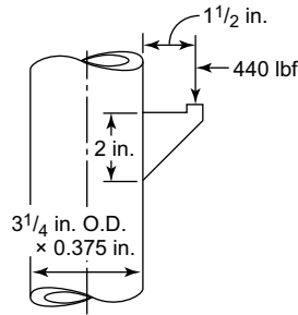
Figure A-73 Structural Attachment With Moment Load
