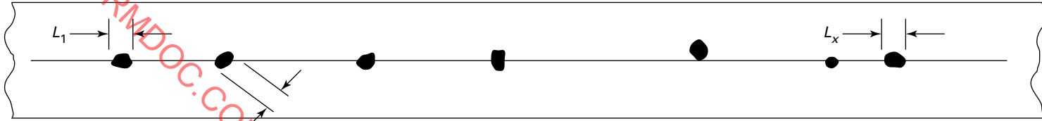
Figure A-250.3.4-1 Aligned Rounded Indications
