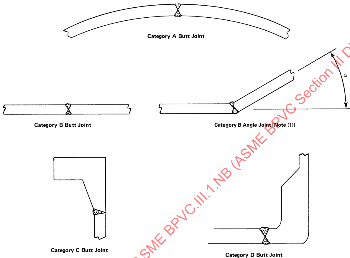
Figure NB-3352-1 Typical Butt Joints
