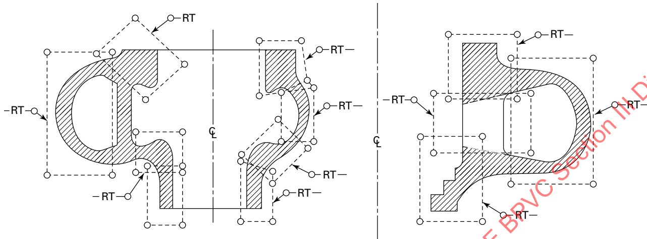
(a) Typical Volute-Type Pump Case
