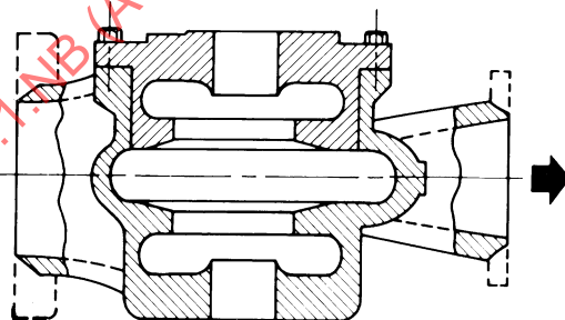
Figure NB-3441.2-1 Type B Pump
