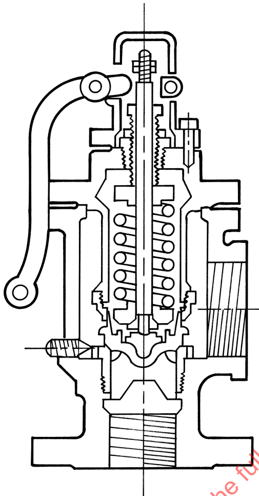
Figure 6.1.2-1 Safety Valve
