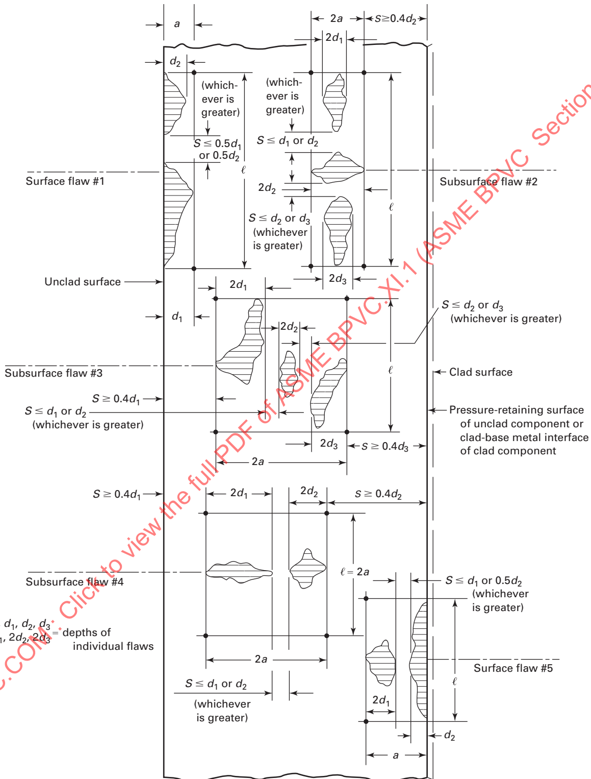
Figure IWA-3330-1 Multiple Planar Flaws Oriented in Plane Normal to Pressure-Retaining Surface
