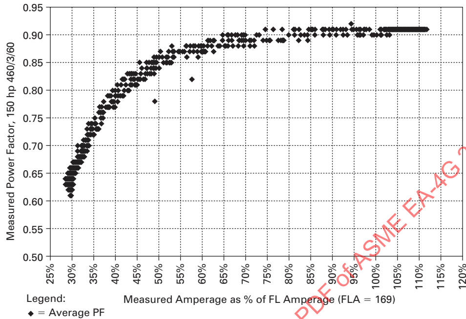
Fig. 3 Measured Power Factor Versus Percent Full-Load Amperage
