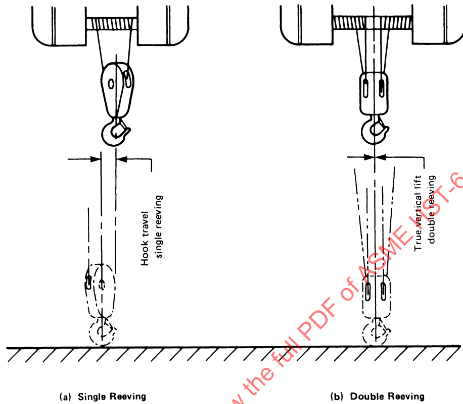
Figure 6-0.2-2 Single and Double Reeving
