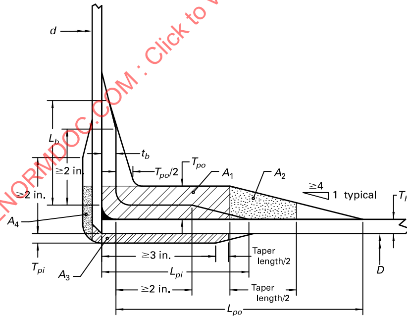
(b) Reinforcement on Inside and Outside [Note (2)]
