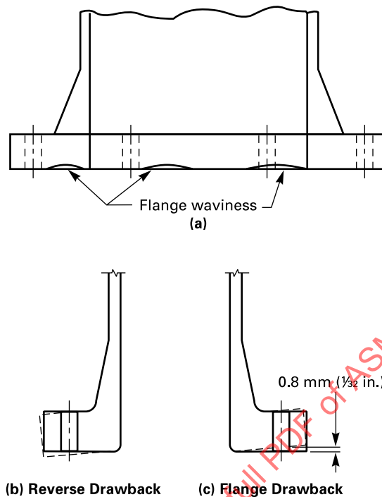
Figure 5-3.1.2.4-1 Flange Tolerances
