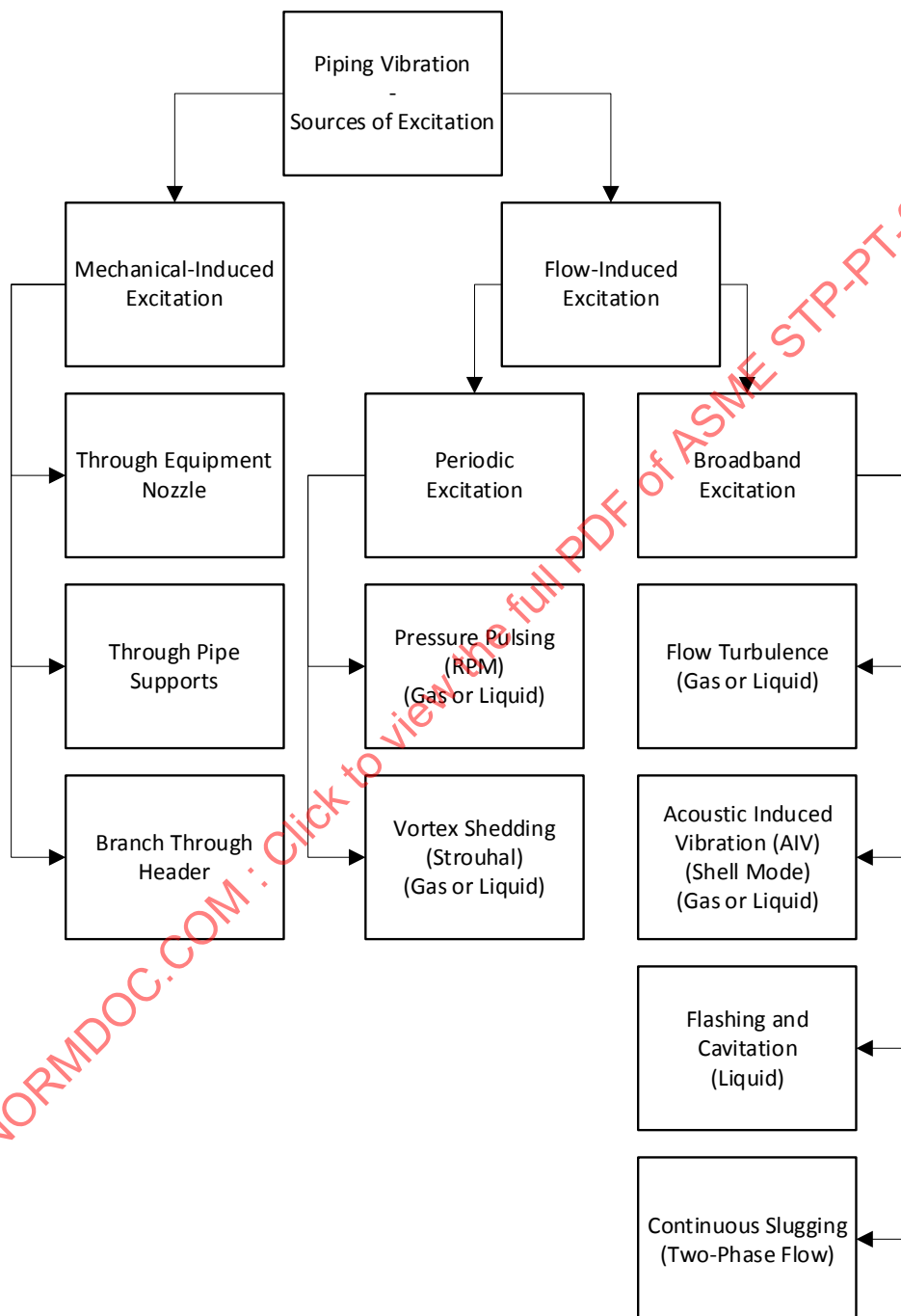
Figure 4-1: Sources of Piping Vibration
