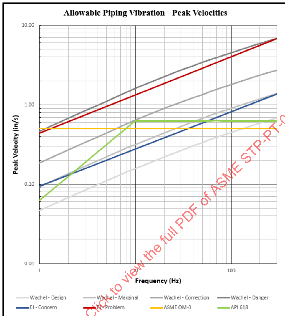
Figure 5-1: Current Vibration Velocity Amplitude Criteria, Superimposed, Color-Coded
