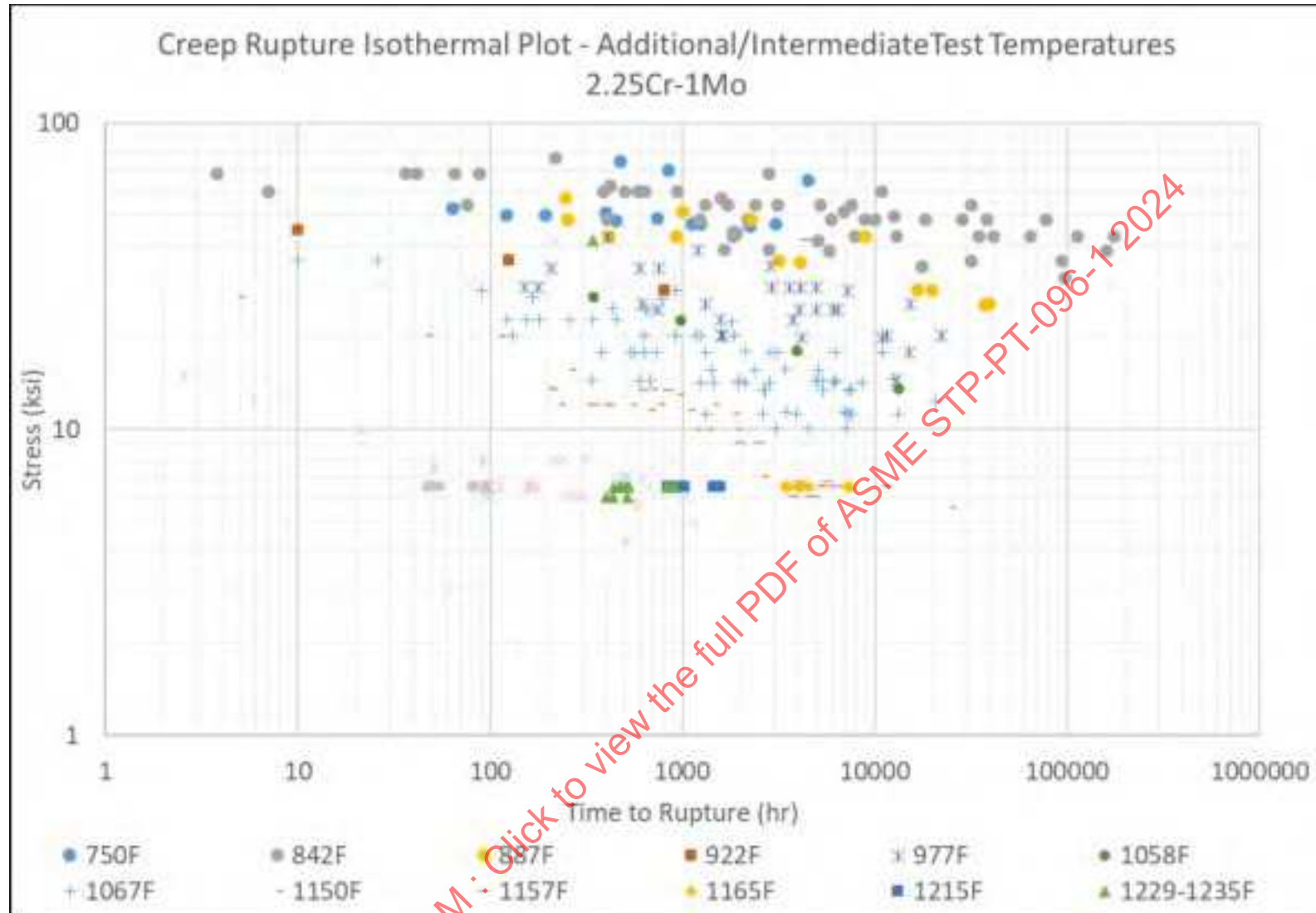
Figure 10-9: Grade 22 Creep Rupture Isotherm Curves for Additional and Intermediate Temperatures
