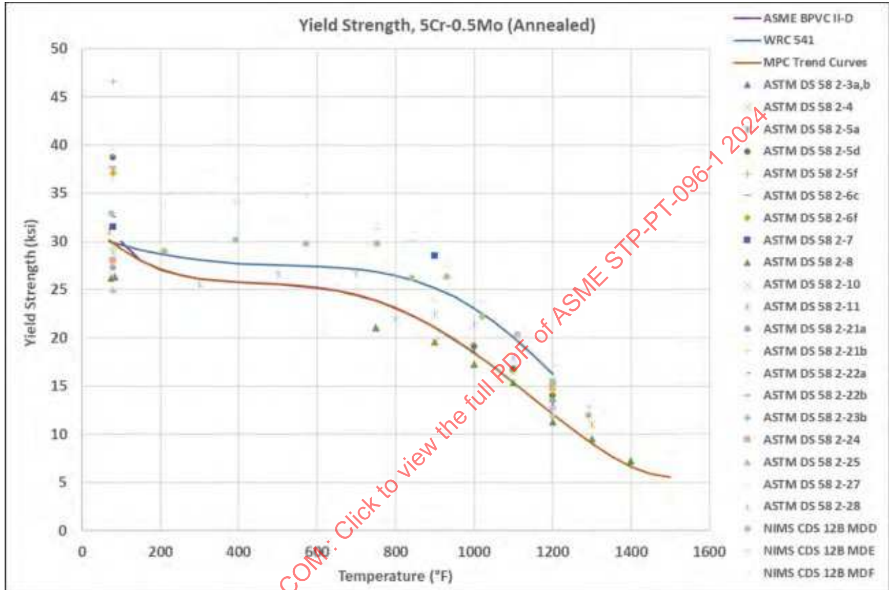
Figure 12-2: Grade 5 (Annealed) Yield Strength Vs. Temperature, By Data Source, Including Trend Curves
