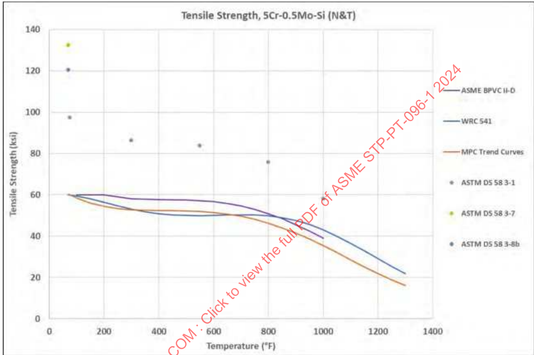
Figure 13-5: 5Cr-0.5Mo-Si (N&T) Tensile Strength Vs. Temperature, By Data Source, Including Trend Curves
