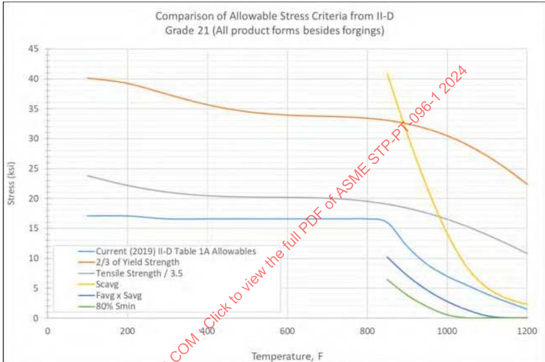
Figure 24-14: Comparison of Current 316H Allowable Stresses (Except Forgings) Vs. ASME II-D Appendix 1 Criteria Applied to Data
