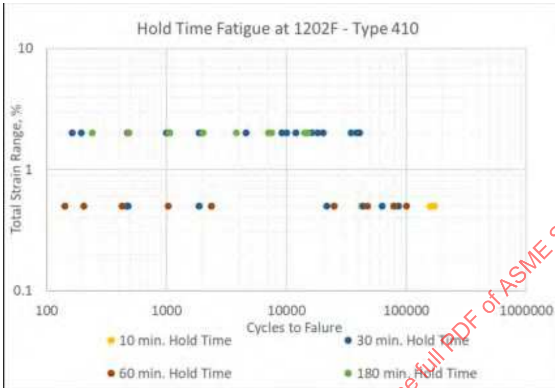
Figure 25-24: Type 410/12Cr Hold Time Data (Creep Fatigue) for Type 410/12Cr, Temperature of 1202°F
