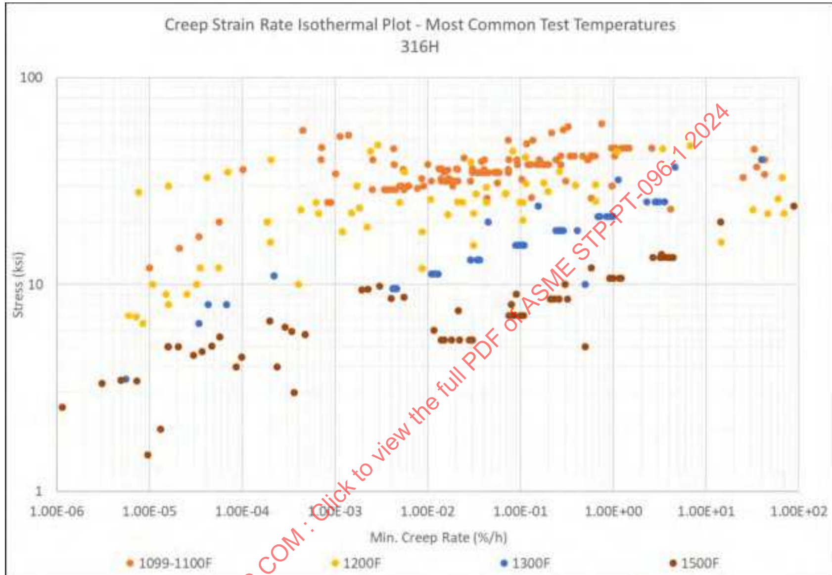
Figure 17-10: 316H Creep Strain Rate (MCR) Isotherm Curves, Temperatures With High Concentration of Data Points
