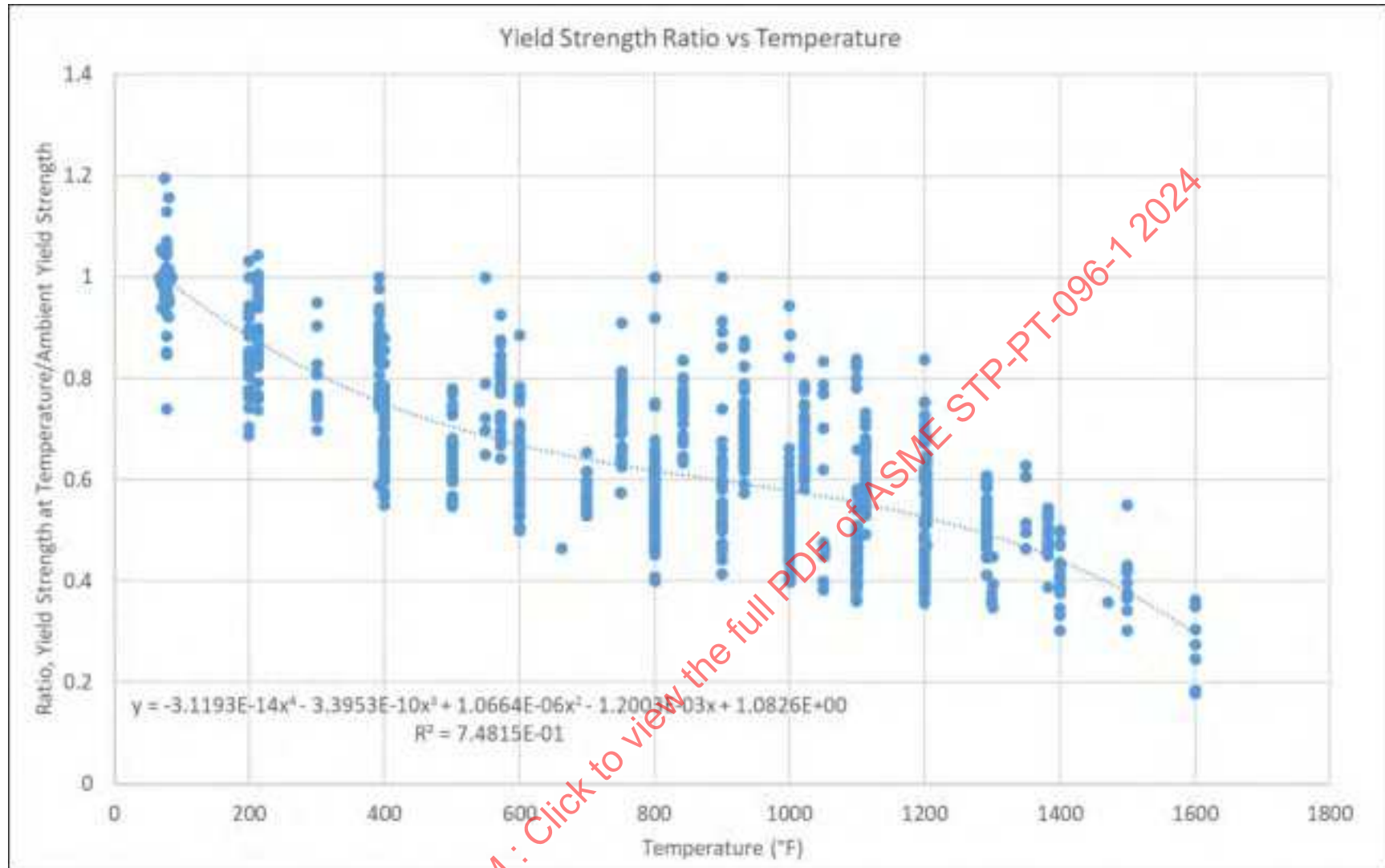
Figure 16-6: 304H Yield Strength Ratios Vs. Temperature, All Combined Data, With Polynomial Regression
