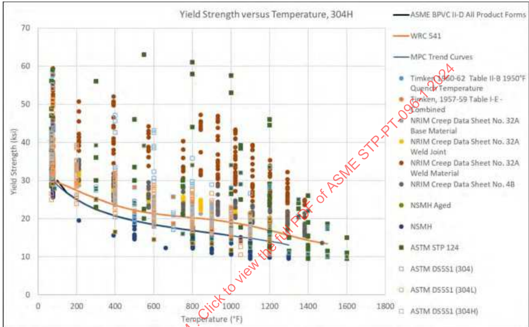
Figure 16-2: 304H Yield Strength Vs. Temperature, By Data Source, Including Trend Curves
