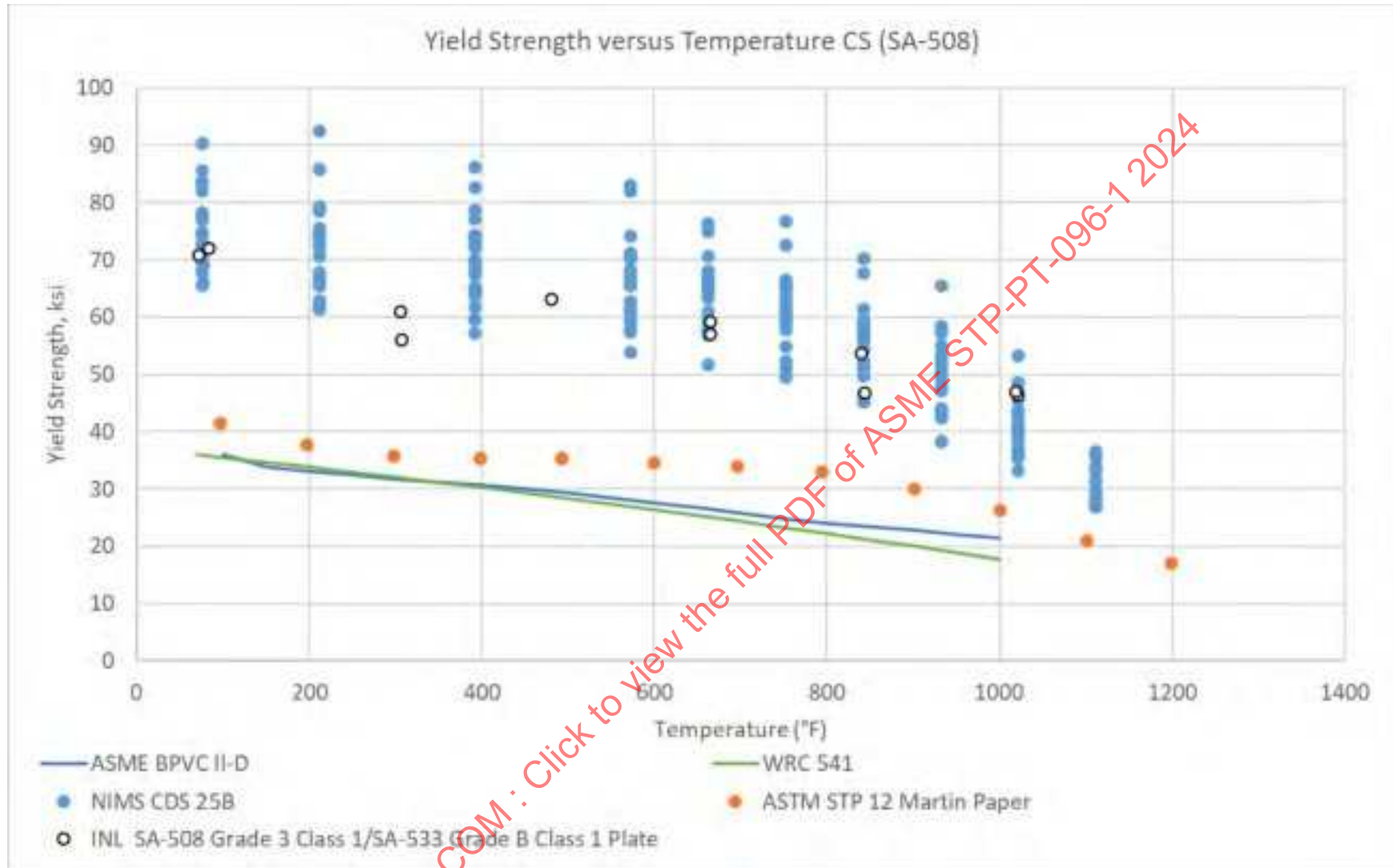
Figure 6-2: CS (SA-508) Yield Strength Vs. Temperature, By Data Source, Including Trend Curves
