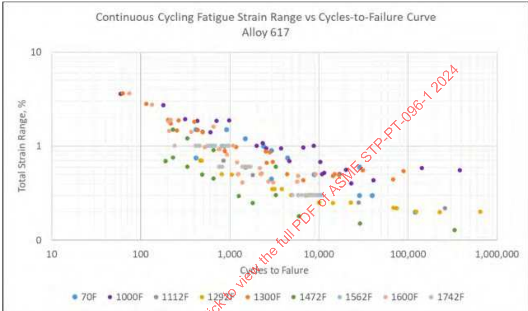
Figure 19-17: Alloy 617 Continuous Cycling Fatigue, Including Room Temperature and Elevated Temperature Data
