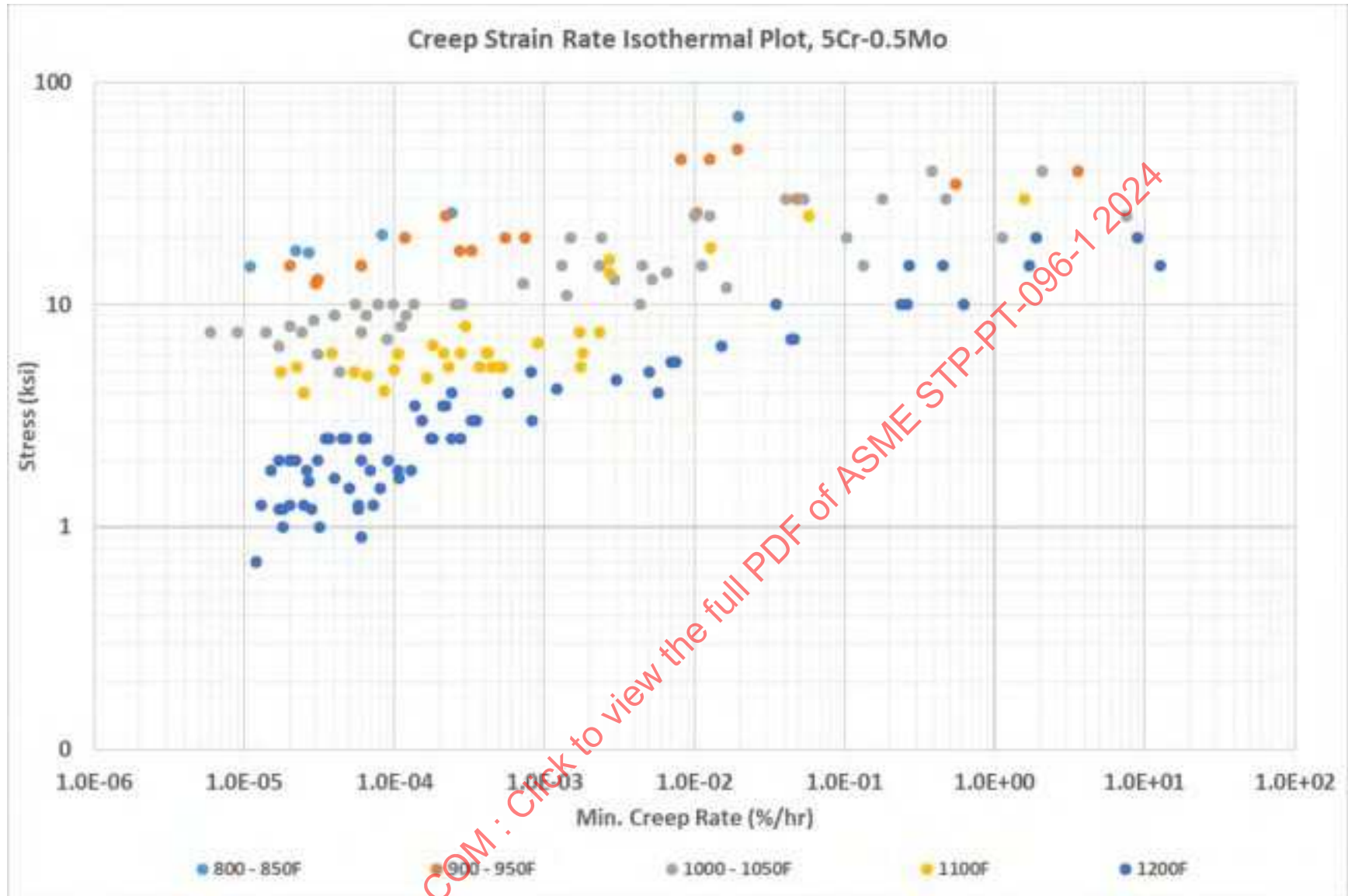
Figure 12-15: Grade 5 Creep Strain Rate (MCR) Isotherm Curves
