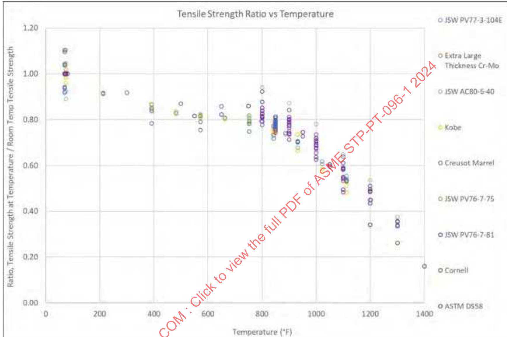
Figure 24-5: 3Cr Tensile Strength Ratios Vs. Temperature (Calculated on a Heat-By-Heat Basis, By Data Source)
