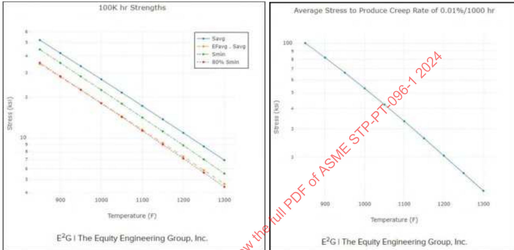
Figure 21-13: Calculated Allowable Stresses Based on Rupture and Creep Strain Rate and ASME II-D Appendix 1 Criteria (Alloy 800H)
