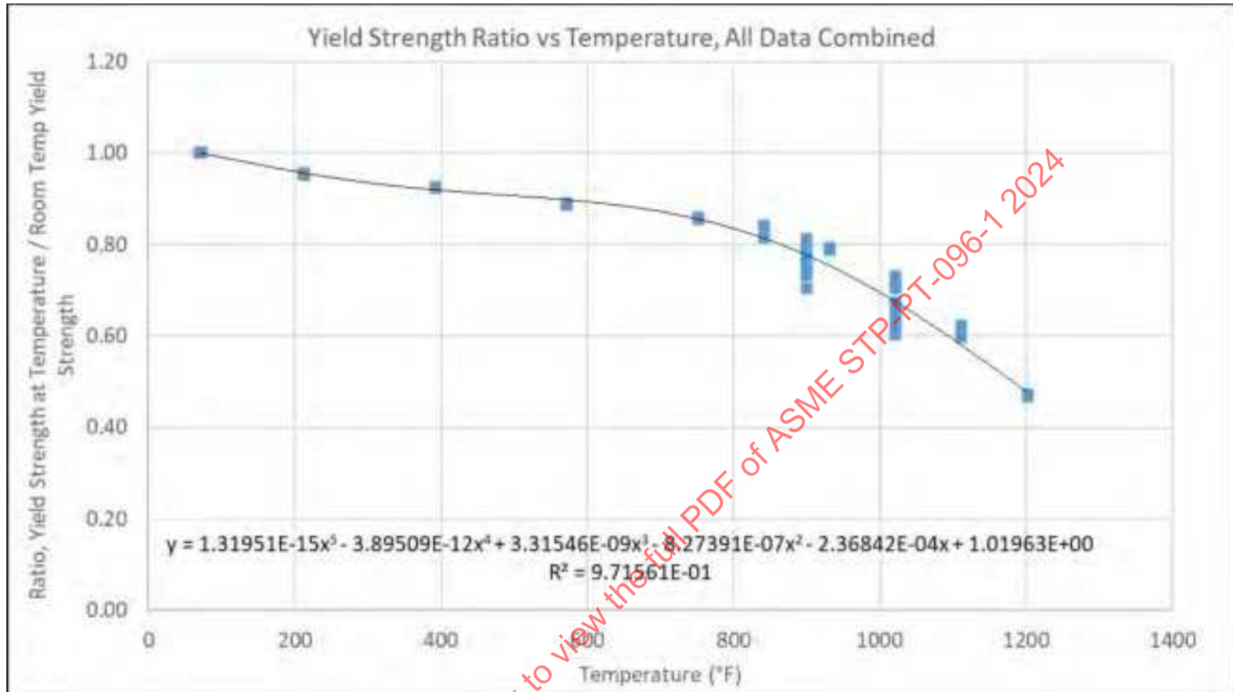
Figure 11-6: Grade 22V Yield Strength Ratios Vs. Temperature, All Combined Data, With Polynomial Regression
