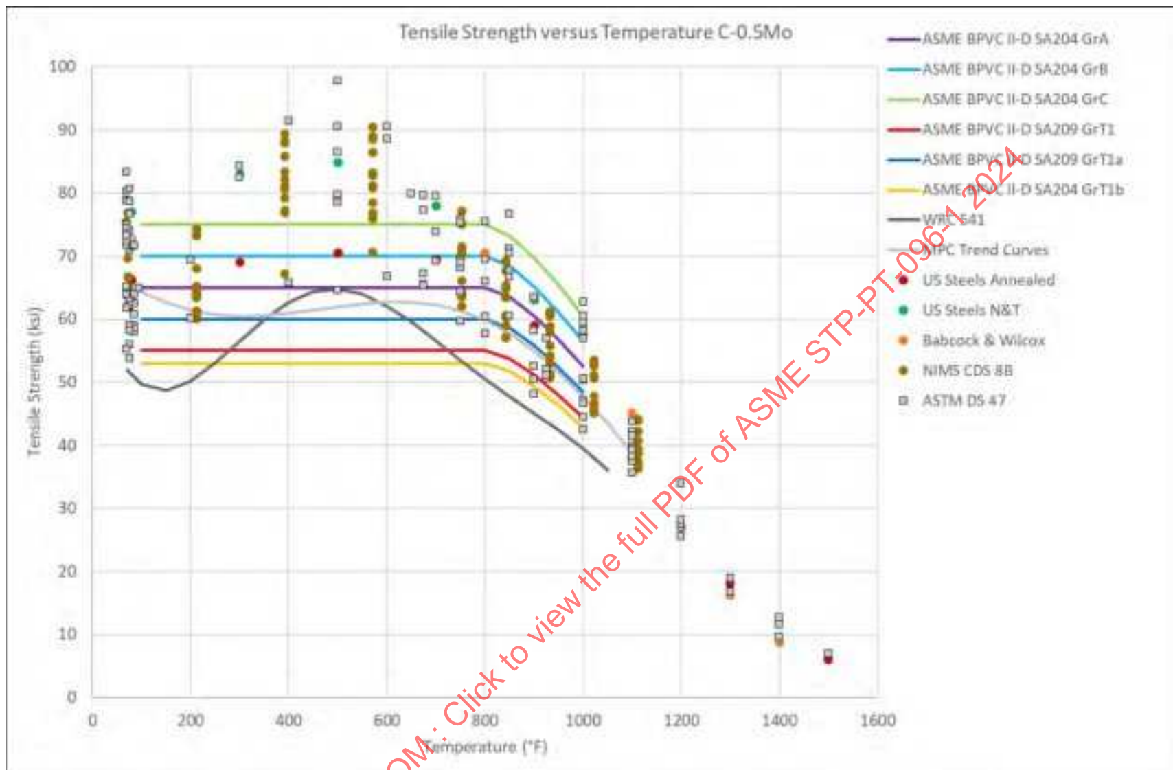
Figure 8-3: C-1/2Mo Tensile Strength Vs. Temperature, By Data Source, Including Trend Curves
