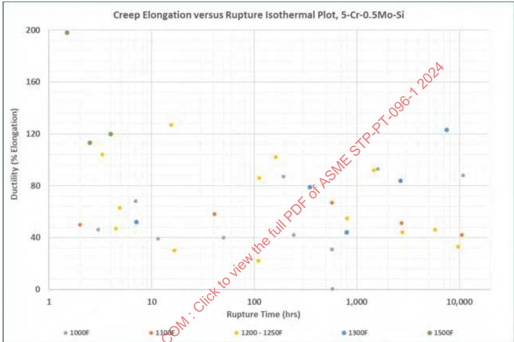
Figure 13-16: 5Cr-0.5Mo-Si Creep Ductility (% Elongation) Vs. Rupture Time Isotherms
