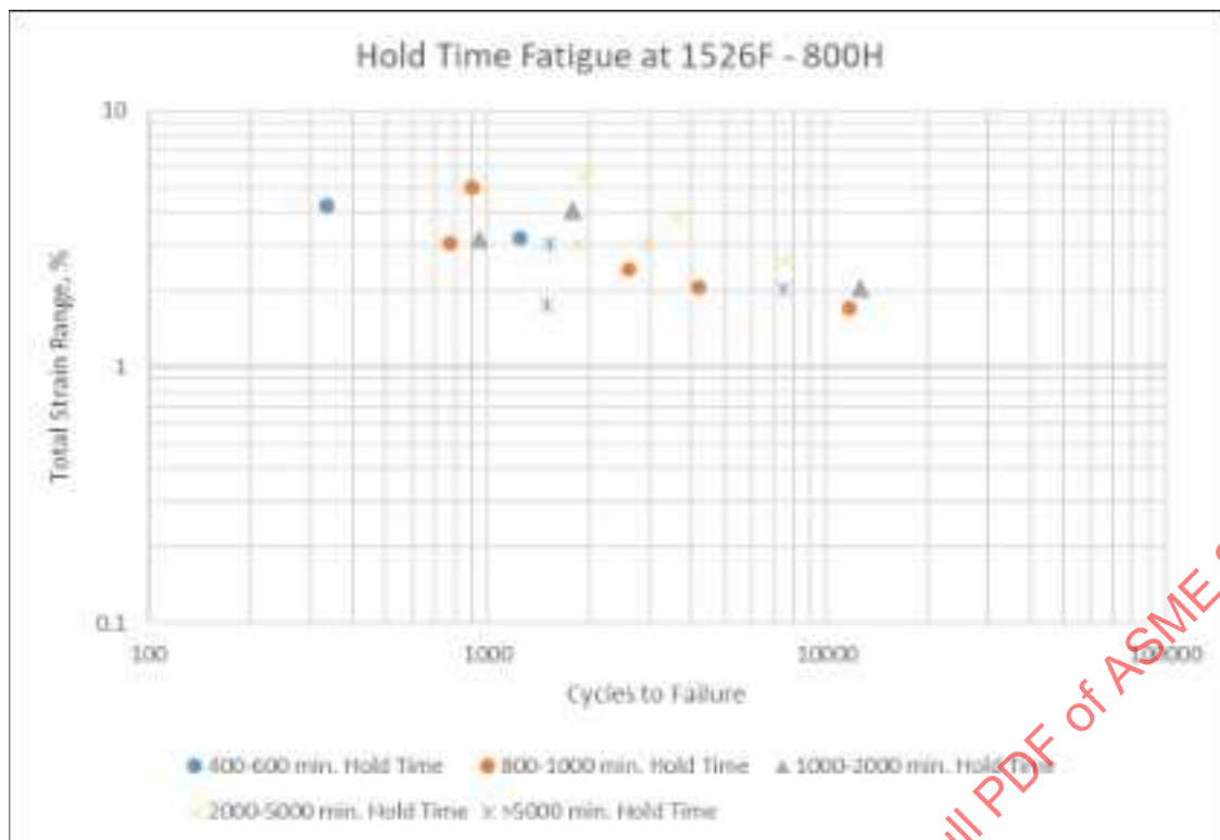
Figure 21-25: Alloy 800H Hold Time Data (Creep Fatigue) for Alloy 800H, Temperature of 1526°F
