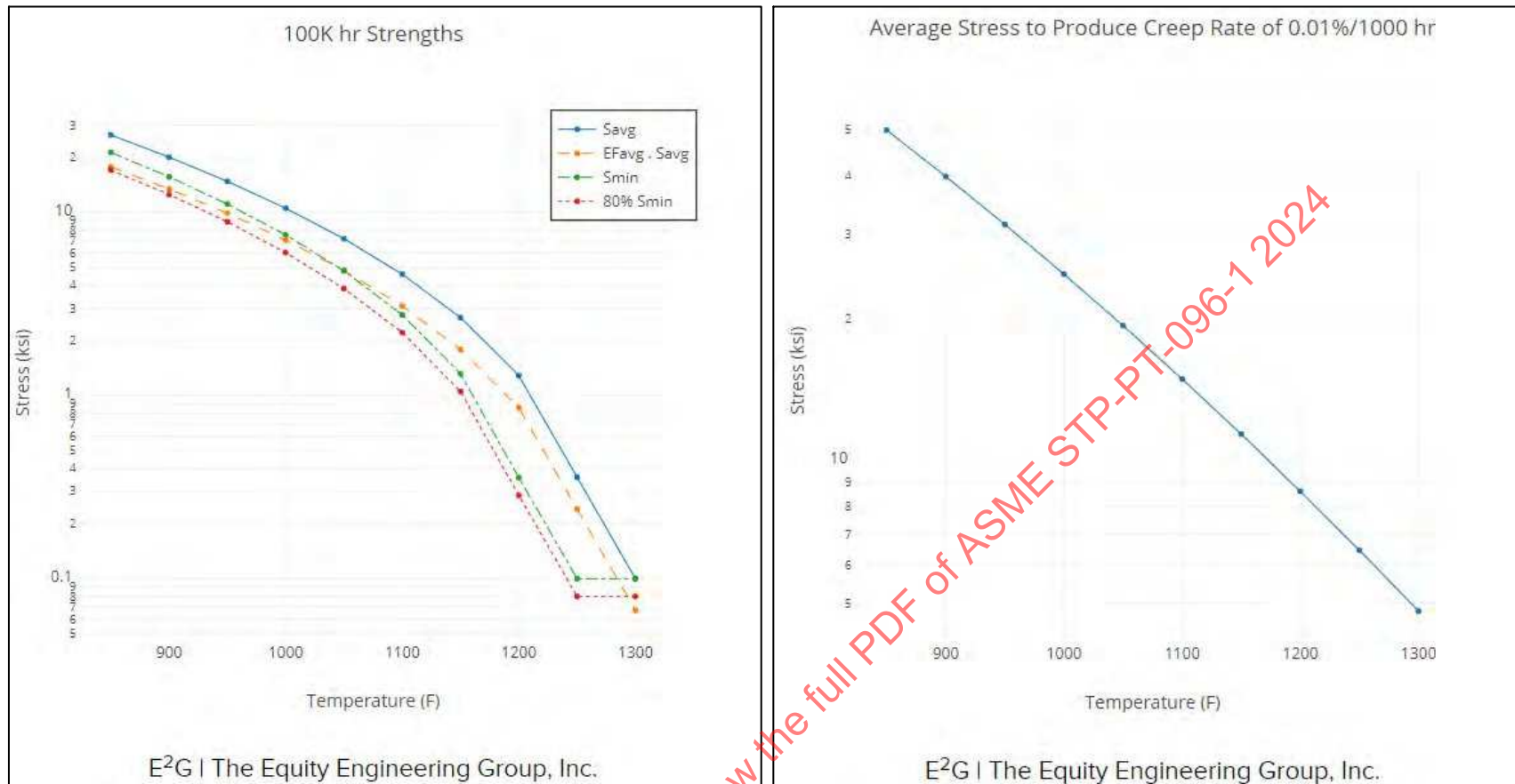
Figure 10-13: Calculated Allowable Stresses Based On Rupture and Creep Strain Rate and ASME II-D Appendix 1 Criteria (Grade 22)
