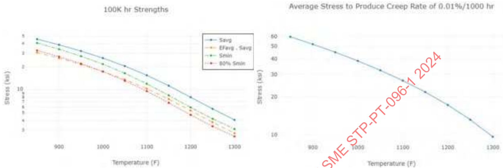
Figure 26-13: Calculated Allowable Stresses Based on Rupture and Creep Strain Rate and ASME II-D Appendix 1 Criteria (321H)
