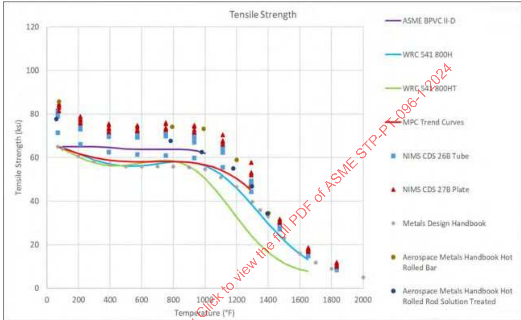
Figure 21-3: Alloy 800H Tensile Strength Vs. Temperature, By Data Source, Including Trend Curves
