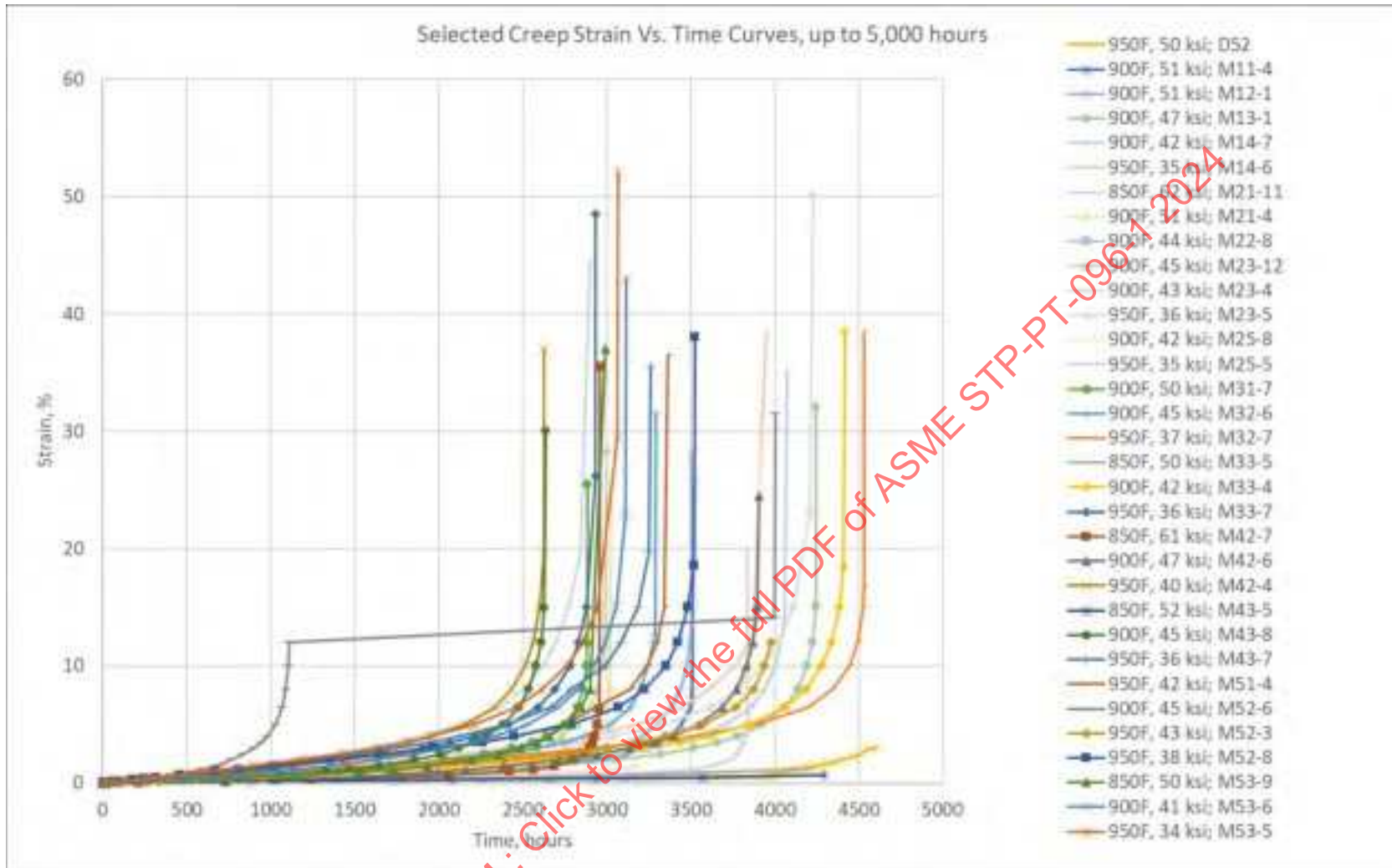
Figure 11-18: Long-Term Strain Vs. Time Data, up to 5,000 Hour Test Durations (Grade 22V)
