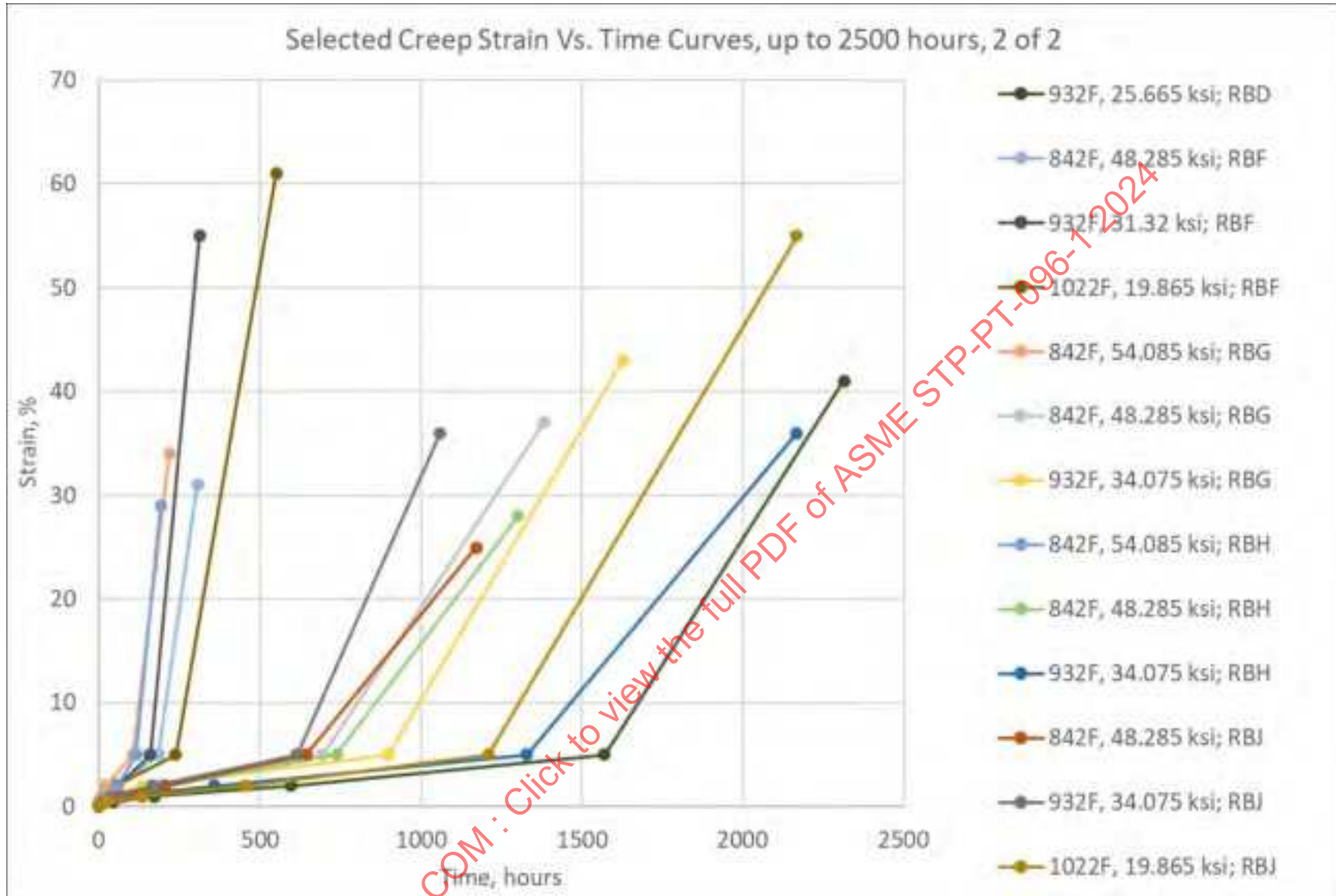
Figure 25-16: Short-Term Strain Vs. Time Data, up to 2,500 Hour Test Durations (Type 410/12Cr), 2 of 2
