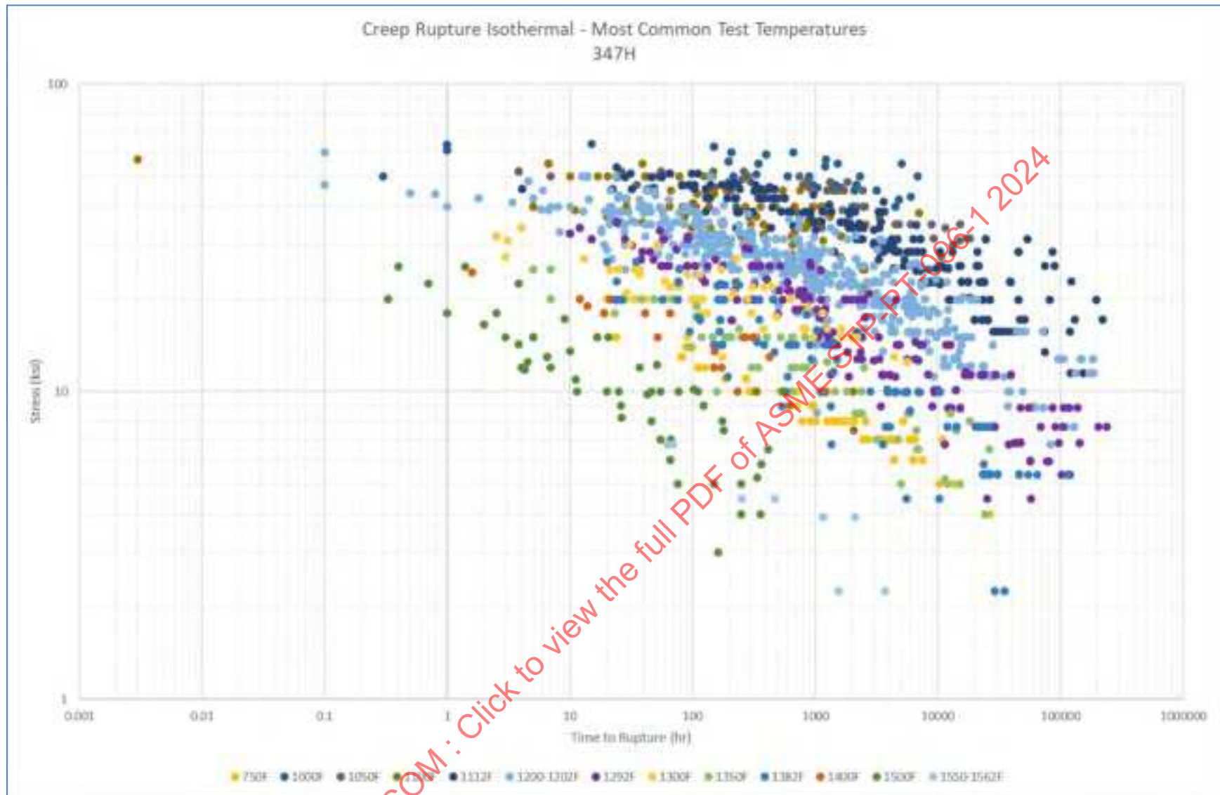
Figure 18-8: 347H Creep Rupture Isotherm Curves, Temperatures With High Concentration of Data Points
