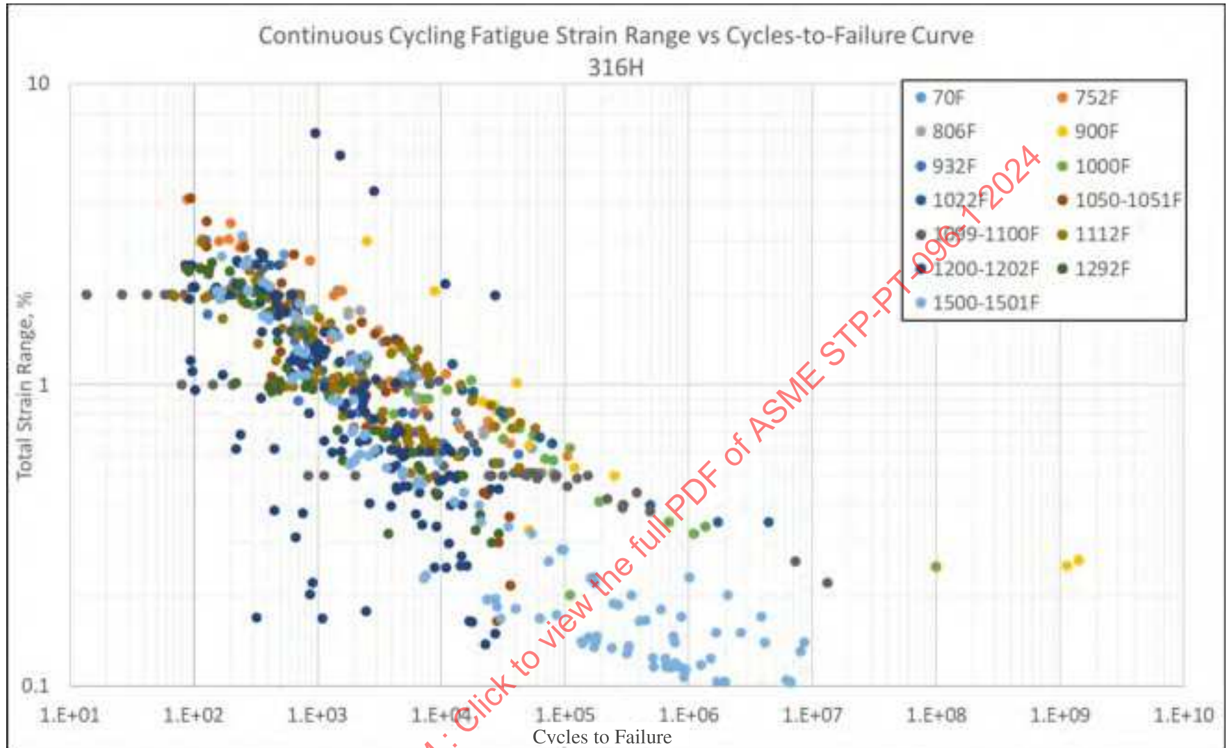
Figure 17-18: Continuous Cycling Fatigue (316H), Including Room Temperature and Elevated Temperature Data
