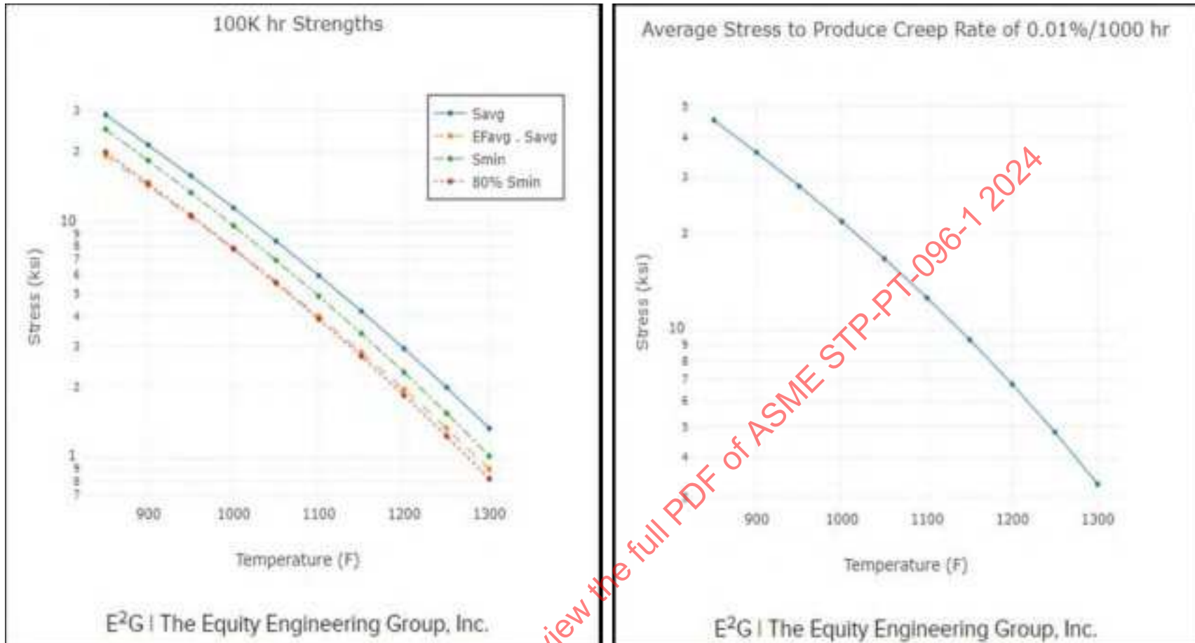
Figure 14-13: Calculated Allowable Stresses Based on Rupture and Creep Strain Rate and ASME II-D Appendix 1 Criteria (Grade 9)
