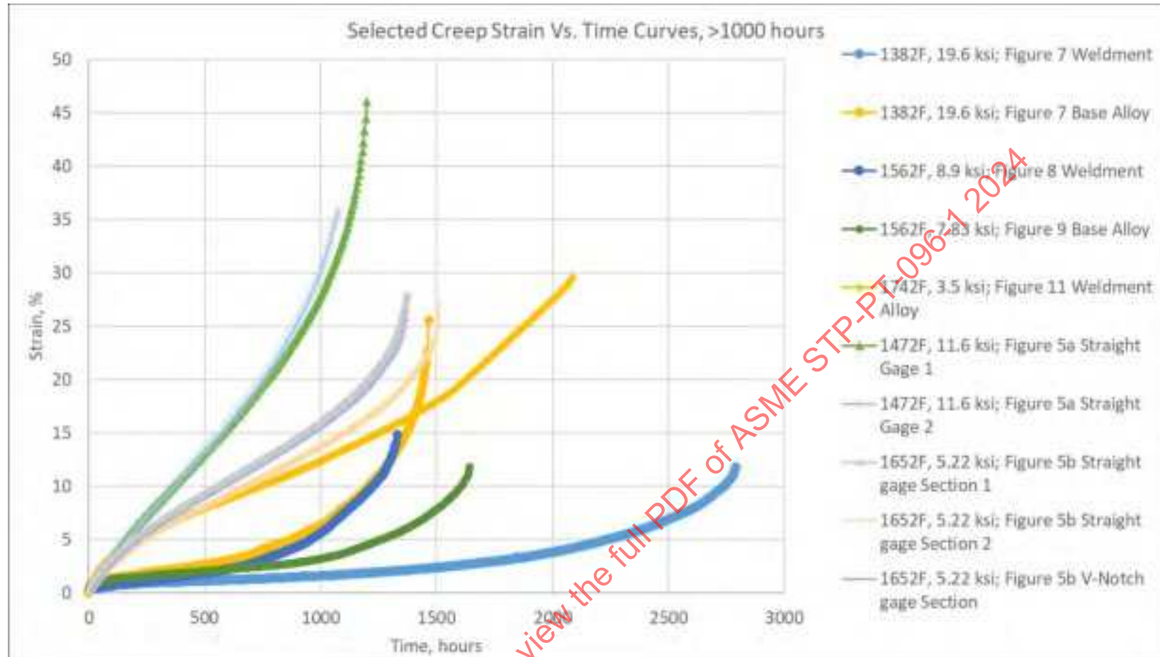
Figure 19-16: Short-Term Strain Vs. Time Data, In Excess of 1,000 Hour Test Durations (Alloy 617)
