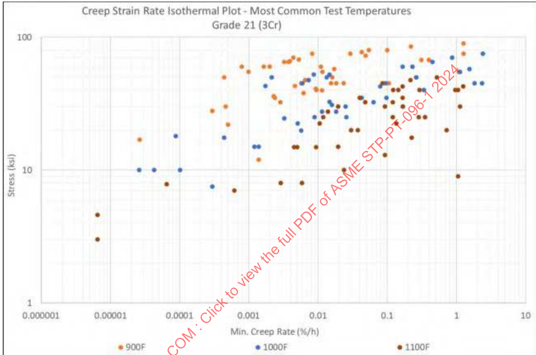
Figure 24-10: 3Cr Creep Strain Rate (MCR) Isotherm Curves, Temperatures With High Concentration of Data Points
