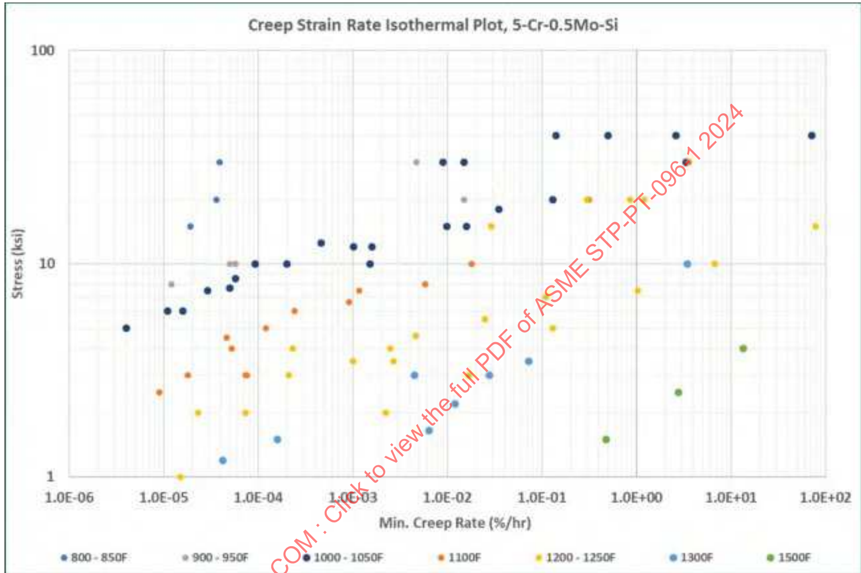
Figure 13-15: 5Cr-0.5Mo-Si Creep Strain Rate (MCR) Isotherm Curves
