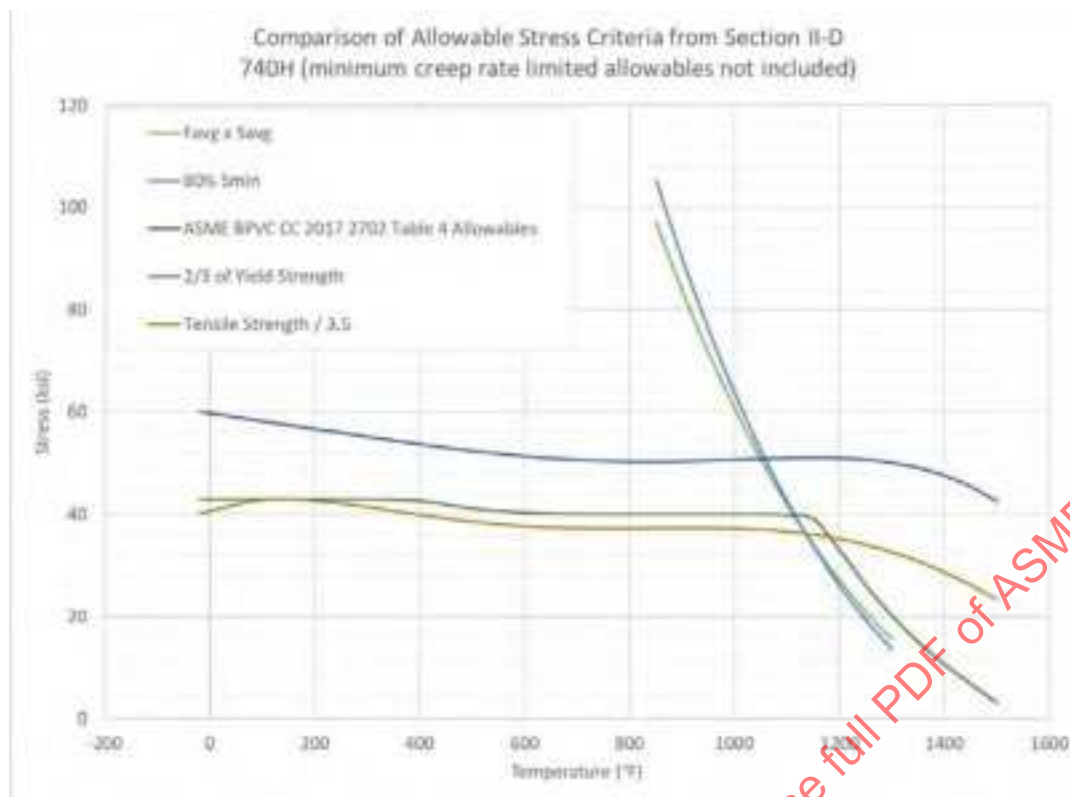
Figure 20-12: Comparison of Current 740H Allowable Stresses Vs. ASME II-D Appendix 1 Criteria Applied to Data
