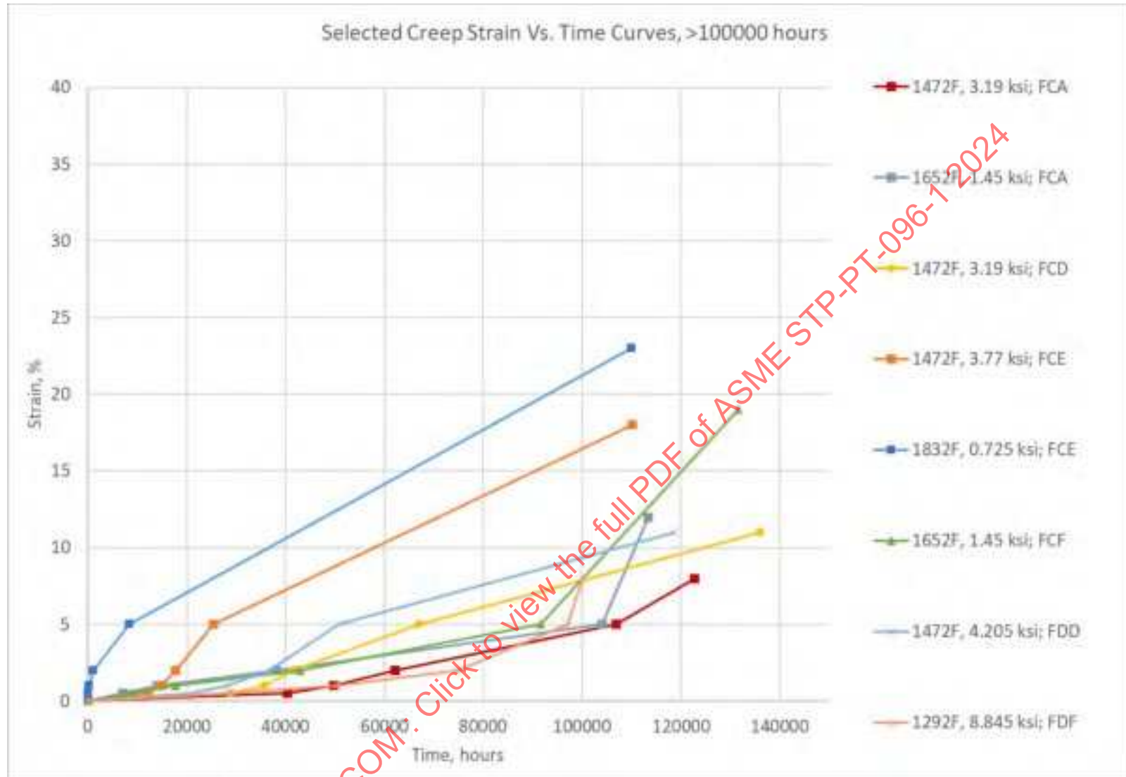
Figure 21-20: Long-Term Strain Vs. Time Data, 10,000 to 100,000 Hour Test Durations (Alloy 800H)
