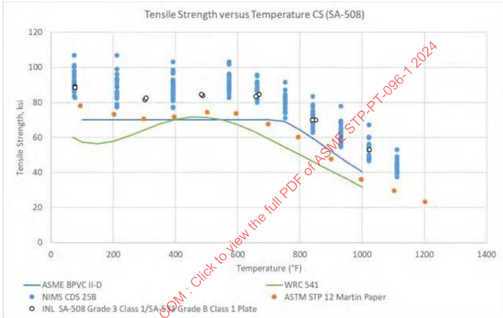
Figure 6-3: CS (SA-508) Tensile Strength Vs. Temperature, By Data Source, Including Trend Curves
