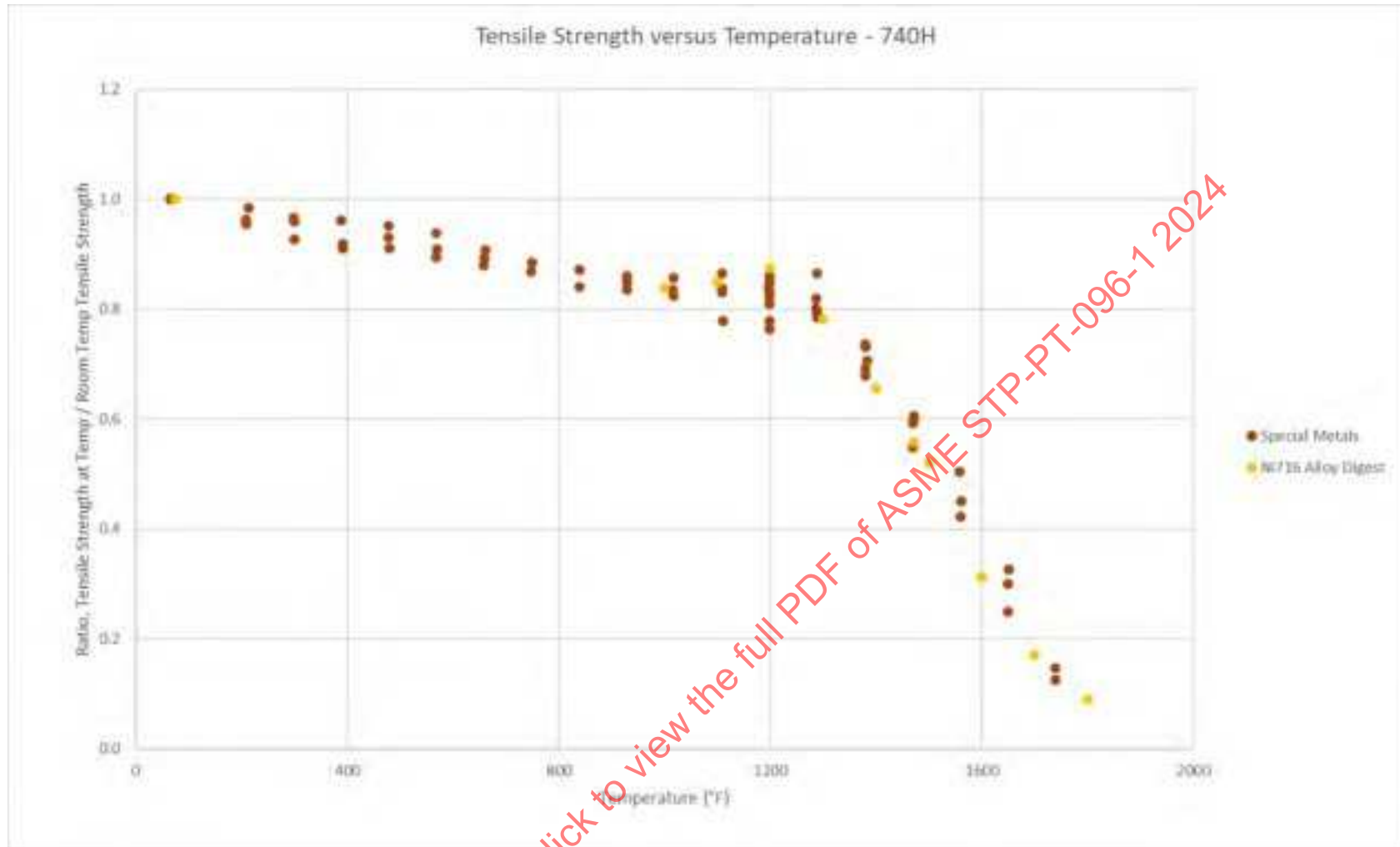
Figure 20-5: 740H Tensile Strength Ratios Vs. Temperature (Calculated on a Heat-By-Heat Basis, By Data Source)
