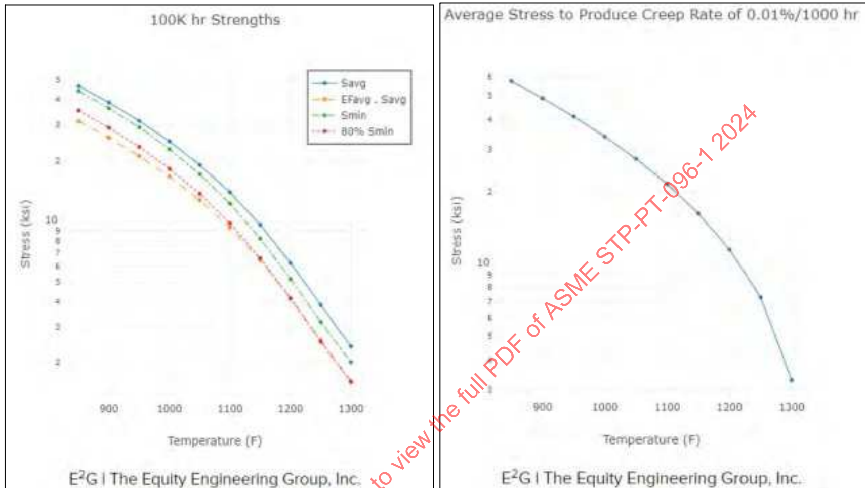
Figure 4-13: Calculated Allowable Stresses Based on Rupture and Creep Strain Rate and ASME II-D Appendix 1 Criteria (Grade 91)
