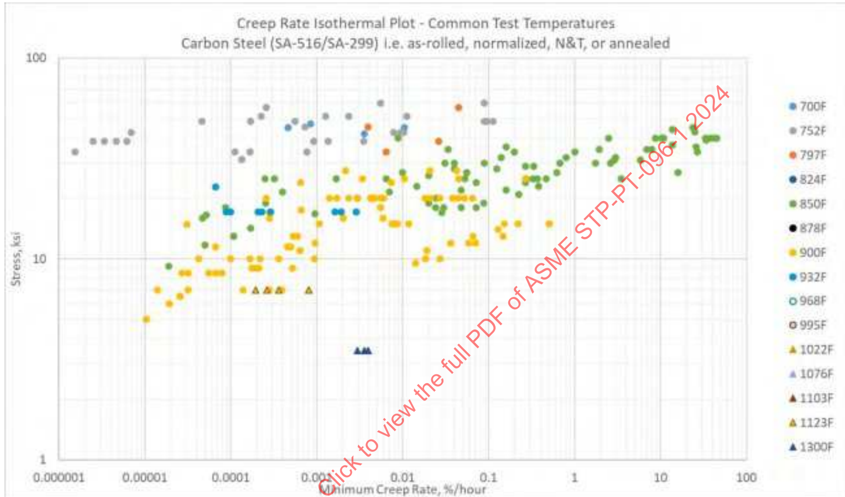
Figure 5-10: CS (516/299) Creep Strain Rate (MCR) Isotherm Curves, 1 of 3
