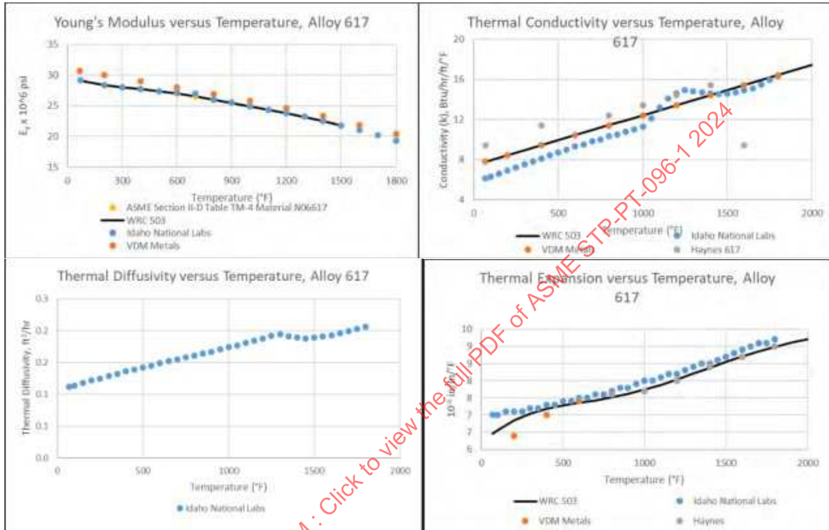
Figure 19-1: Alloy 617 Modulus ( E_y ), Thermal Conductivity ( k ), Thermal Diffusivity (TD), & Thermal Expansion ( \alpha ) With Temperature
