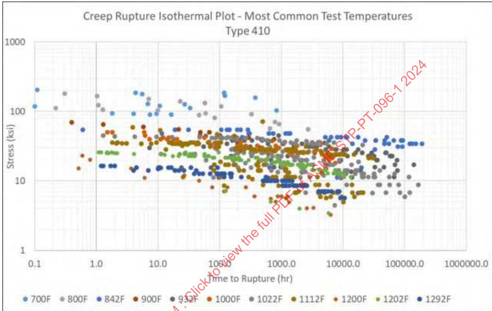
Figure 25-8: Type 410/12Cr Creep Rupture Isotherm Curves, Temperatures With High Concentration of Data Points
