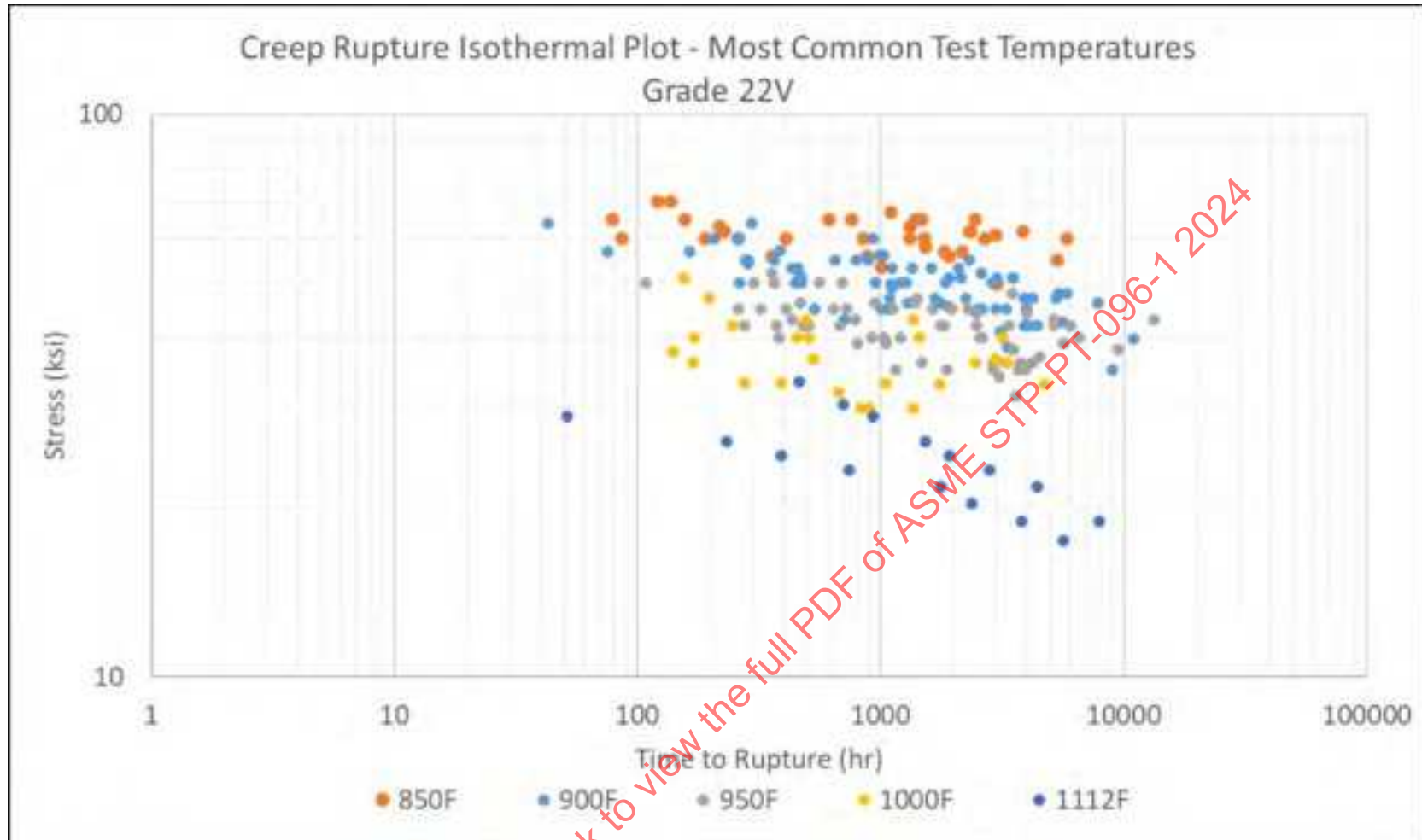
Figure 11-8: Grade 22V Creep Rupture Isotherm Curves, Temperatures With High Concentration of Data Points
