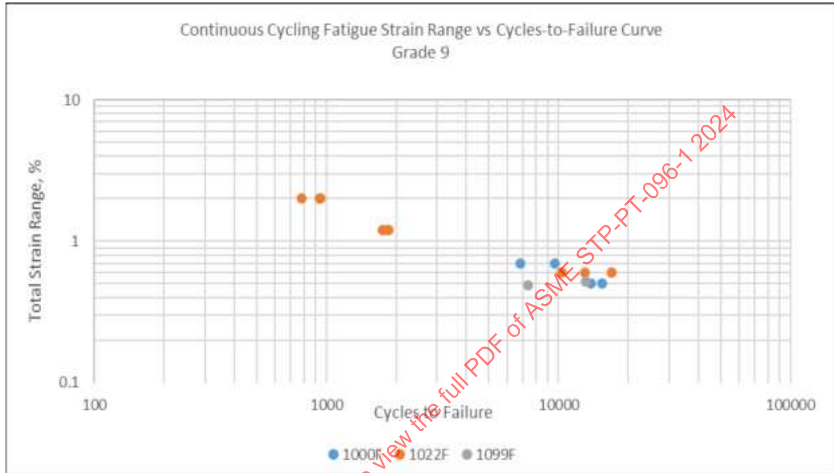
Figure 14-19: Grade 9 Continuous Cycling Fatigue Data, Including Elevated Temperature Data
