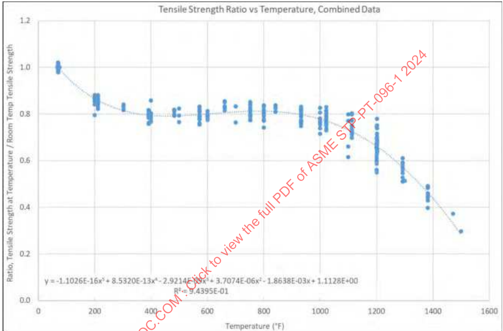
Figure 26-7: 321H Tensile Strength Ratios Vs. Temperature, All Combined Data, With Polynomial Regression
