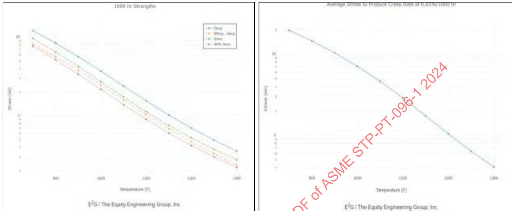
Figure 5-14: Calculated Allowable Stresses Based on Rupture and Creep Strain Rate and ASME II-D Appendix 1 Criteria (CS (516/299))
