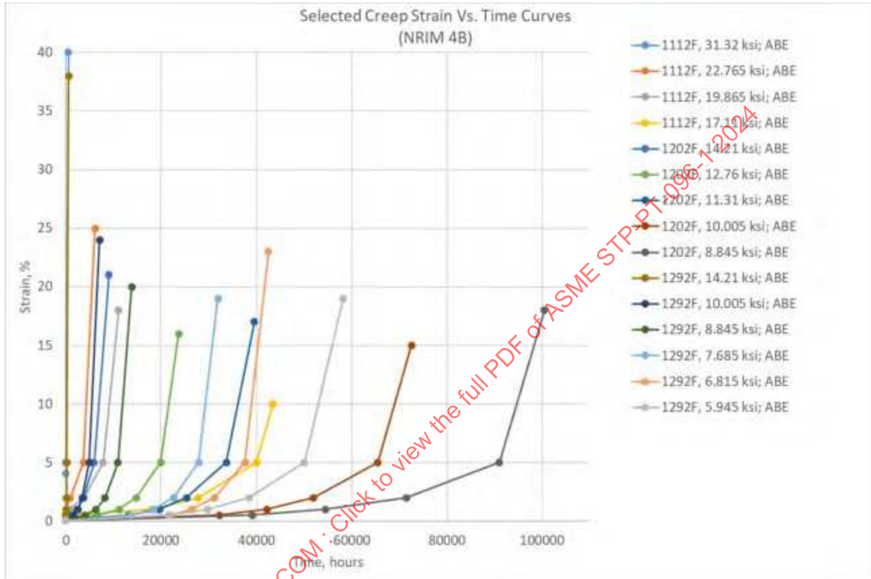
Figure 16-14: Strain Vs. Time Data at Multiple Temperatures From NRIM 4B (304H)
