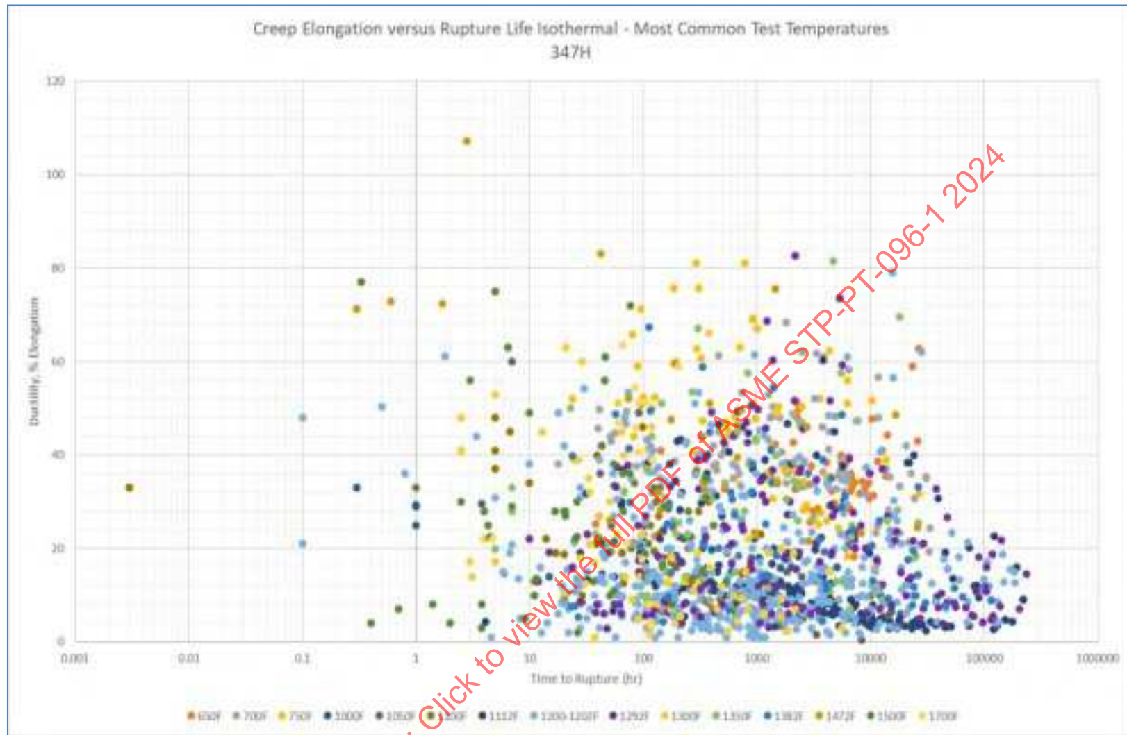
Figure 18-11: 347H Creep Ductility (% Elongation) Vs. Rupture Time Isotherms, Most Common Test Temperatures
