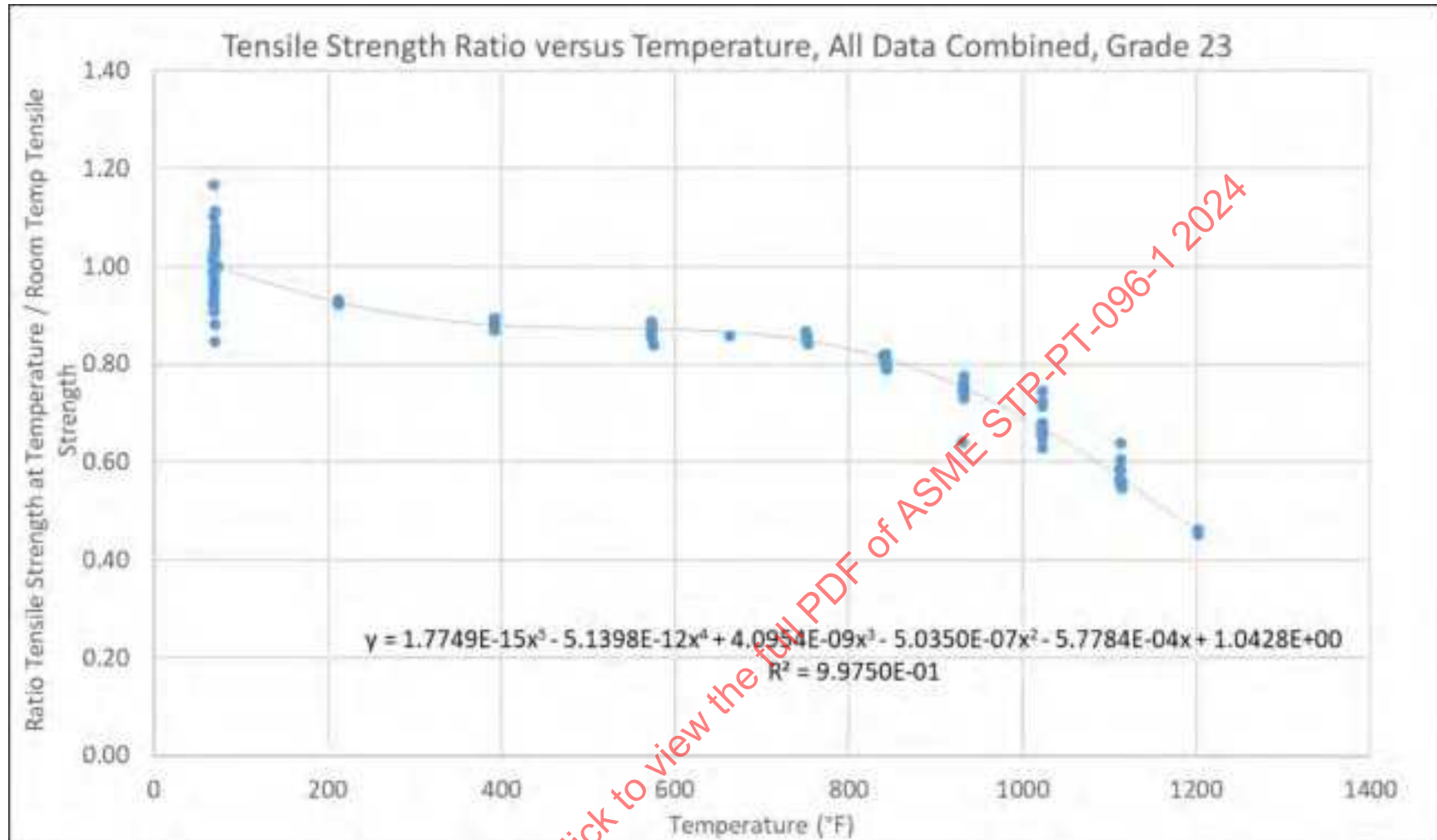
Figure 23-7: Grade 23 Tensile Strength Ratios Vs. Temperature, All Combined Data, With Polynomial Regression
