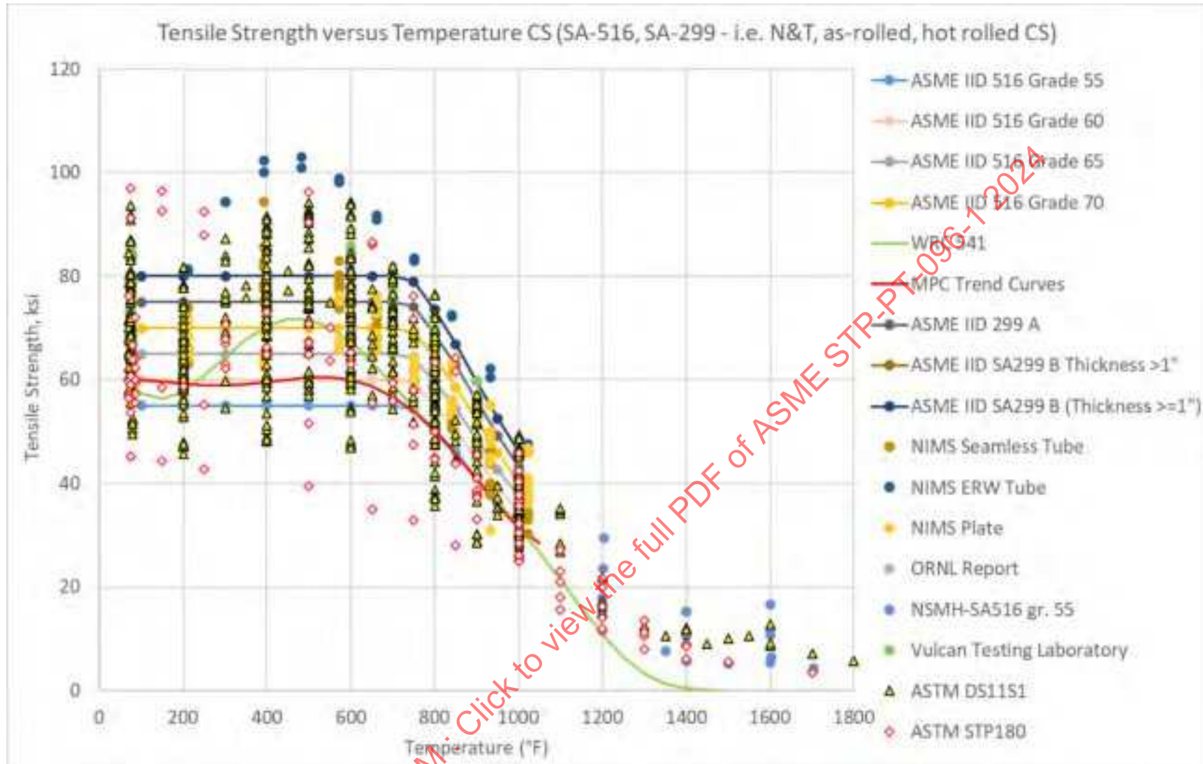
Figure 5-3: CS (516/299) Tensile Strength Vs. Temperature, By Data Source, Including Trend Curves
