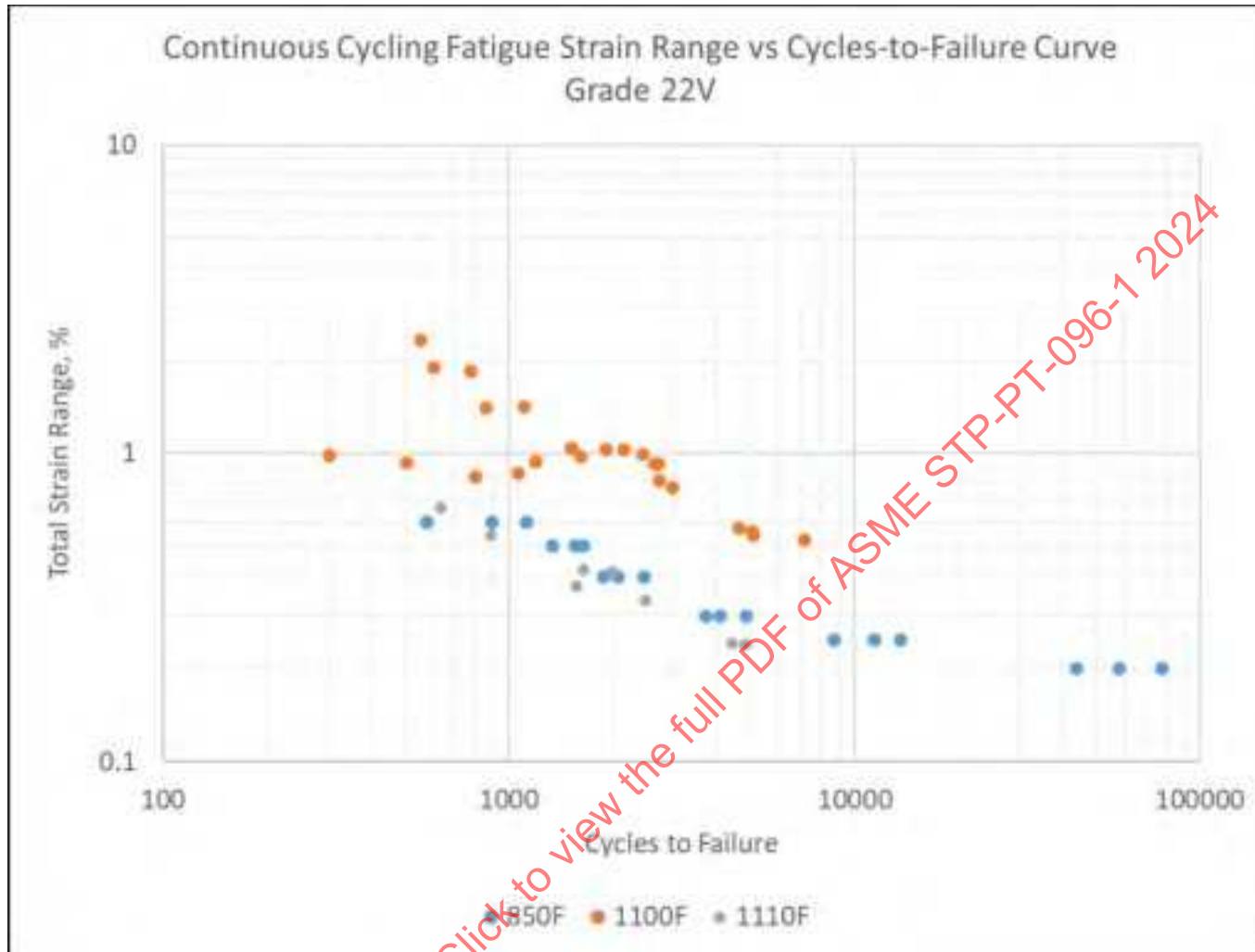
Figure 11-21: Grade 22V Continuous Cycling Fatigue (Grade 22V), Including Elevated Temperature Data
