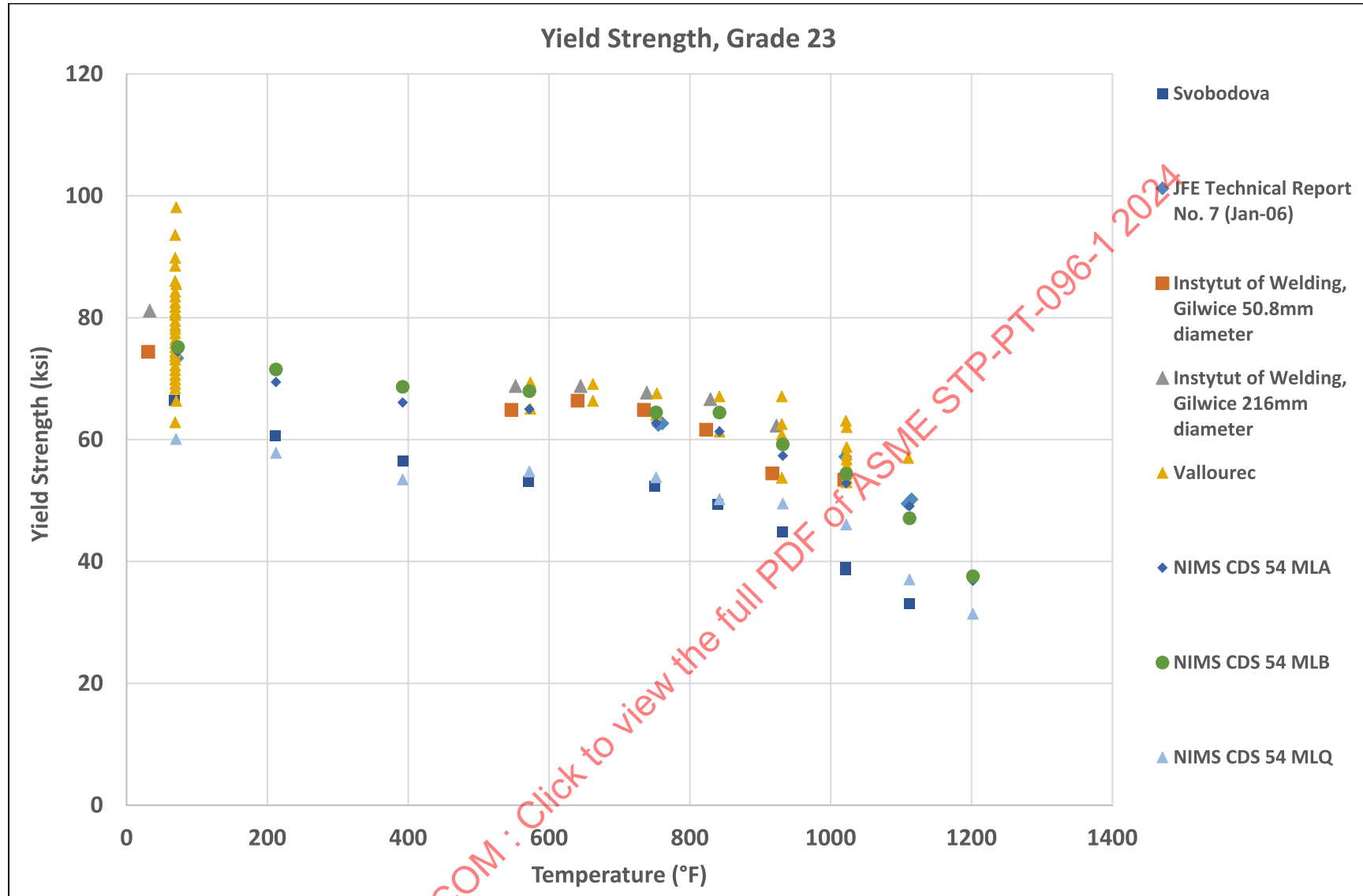
Figure 23-2: Grade 23 Yield Strength Vs. Temperature, By Data Source
