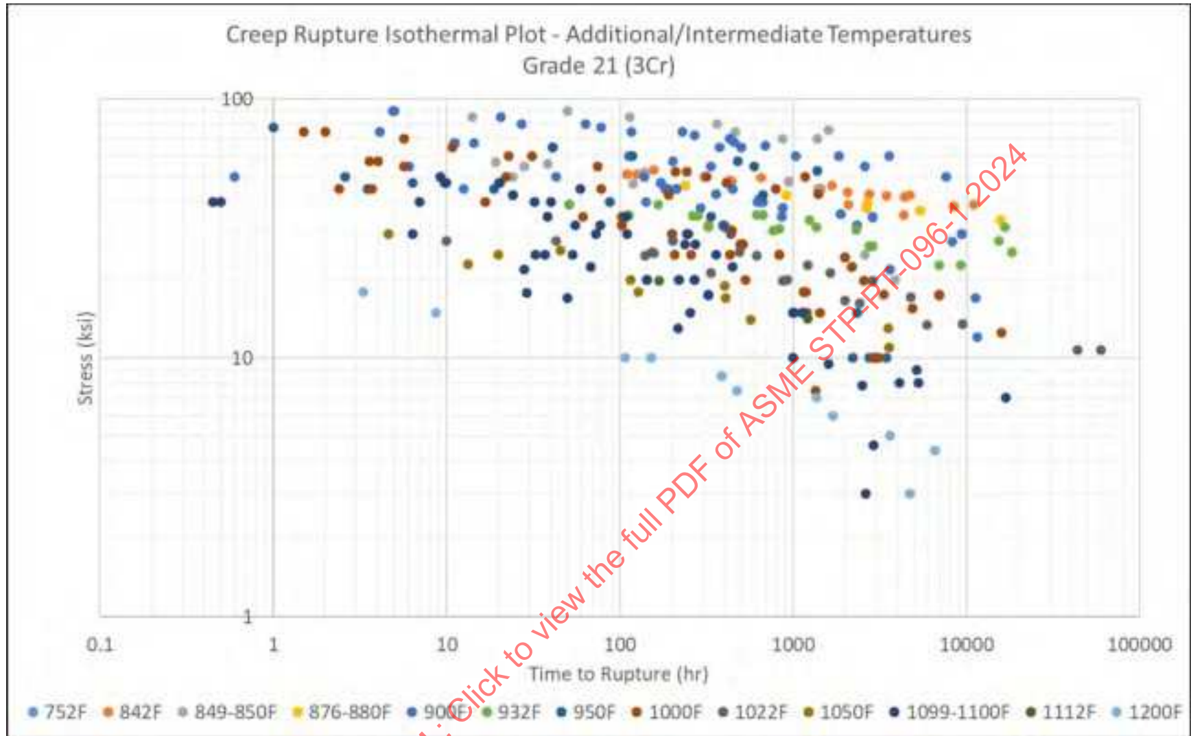
Figure 24-9: 3Cr Creep Rupture Isotherm Curves for Additional and Intermediate Temperatures
