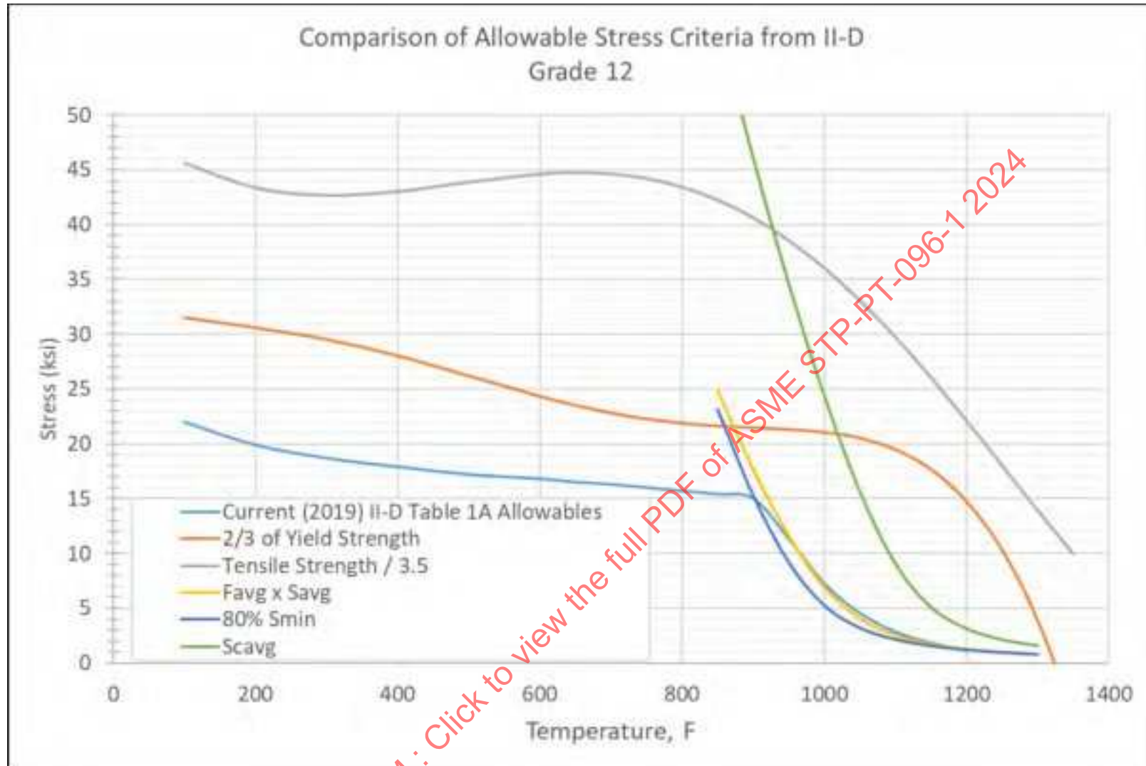
Figure 22-13: Comparison of Current Grade 12 Allowable Stresses Vs. ASME II-D Appendix 1 Criteria Applied to Data
