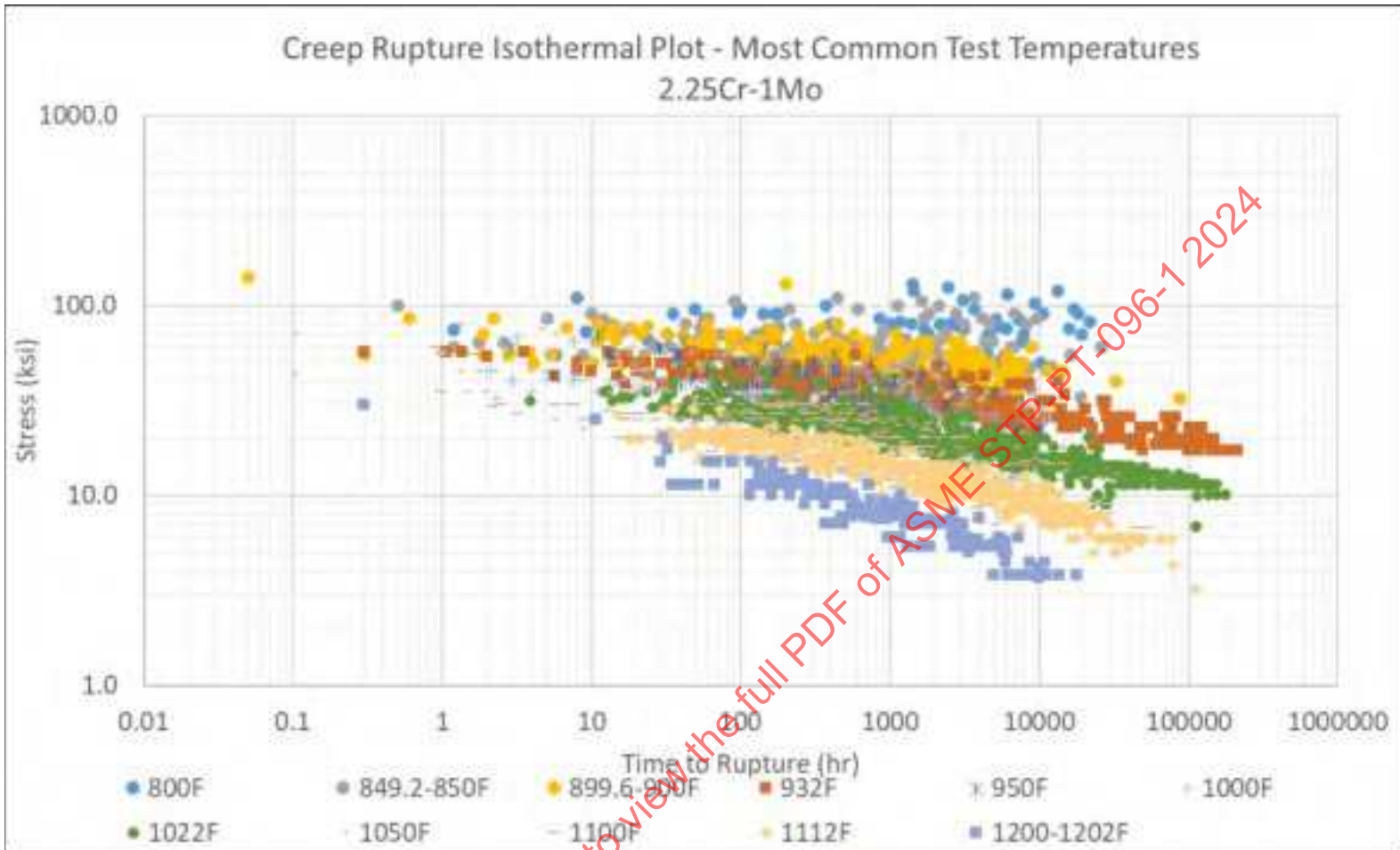
Figure 10-8: Grade 22 Creep Rupture Isotherm Curves, Temperatures With High Concentration of Data Points
