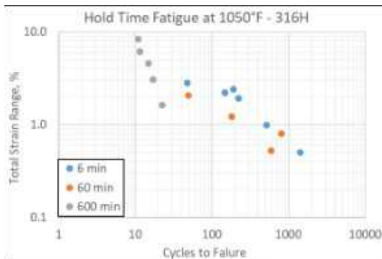
Figure 17-19: Hold Time Data (Creep Fatigue) for 316H, Temperature of 1050°F
