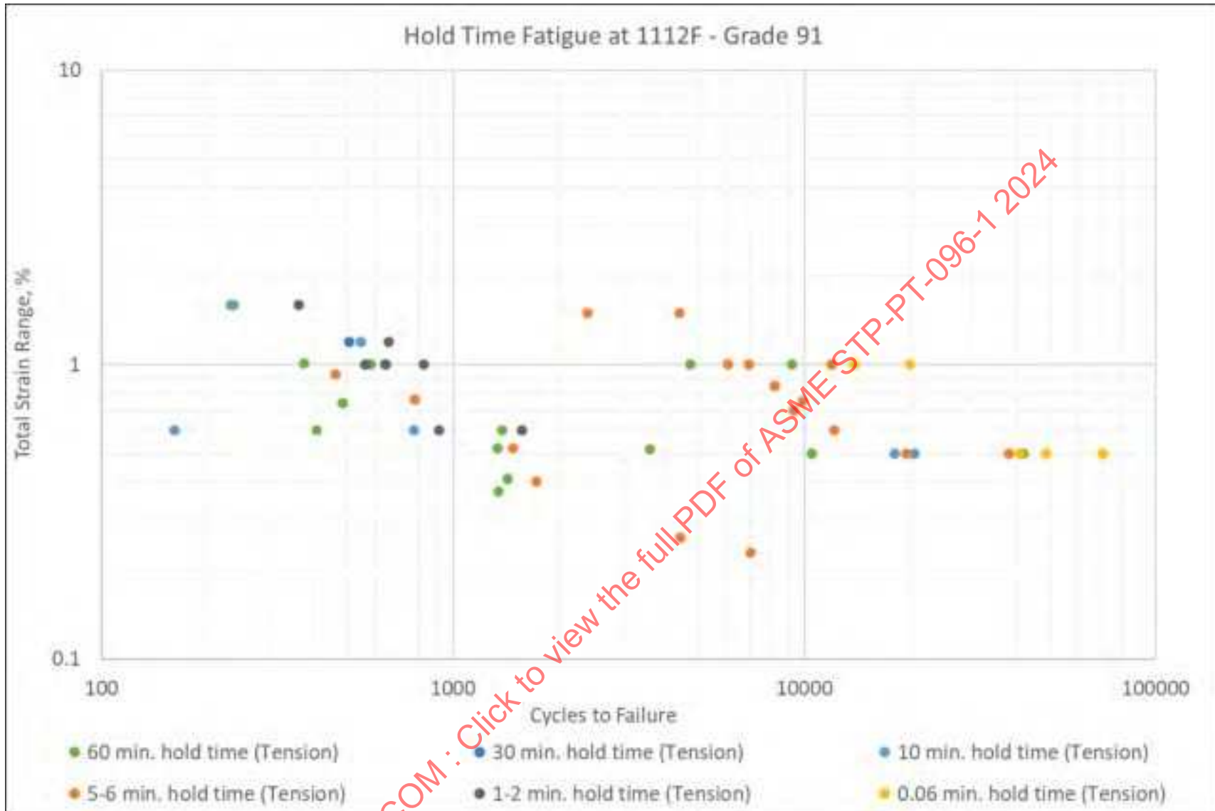
Figure 4-23: Grade 91 Hold Time Data (Creep Fatigue) For Grade 91, Temperature of 1112°F
