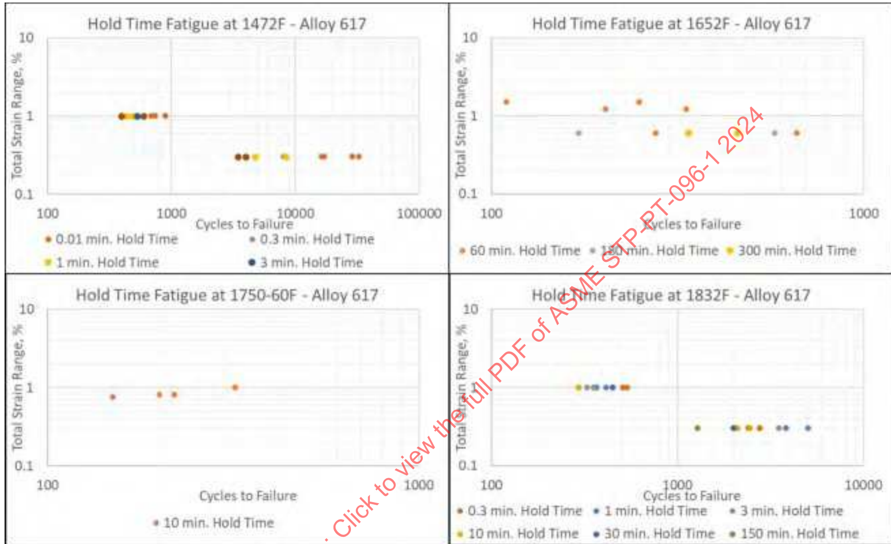
Figure 19-18: Alloy 617 Hold Time Data (Creep Fatigue) for Alloy 617, Temperatures of 1472°F, 1652°F, 1750-60°F, & 1832°F
