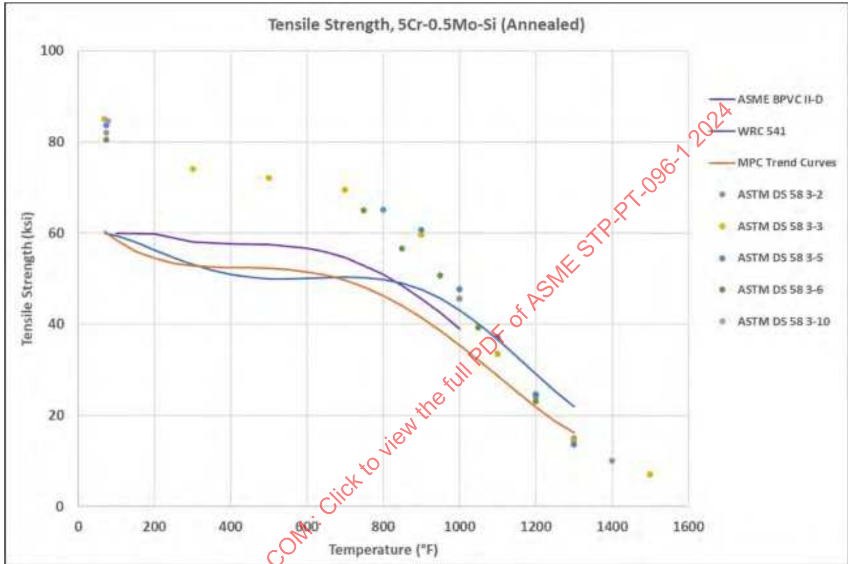
Figure 13-3: 5Cr-0.5Mo-Si (Annealed) Strength Vs. Temperature, By Data Source, Including Trend Curves
