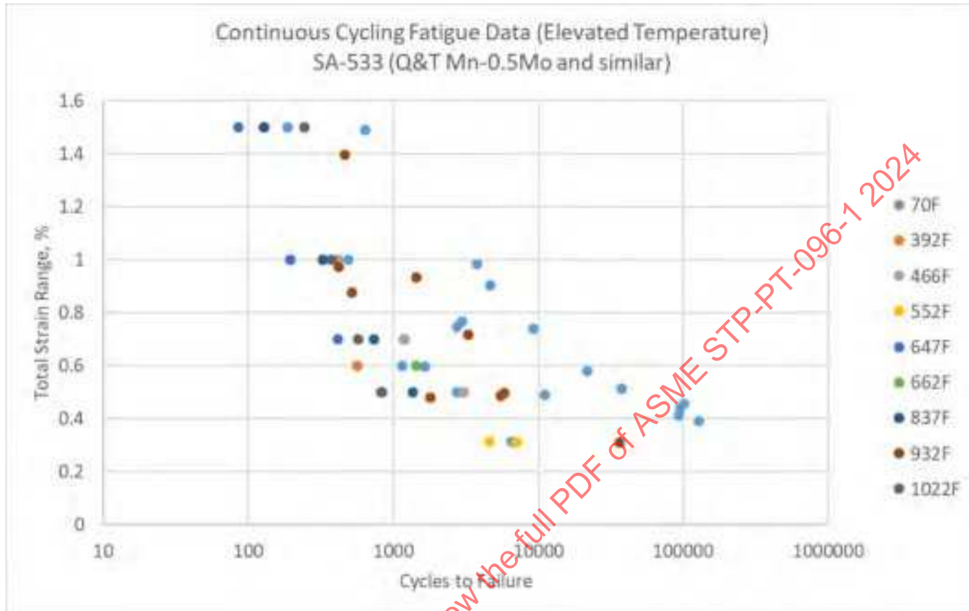
Figure 7-14: SA-533 (Q&T Mn-0.5Mo and Similar) Continuous Cycling Fatigue, Elevated Temperature Data
