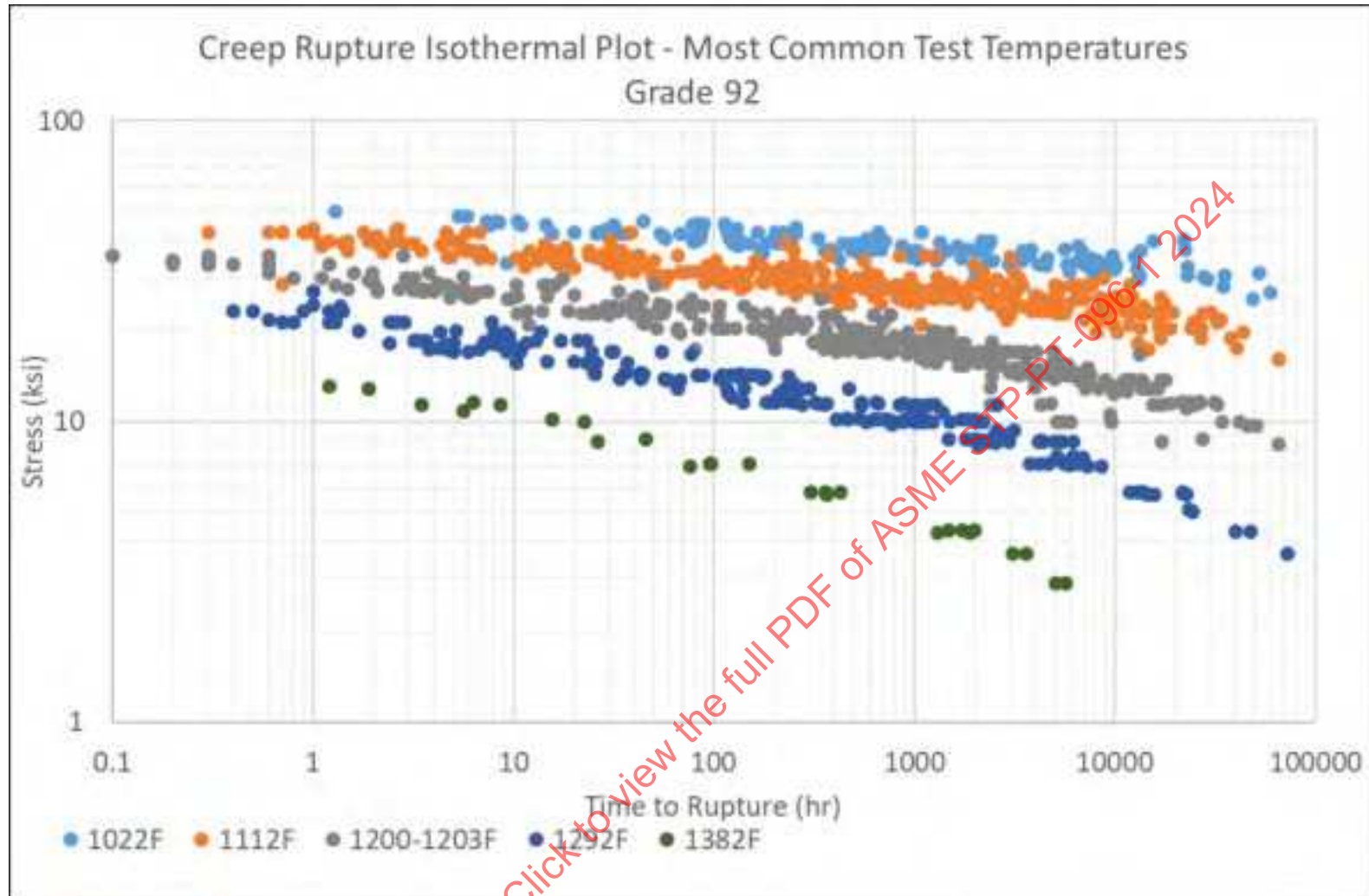
Figure 15-8: Grade 92 Creep Rupture Isotherm Curves, Temperatures With High Concentration of Data Points
