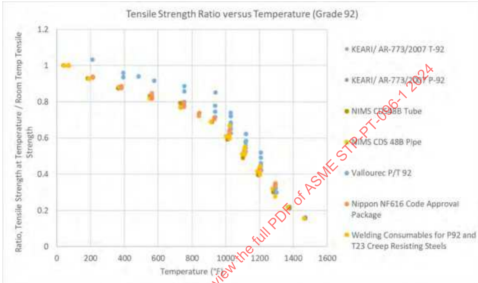
Figure 15-5: Grade 92 Tensile Strength Ratios Vs. Temperature (Calculated on a Heat-By-Heat Basis, By Data Source)
