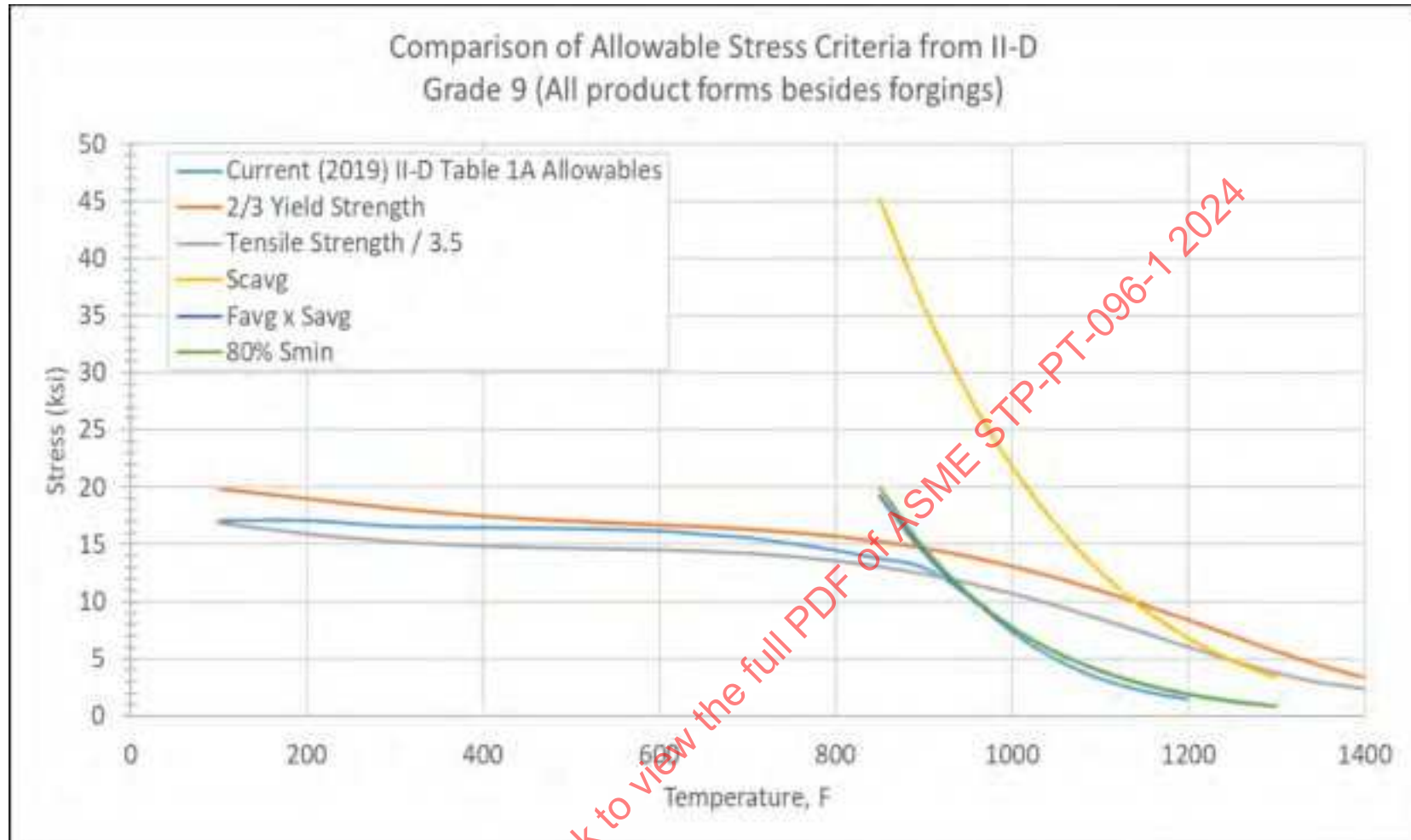
Figure 14-14: Comparison of Current Grade 9 Allowable Stresses (Annealed) Vs. ASME II-D Appendix 1 Criteria Applied to Data
