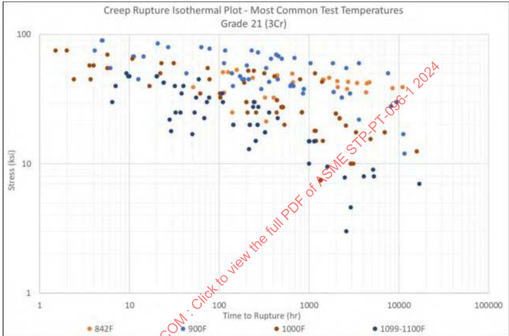
Figure 24-8: 3Cr Creep Rupture Isotherm Curves, Temperatures With High Concentration of Data Points
