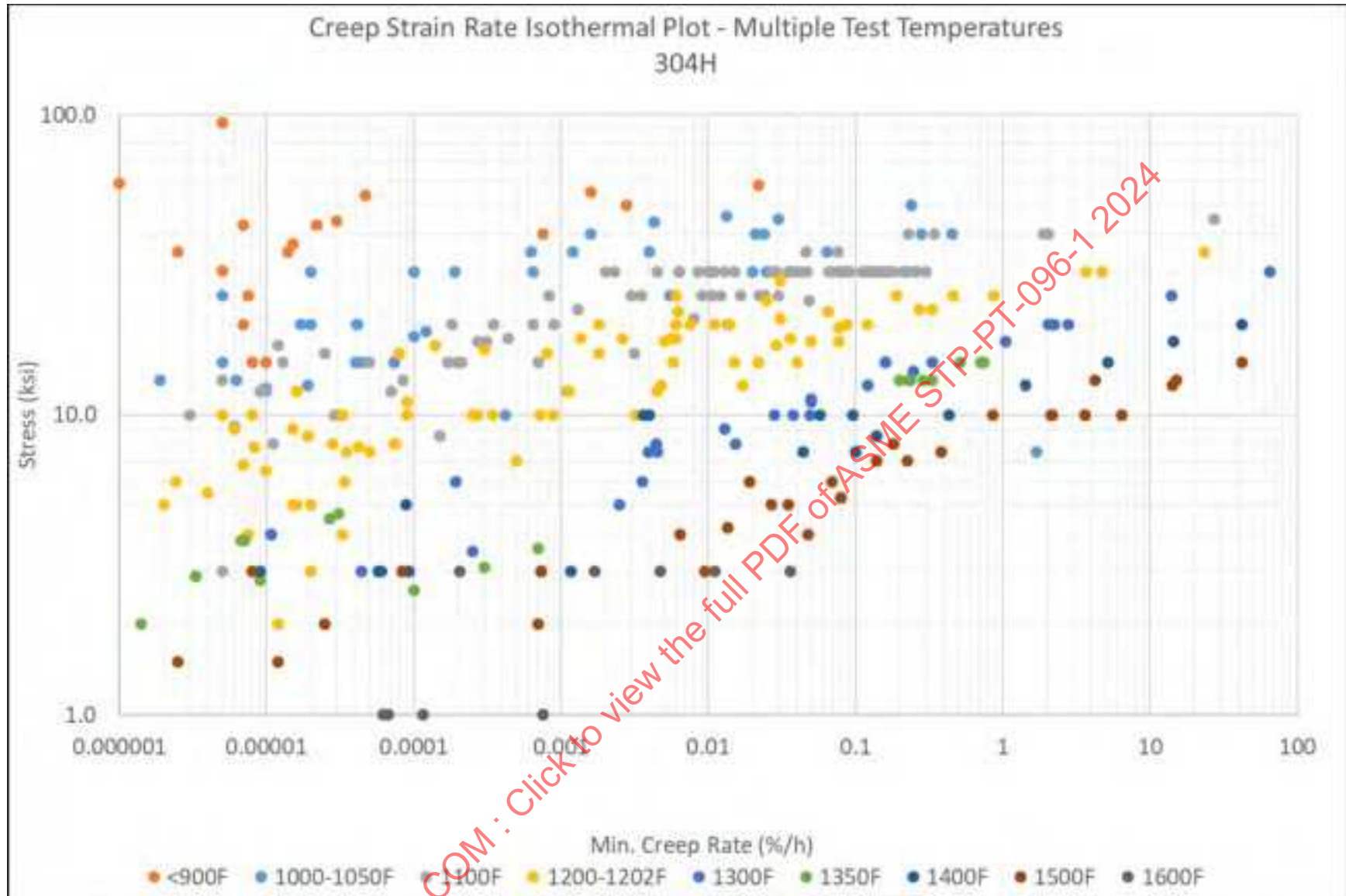
Figure 16-10: 304H Creep Strain Rate (MCR) Isotherm Curves, Temperatures with High Concentration of Data Points
