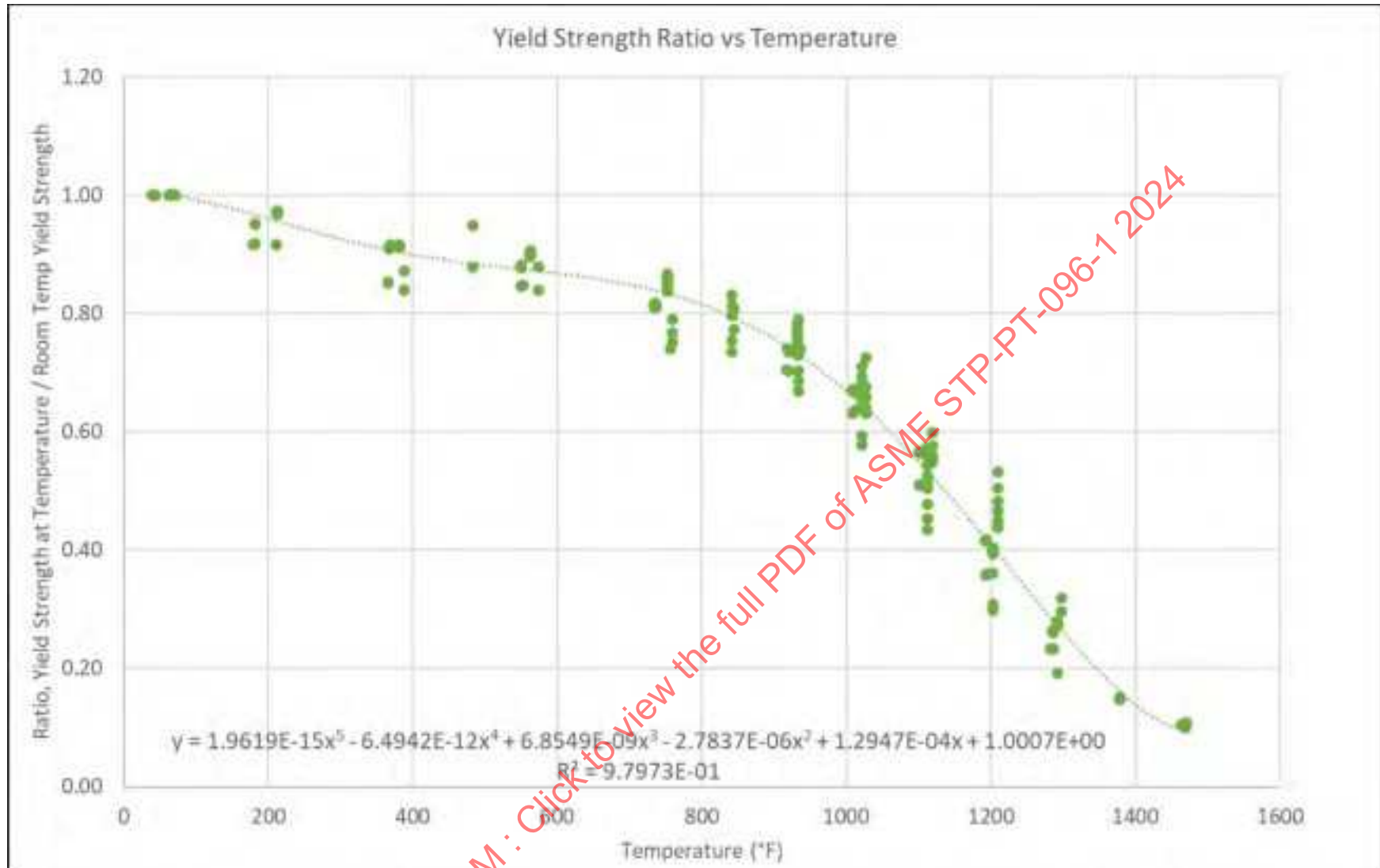
Figure 15-6: Grade 92 Yield Strength Ratios Vs. Temperature, All Combined Data, With Polynomial Regression
