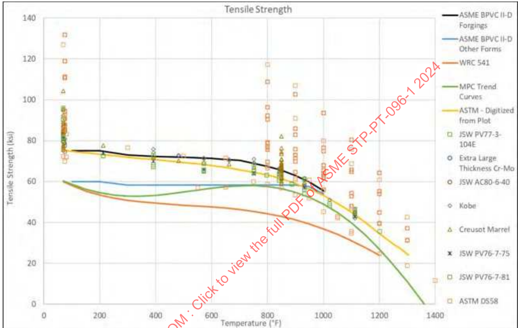
Figure 24-3: 3Cr Tensile Strength Vs. Temperature, By Data Source, Including Trend Curves
