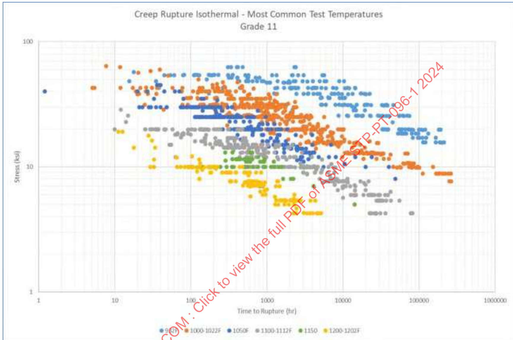
Figure 9-8: Grade 11 Creep Rupture Isotherm Curves, Temperatures With High Concentration of Data Points
