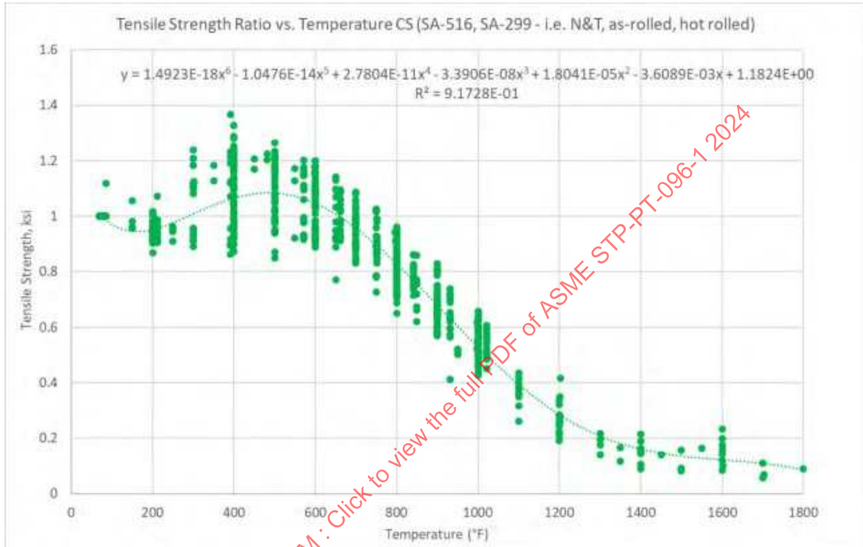
Figure 5-7: CS (516/299) Tensile Strength Ratios Vs. Temperature, All Combined Data, With Polynomial Regression
