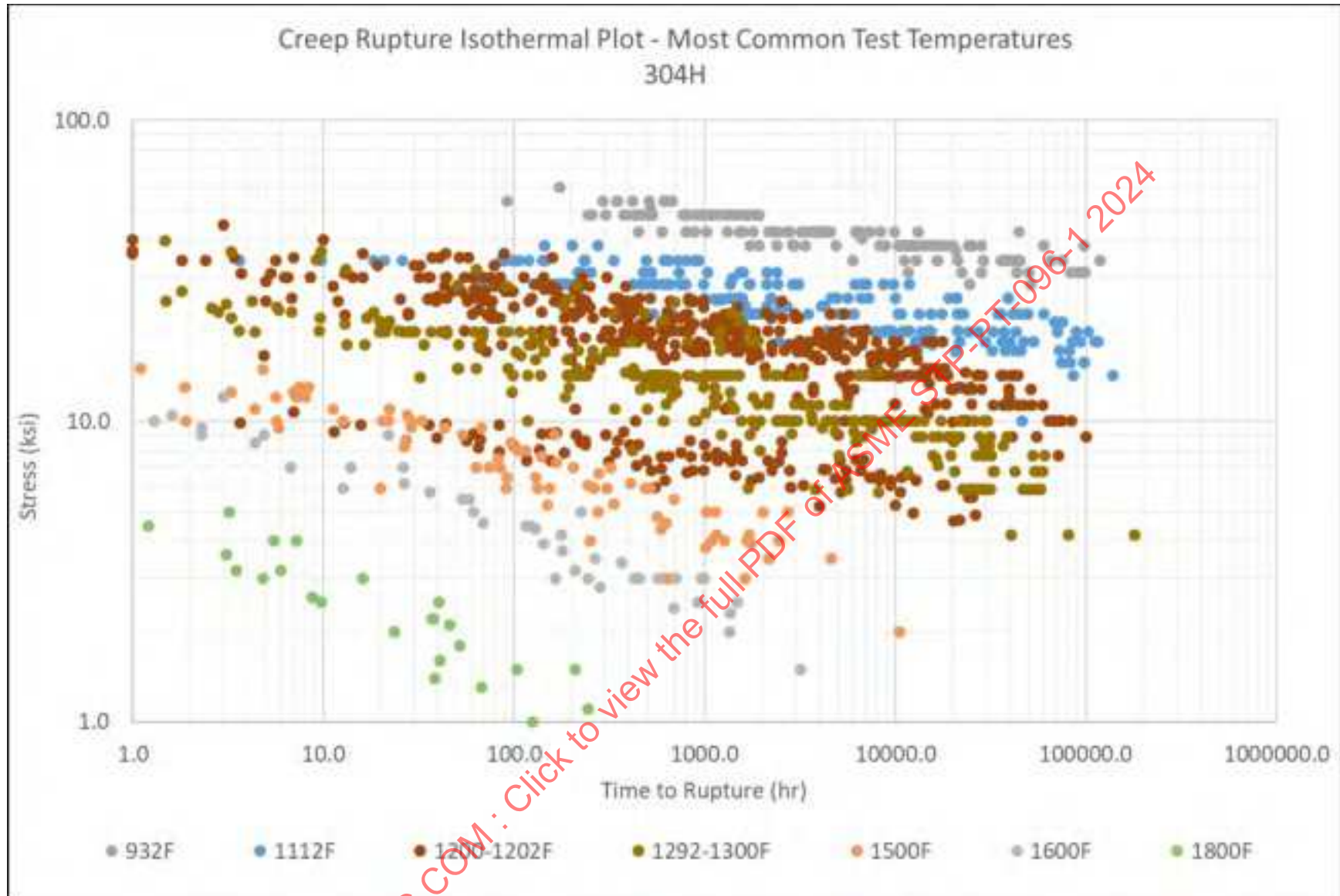
Figure 16-8: 304H Creep Rupture Isotherm Curves, Temperatures With High Concentration of Data Points
