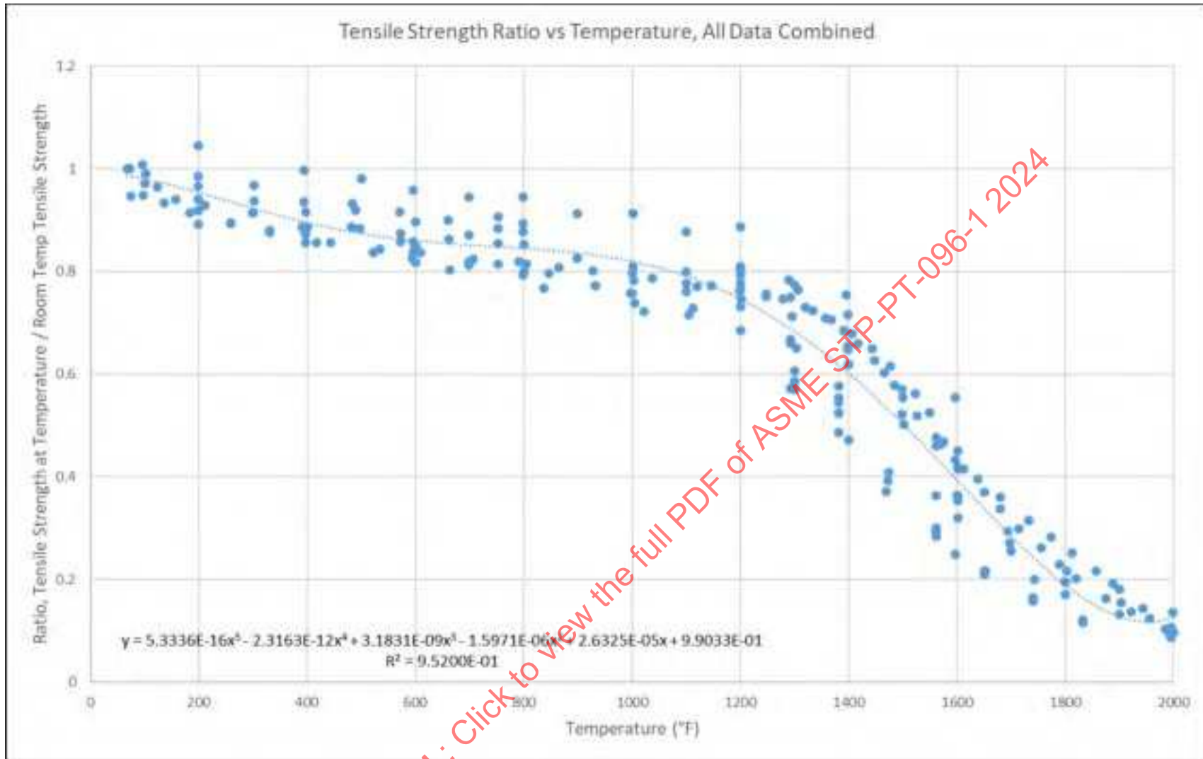
Figure 19-7: Alloy 617 Tensile Strength Ratios Vs. Temperature, All Combined Data, With Polynomial Regression
