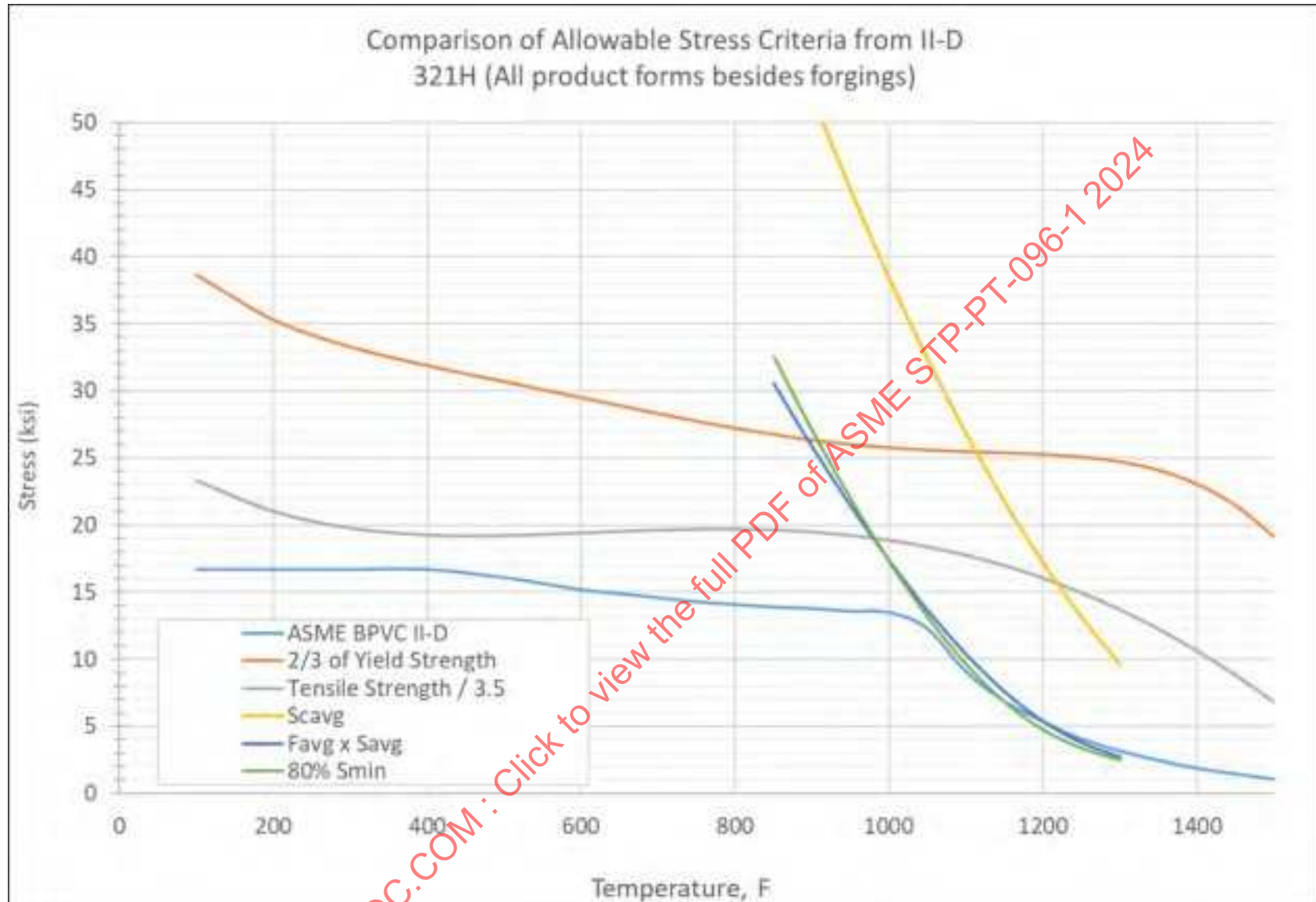
Figure 26-14: Comparison of Current 321H Allowable Stresses (Except Forgings) Vs. ASME II-D Appendix 1 Criteria Applied to Data
