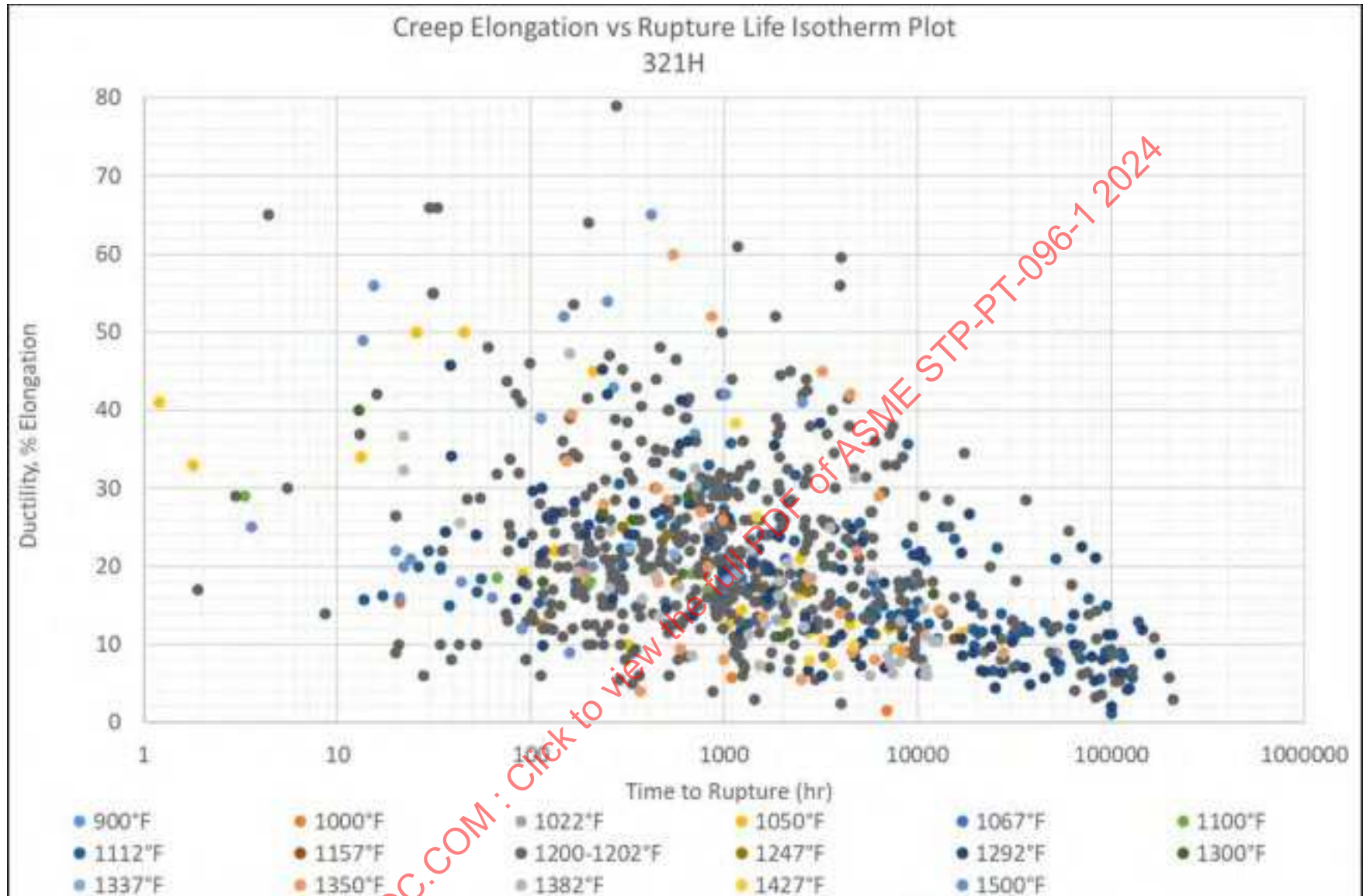
Figure 26-12: 321H Creep Ductility (% Elongation) Vs. Rupture Time Isotherms
