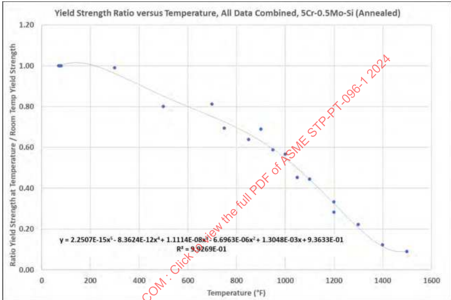
Figure 13-10: 5Cr-0.5Mo-Si (Annealed) Yield Strength Ratios Vs. Temperature, All Combined Data, With Polynomial Regression
