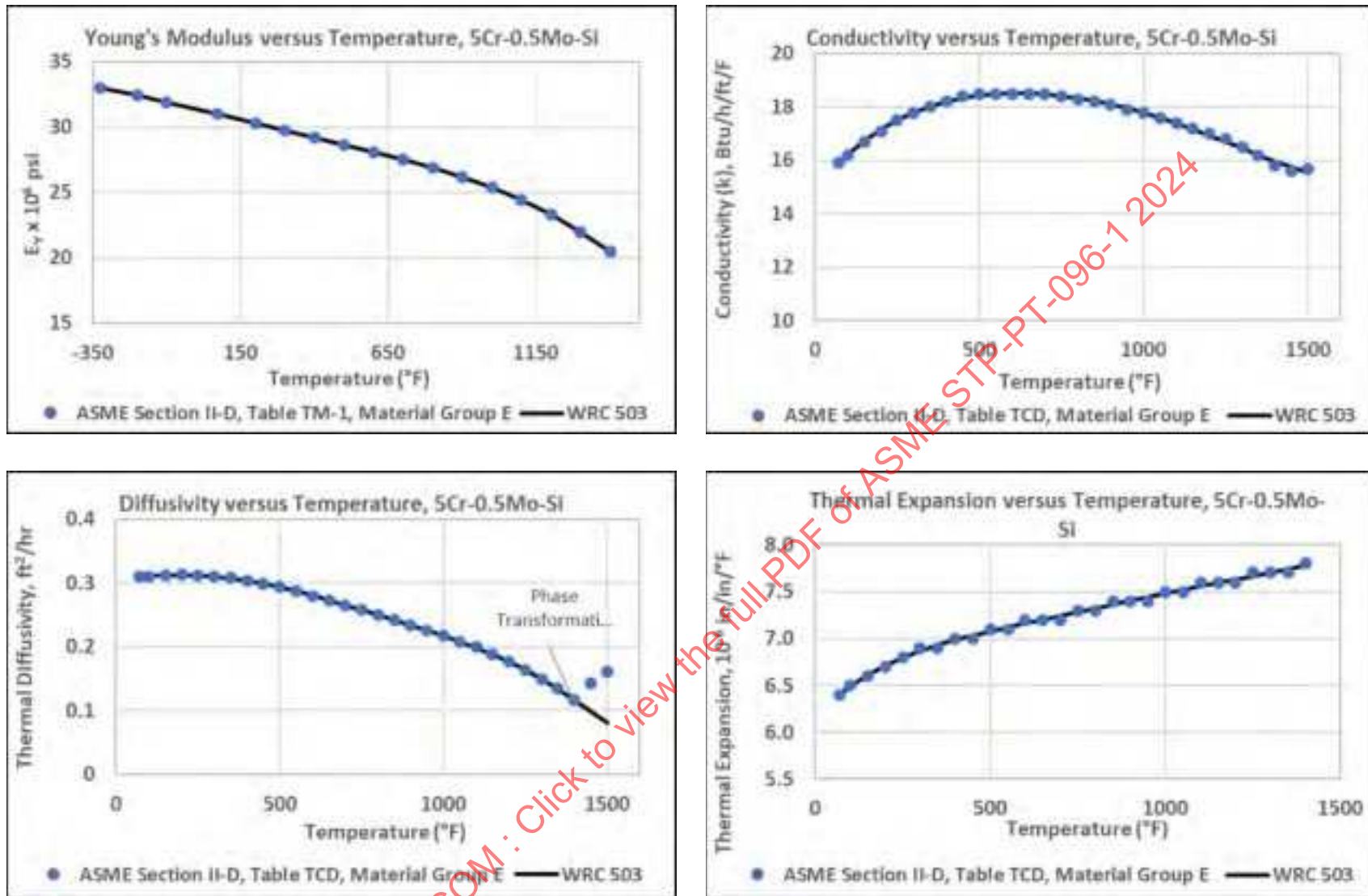
Figure 13-1: 5Cr-0.5Mo-Si Modulus ( E_y ), Thermal Conductivity ( k ), Thermal Diffusivity (TD), & Thermal Expansion ( \alpha ) With Temperature
