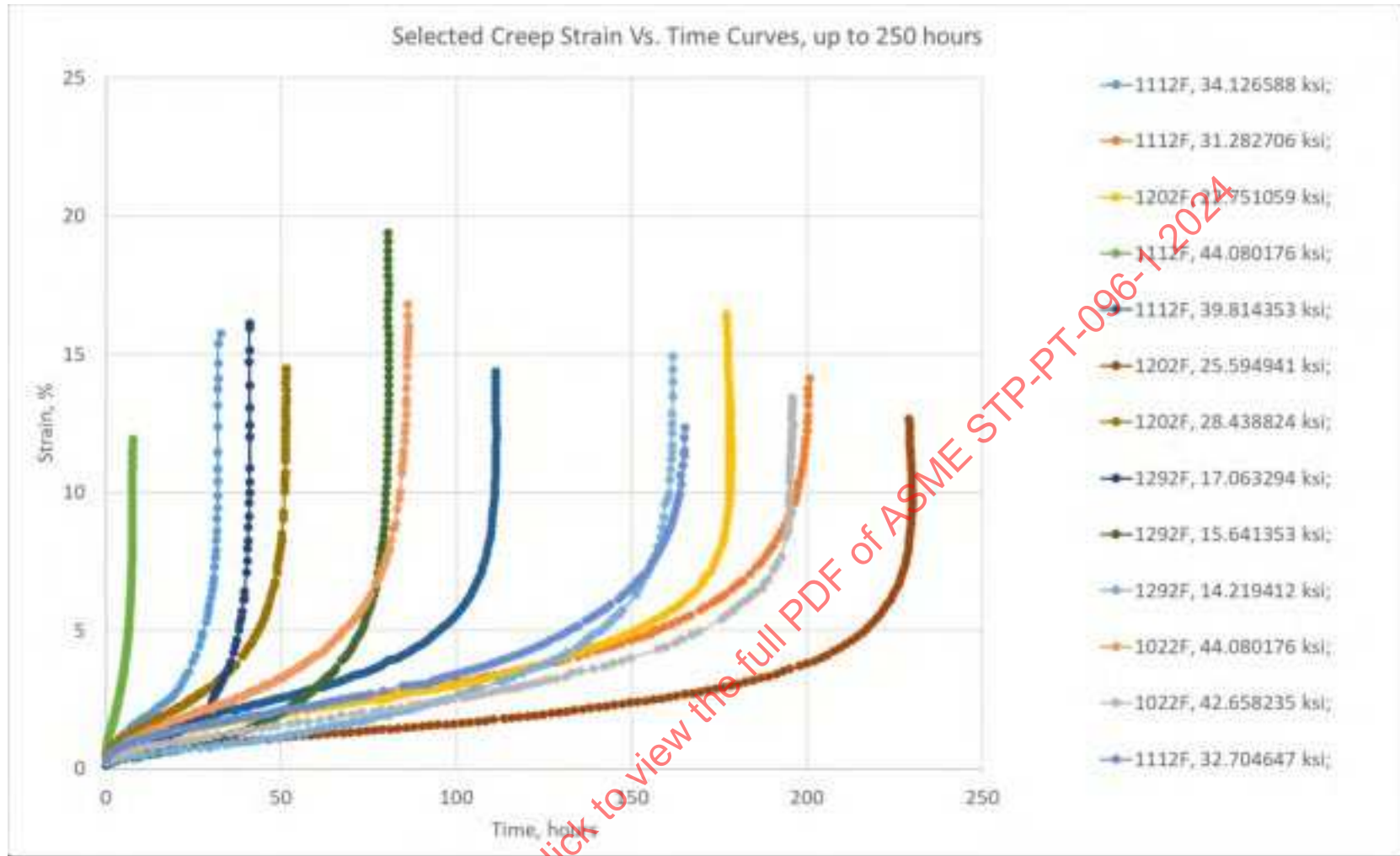
Figure 15-14: Short-Term Strain Vs. Time Data, Up to 250 Hour Test Durations (Grade 92)
