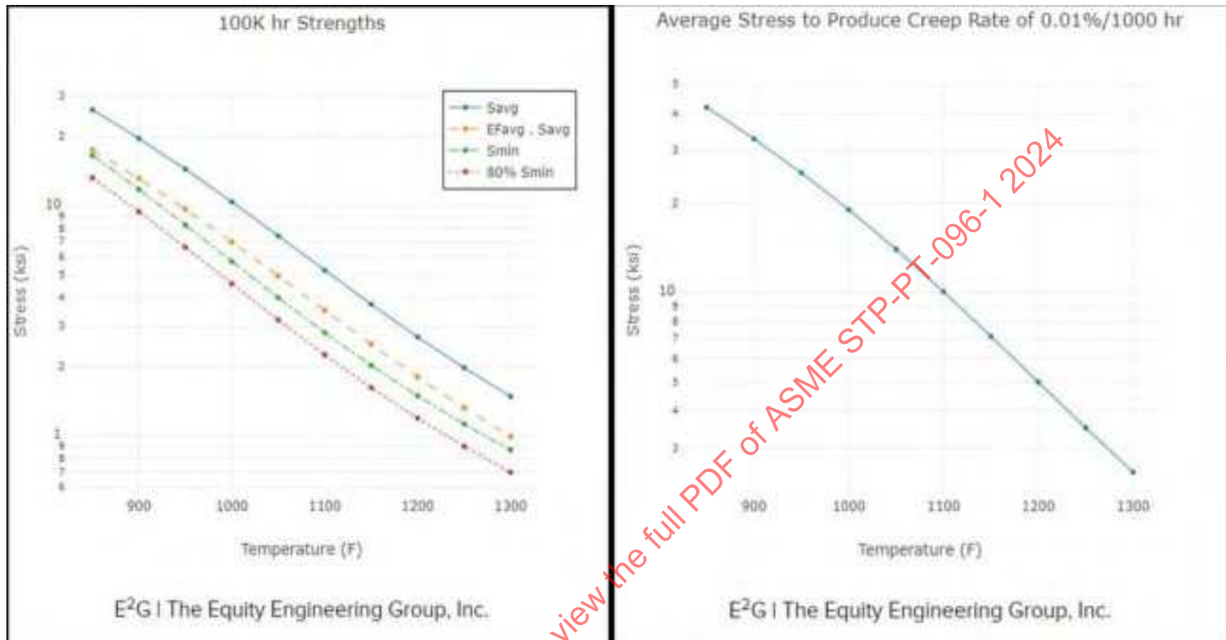
Figure 25-13: Calculated Allowable Stresses Based on Rupture and Creep Strain Rate and ASME II-D Appendix 1 Criteria (Type 410/12Cr)
