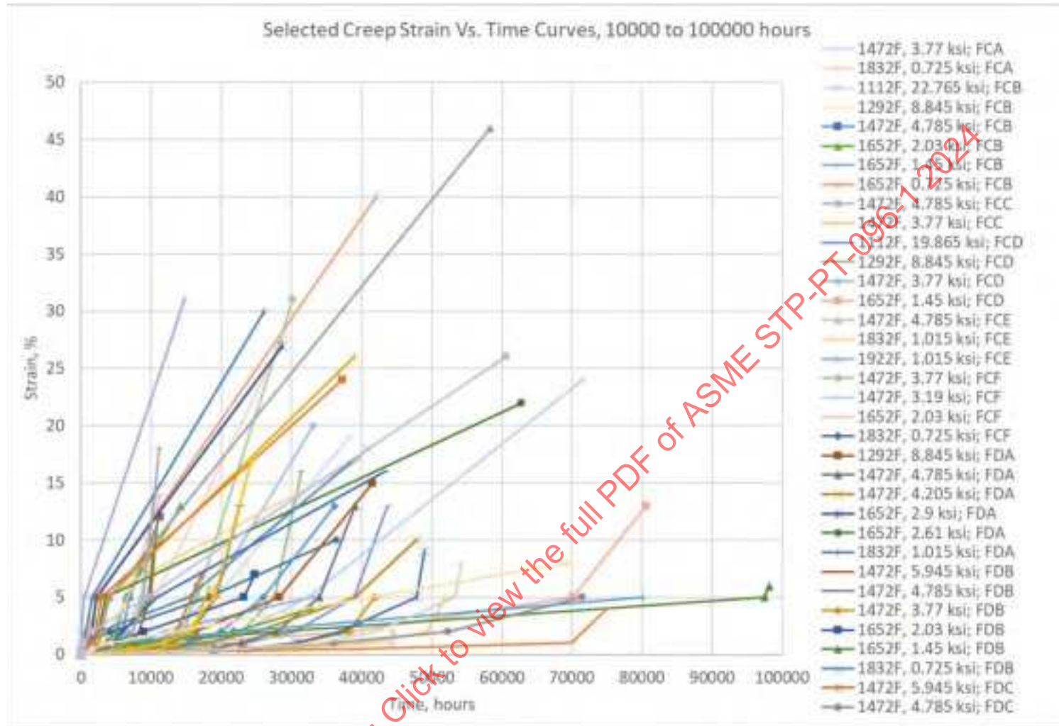
Figure 21-19: Long-Term Strain Vs. Time Data, 10,000 to 100,000 Hour Test Durations (Alloy 800H)
