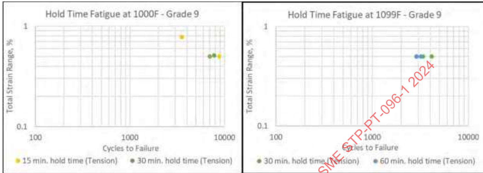
Figure 14-20: Grade 9 Hold Time Data (Creep Fatigue) for Grade 9, Temperatures of 1000°F & 1099°F
