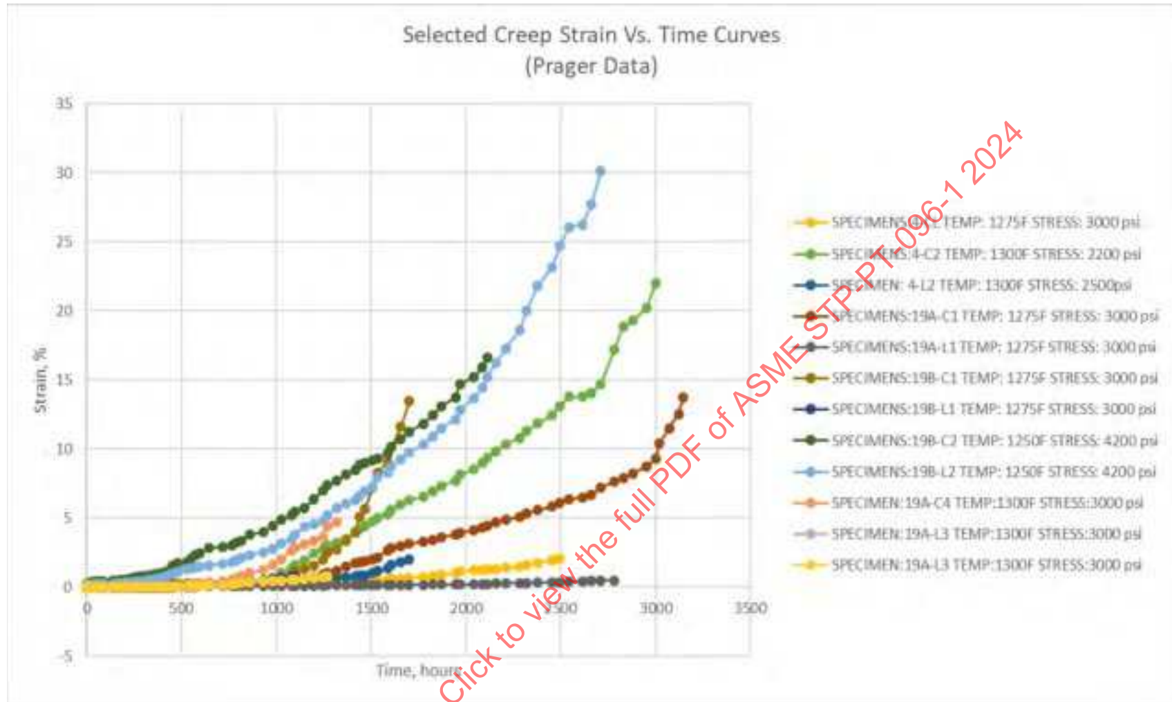
Figure 10-17: Creep Strain Vs. Time Data, (Grade 22) 3 of 3
