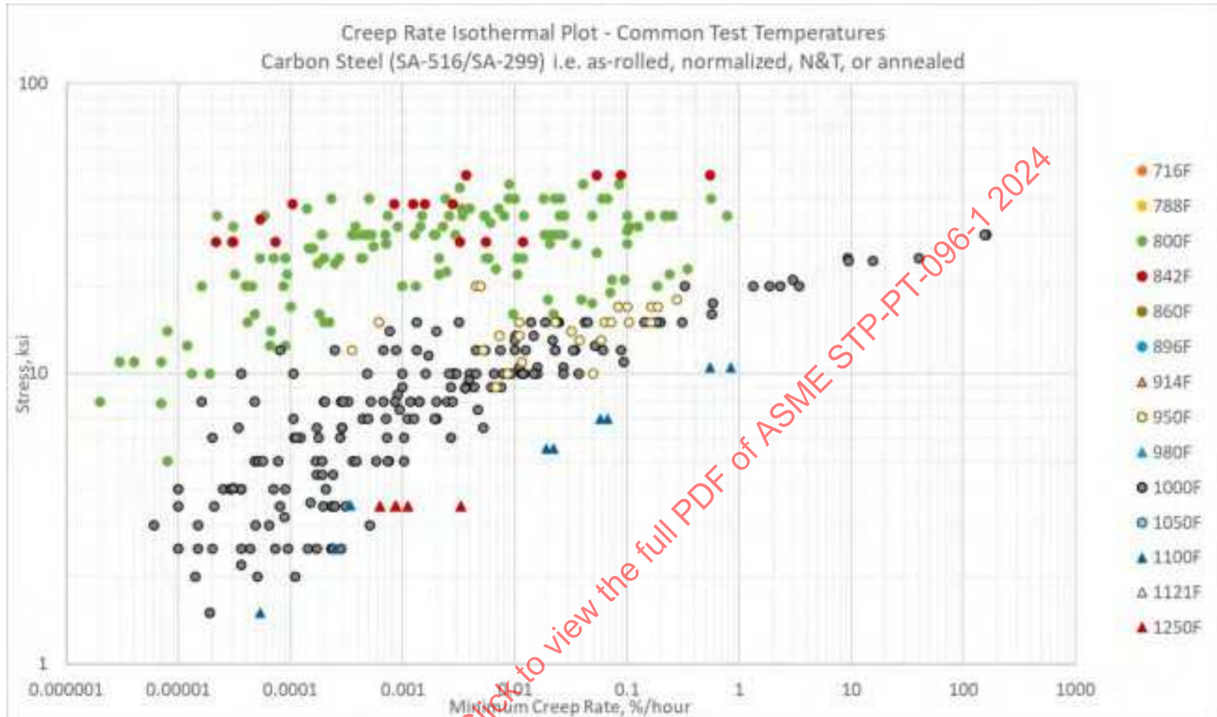
Figure 5-11: CS (516/299) Creep Strain Rate (MCR) Isotherm Curves, 2 of 3
