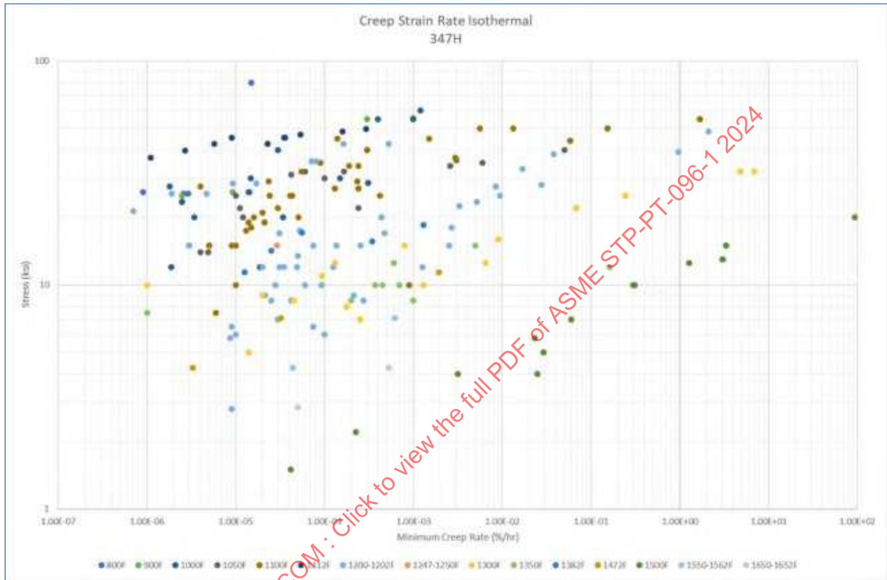
Figure 18-10: 347H Creep Strain Rate (MCR) Isotherm Curves
