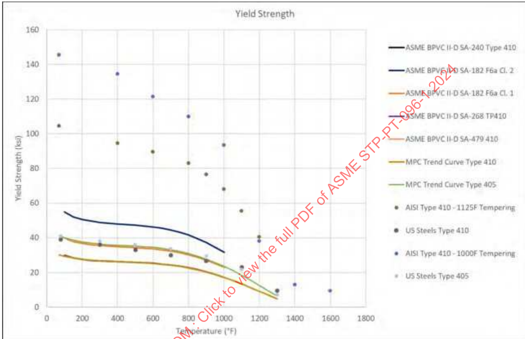
Figure 25-2: Type 410/12Cr Yield Strength Vs. Temperature, By Data Source, Including Trend Curves
