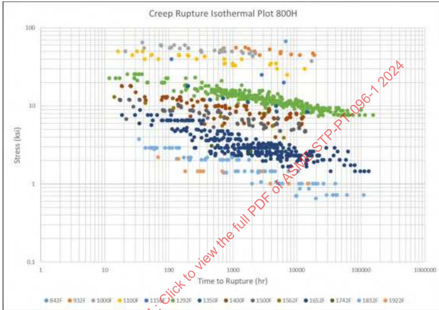
Figure 21-8: Alloy 800H Creep Rupture Isotherm Curves, First Lot of Temperatures
