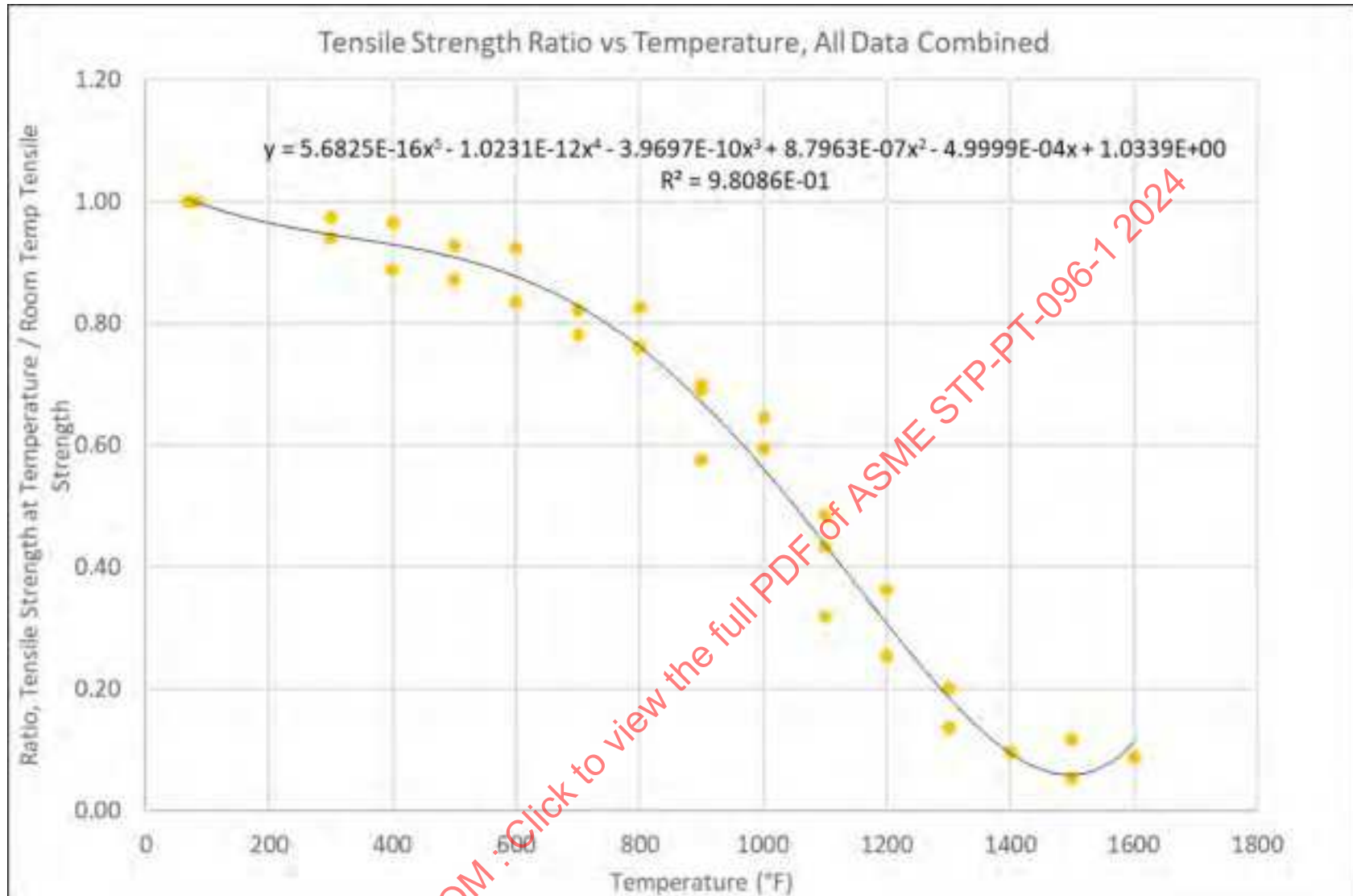
Figure 25-7: Type 410/12Cr Tensile Strength Ratios Vs. Temperature, All Combined Data, With Polynomial Regression
