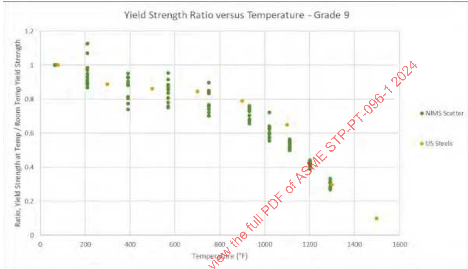
Figure 14-4: Grade 9 Yield Strength Ratios Vs. Temperature (Calculated on a Heat-By-Heat Basis, By Data Source)
