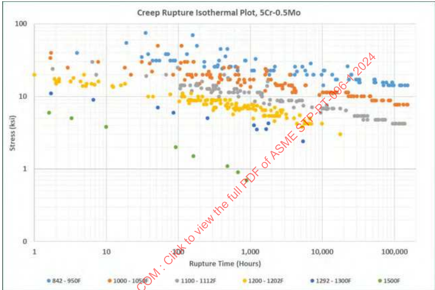
Figure 12-14: Grade 5 Creep Rupture Isotherm Curves
