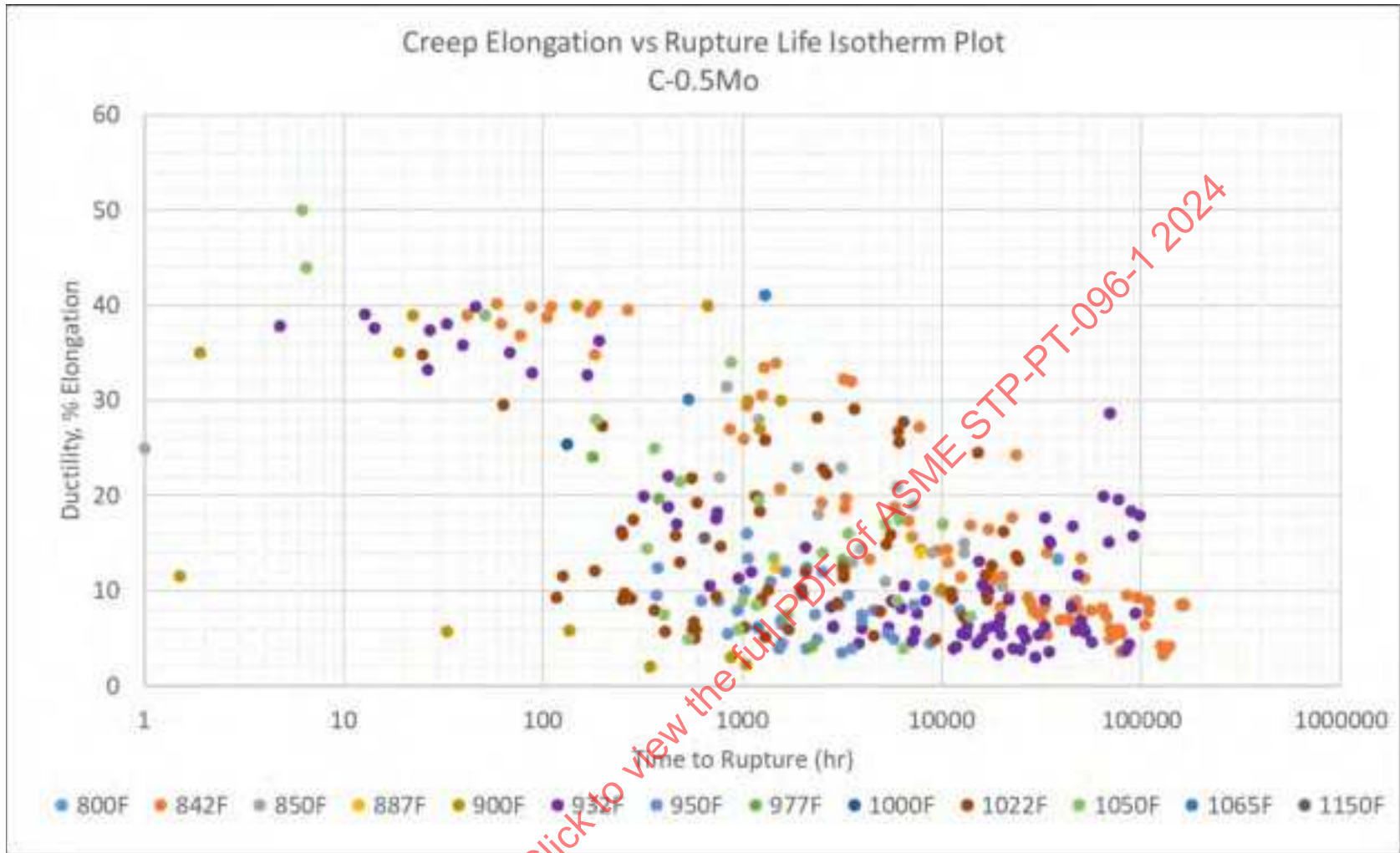
Figure 8-12: C-1/2Mo Creep Ductility (% Elongation) Vs. Rupture Time Isotherms
