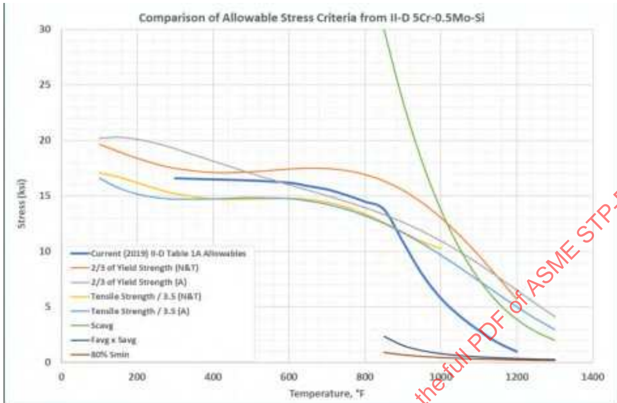
Figure 13-19: Comparison of Current 5Cr-0.5Mo-Si Allowable Stresses Vs. ASME II-D Appendix 1 Criteria Applied to Data
