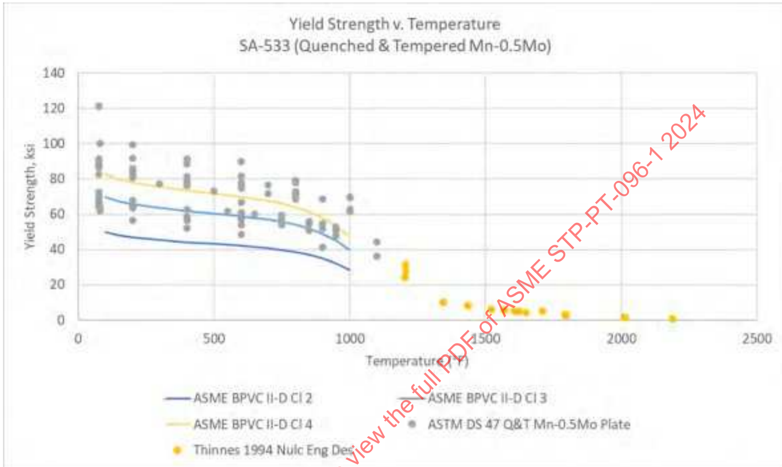
Figure 7-1: SA-533 (Q&T Mn-0.5Mo) Yield Strength Vs. Temperature, By Data Source, Including Trend Curves
