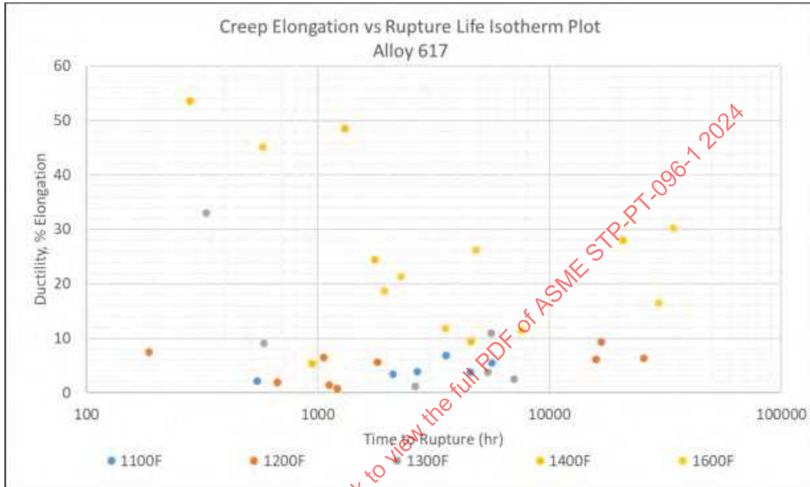
Figure 19-12: Alloy 617 Creep Ductility (% Elongation) Vs. Rupture Time Isotherms
