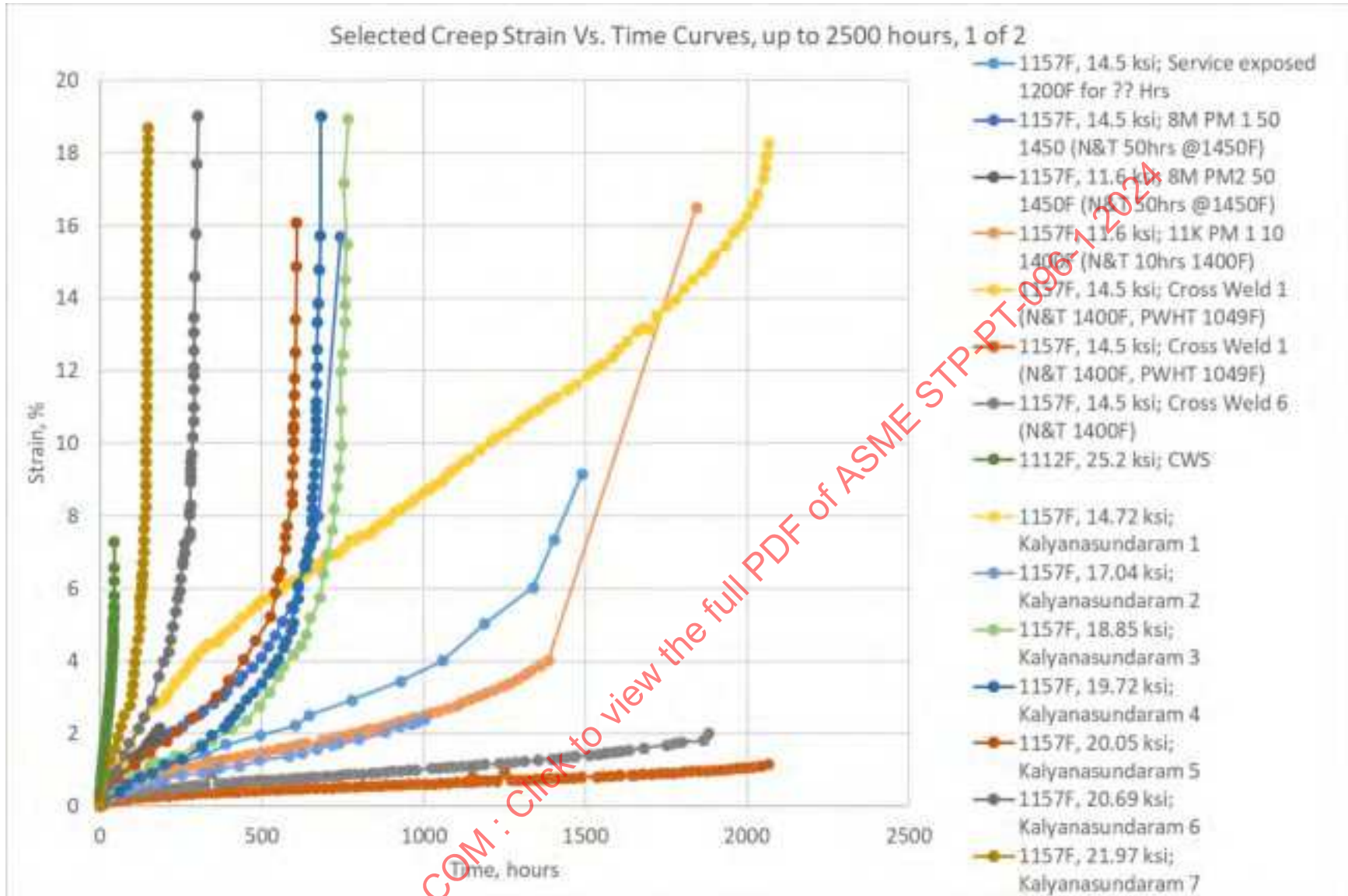
Figure 4-15: Short-Term Strain Vs. Time Data, up to 2,500 Hour Test Durations (Grade 91), 1 of 2
