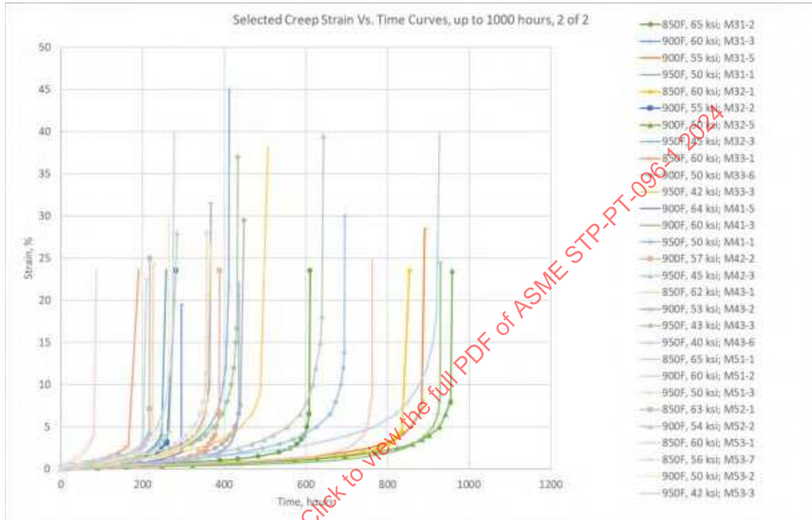
Figure 11-15: Short-Term Strain Vs. Time Data, up to 1,000 Hour Test Durations (Grade 22V), 2 of 2
