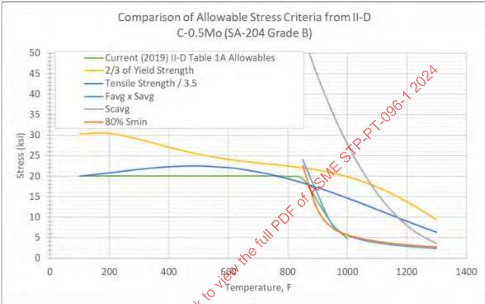
Figure 8-14: Comparison of Current C-1/2Mo Allowable Stresses (SA-204 Grade B) Vs. ASME II-D Appendix 1 Criteria Applied to Data
