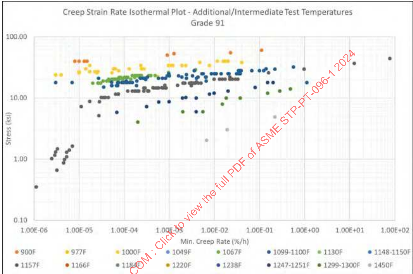
Figure 4-11: Grade 91 Creep Strain Rate (MCR) Isotherm Curves for Additional and Intermediate Temperatures
