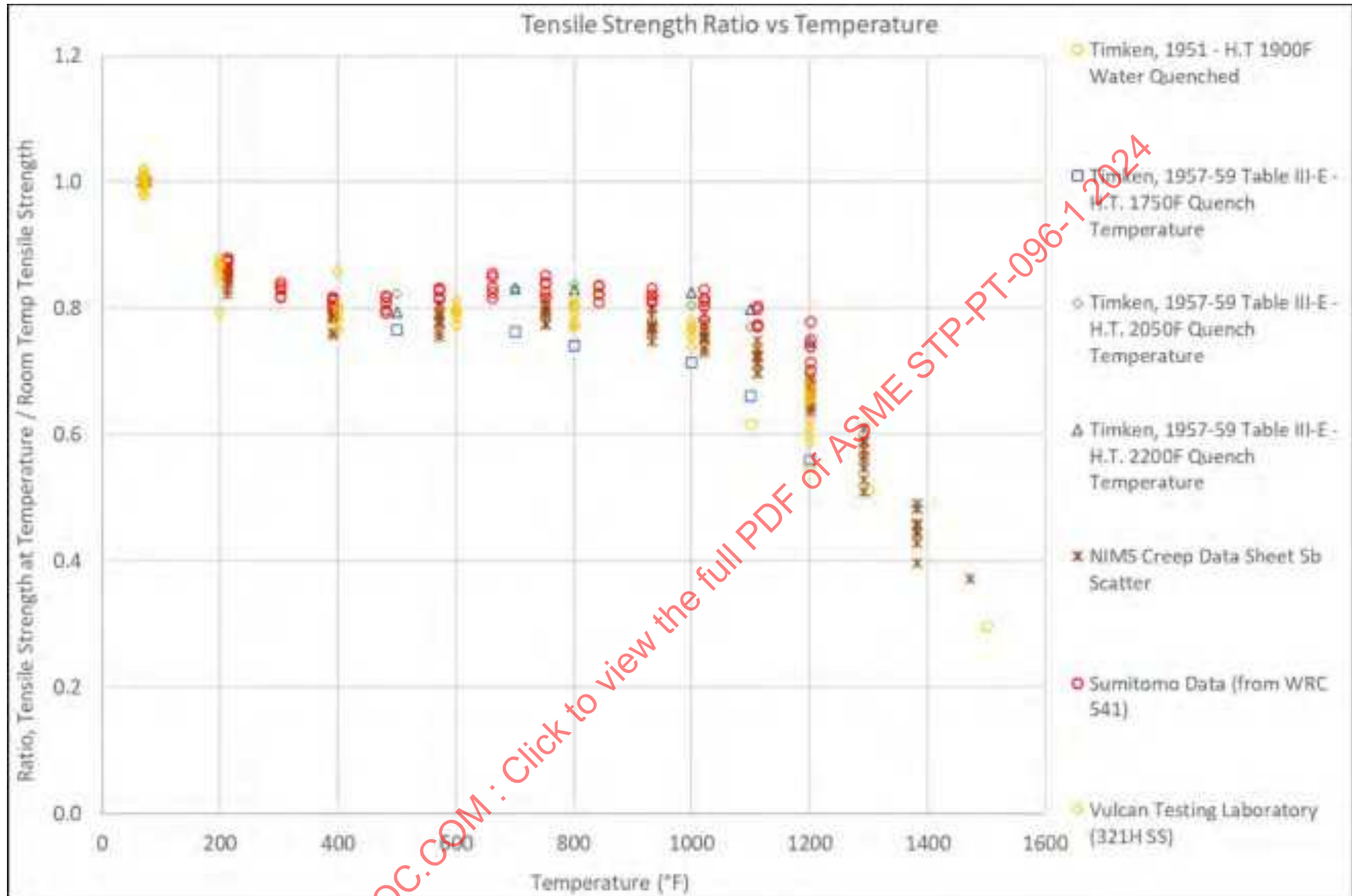
Figure 26-5: 321H Tensile Strength Ratios Vs. Temperature (Calculated on a Heat-By-Heat Basis, By Data Source)
