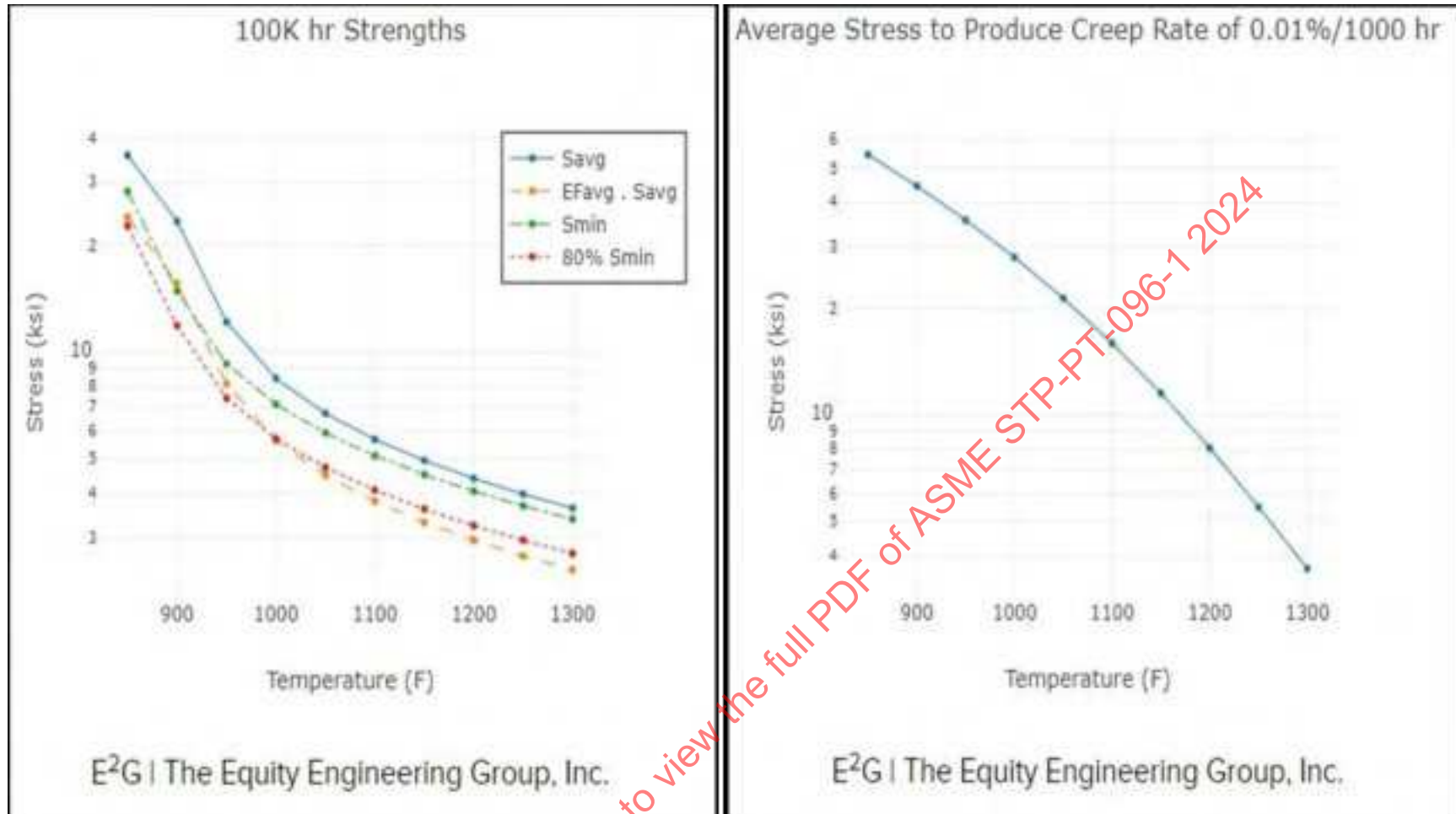
Figure 8-13: Calculated Allowable Stresses Based on Rupture and Creep Strain Rate and ASME II-D Appendix 1 Criteria (C-1/2Mo)
