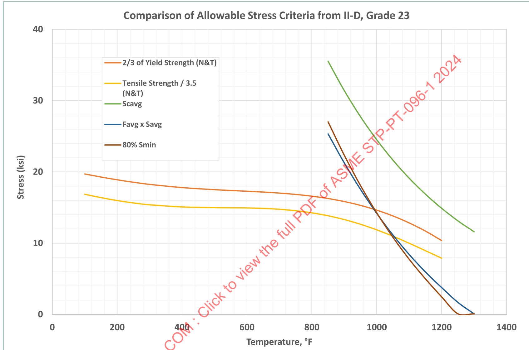
Figure 23-13: Comparison of ASME II-D Appendix 1 Criteria Applied to Grade 23 Data
