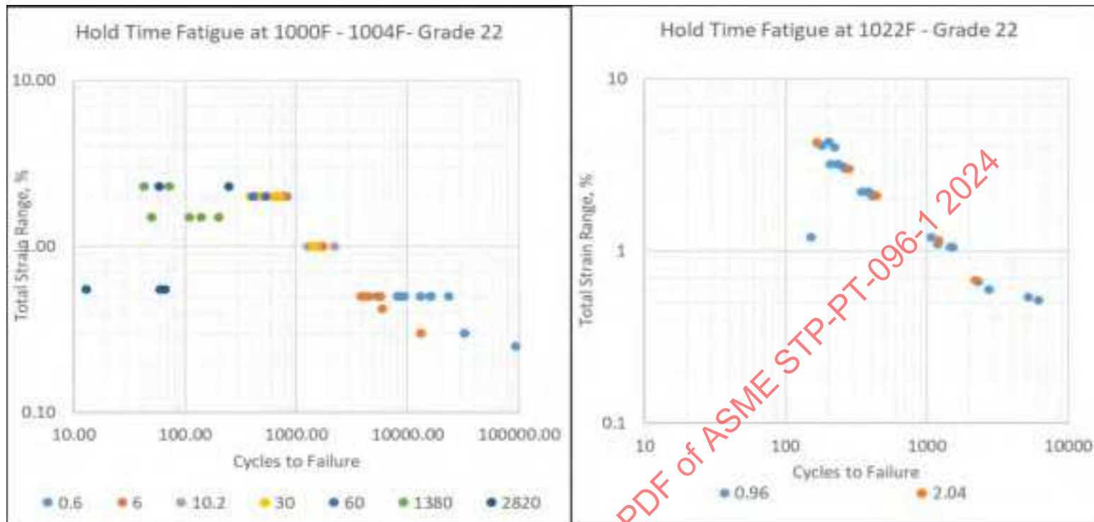
Figure 10-20: Grade 22 Hold Time Fatigue Data at Selected Elevated Temperatures, 2 of 2
