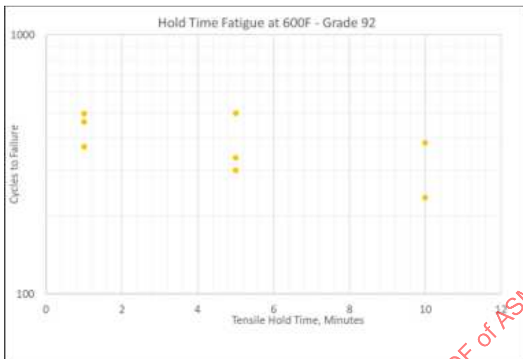
Figure 15-18: Grade 92 Hold Time Data (Creep Fatigue) for Grade 92, Temperature of 600°F
