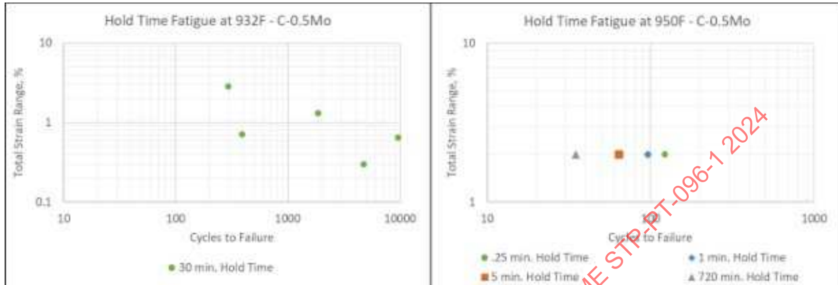
Figure 8-19: C-1/2Mo Hold Time Data (Creep Fatigue) for C-1/2Mo, Temperatures of 932°F and 950°F
