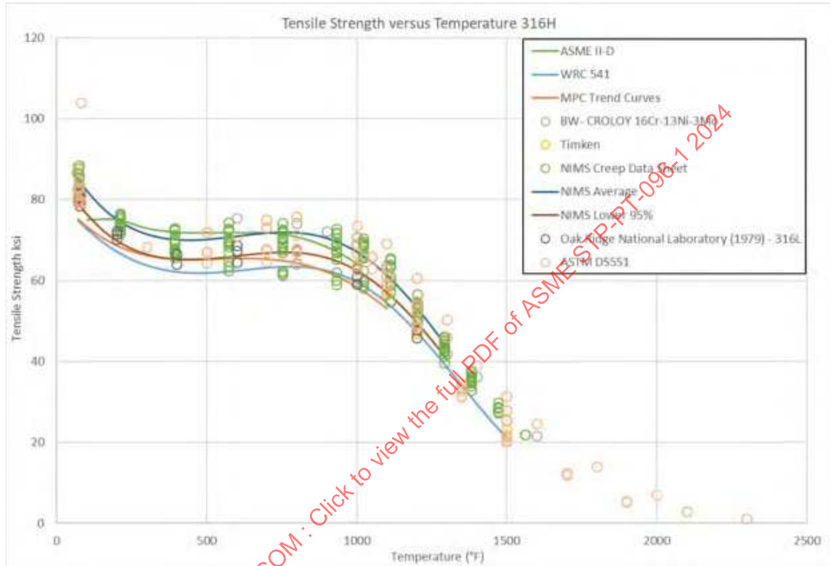
Figure 17-3: 316H Tensile Strength Vs. Temperature, By Data Source, Including Trend Curves
