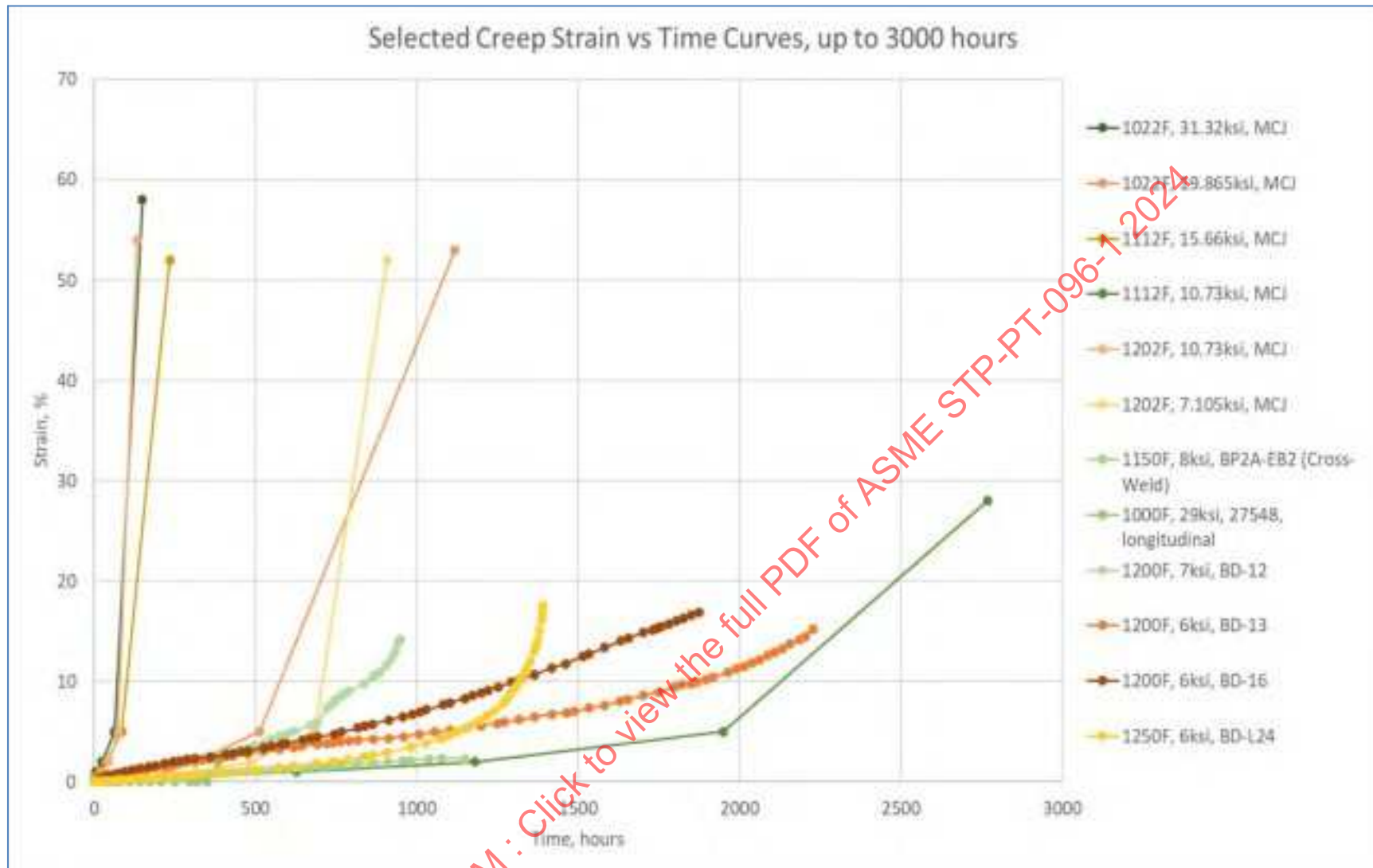
Figure 9-14: Creep Strain Vs. Time Data, up to 3,000 Hour Test Durations (Grade 11)
