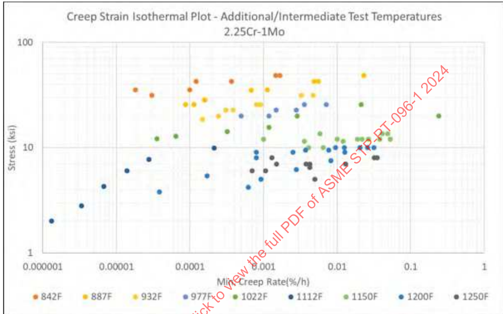
Figure 10-11: Grade 22 Creep Strain Rate (MCR) Isotherm Curves for Additional/Intermediate Temperatures
