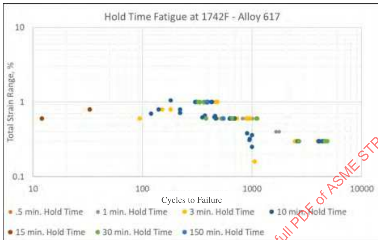
Figure 19-21: Alloy 617 Hold Time Data (Creep Fatigue) For Alloy 617, Temperature of 1742°F
