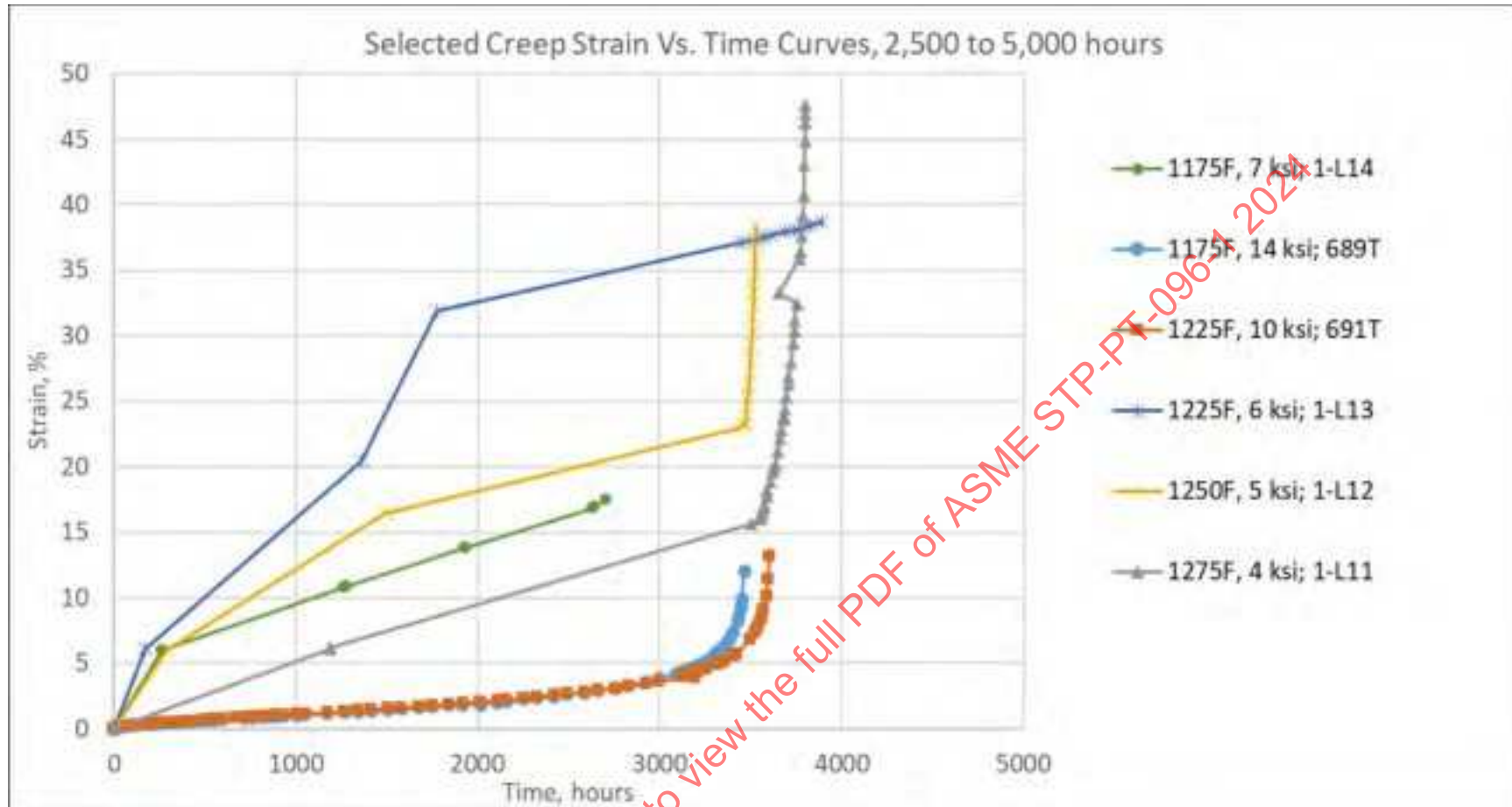
Figure 14-16: Medium-Term Strain Vs. Time Data, 2,500 to 5,000 Hour Test Durations (Grade 9)
