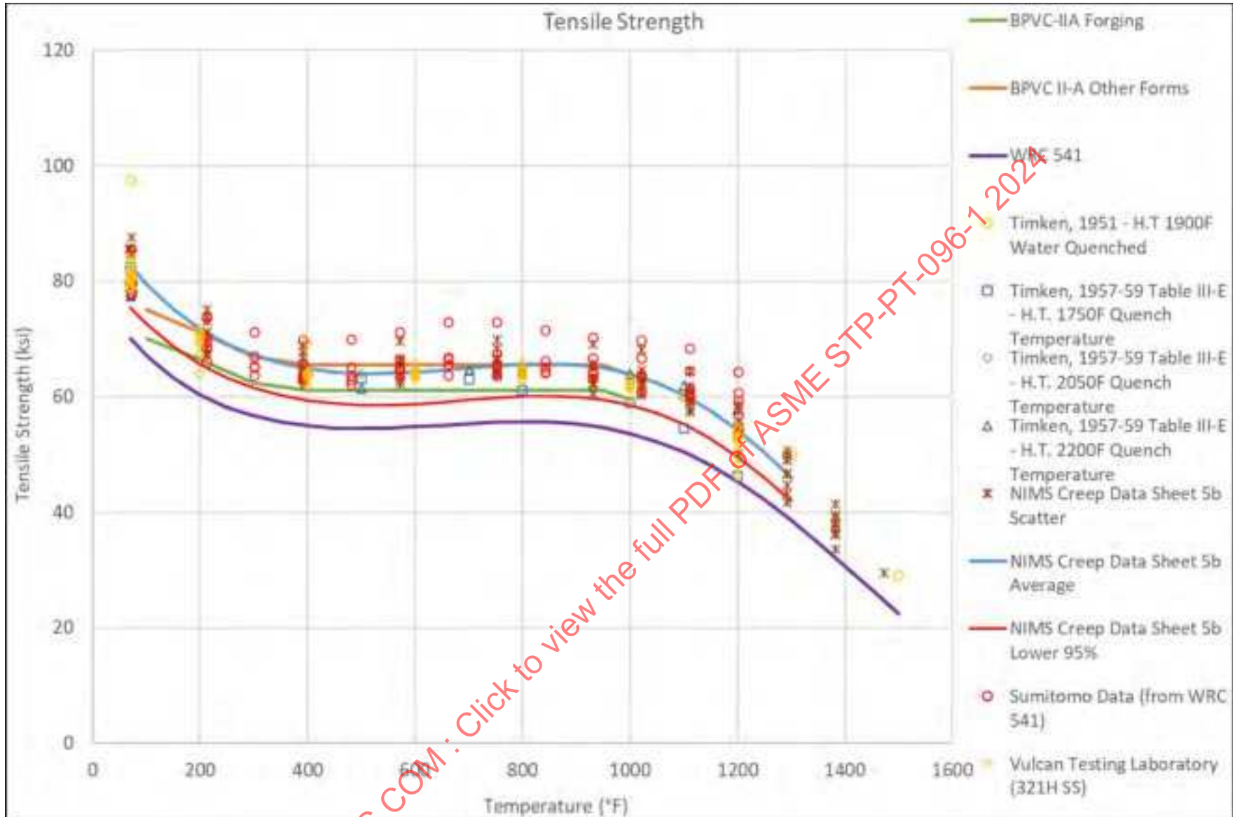
Figure 26-3: 321H Tensile Strength Vs. Temperature, By Data Source, Including Trend Curves
