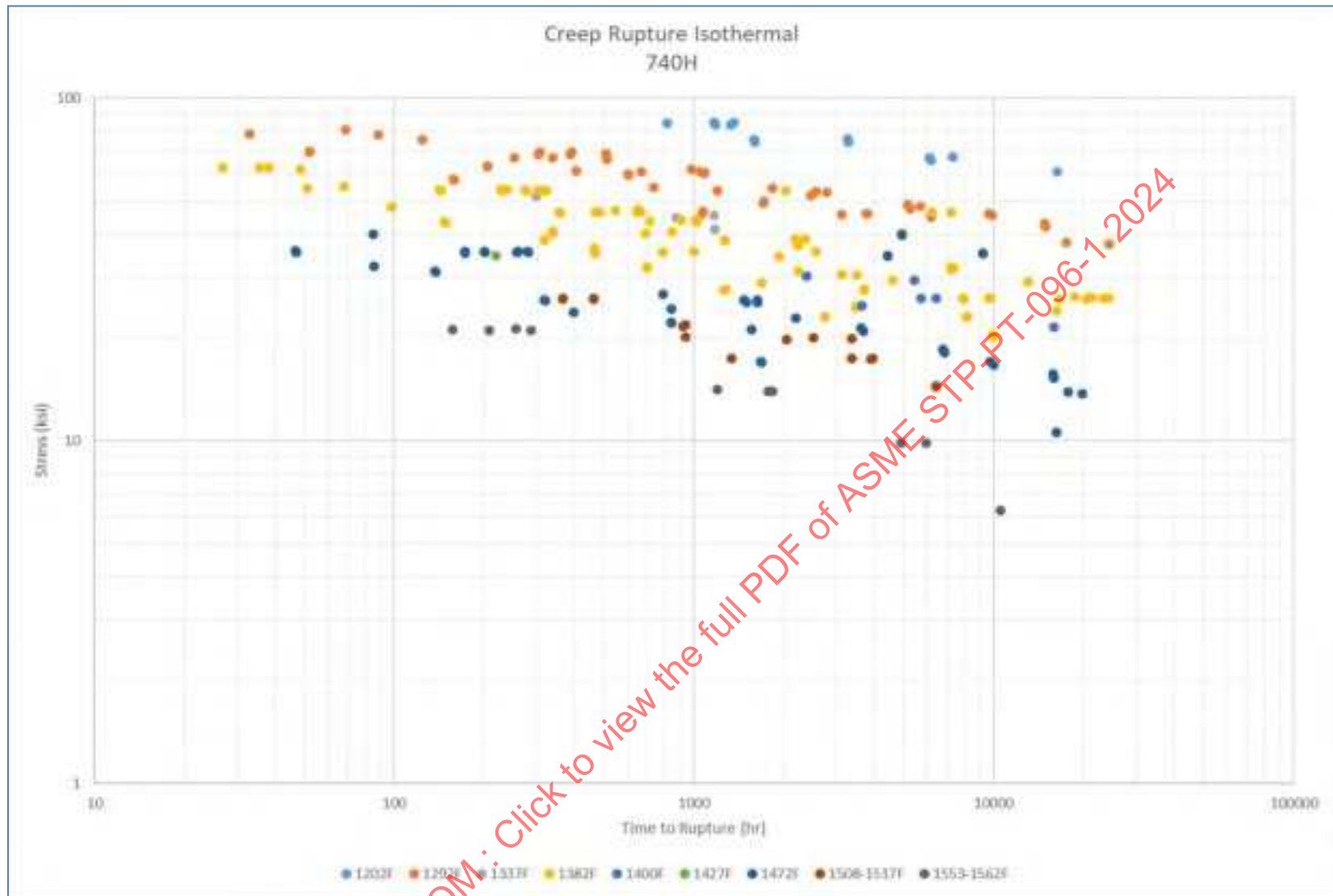
Figure 20-8: 740H Creep Rupture Isotherm Curves
