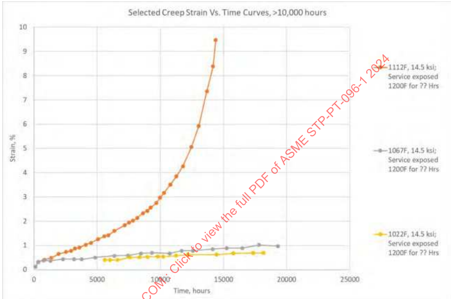
Figure 4-19: Long-Term Strain Vs. Time Data, In Excess of 10,000 Hour Test Durations (Grade 91)
