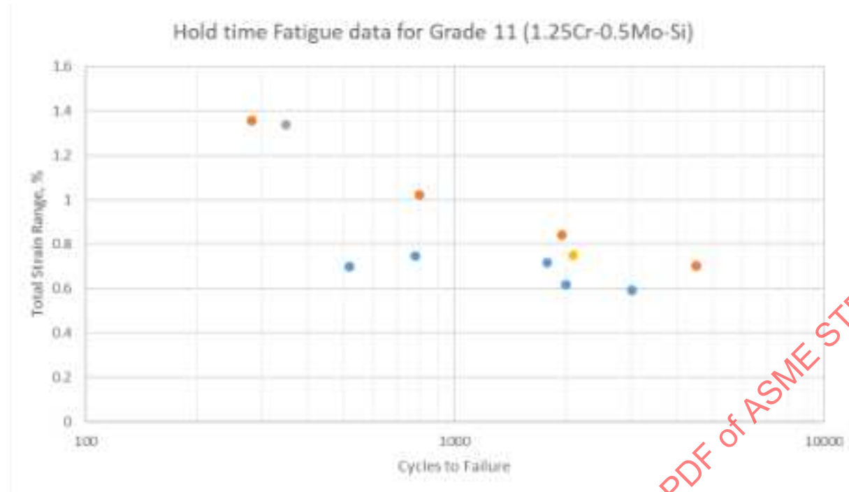
Figure 9-17: Grade 11 Continuous Cycling Fatigue, Including Room Temperature and Elevated Temperature Data
