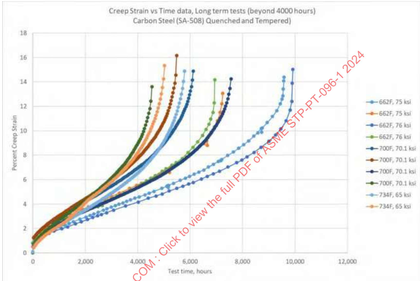
Figure 6-13: Strain Vs. Time Data – CS (SA-508), 1 of 2
