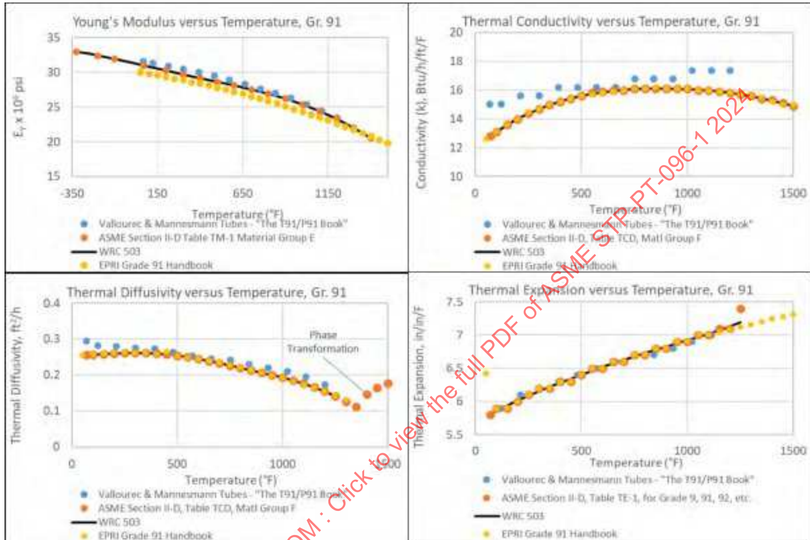
Figure 4-1: Grade 91 Modulus ( E_y ), Thermal Conductivity ( k ), Thermal Diffusivity (TD), & Thermal Expansion ( \alpha ) With Temperature
