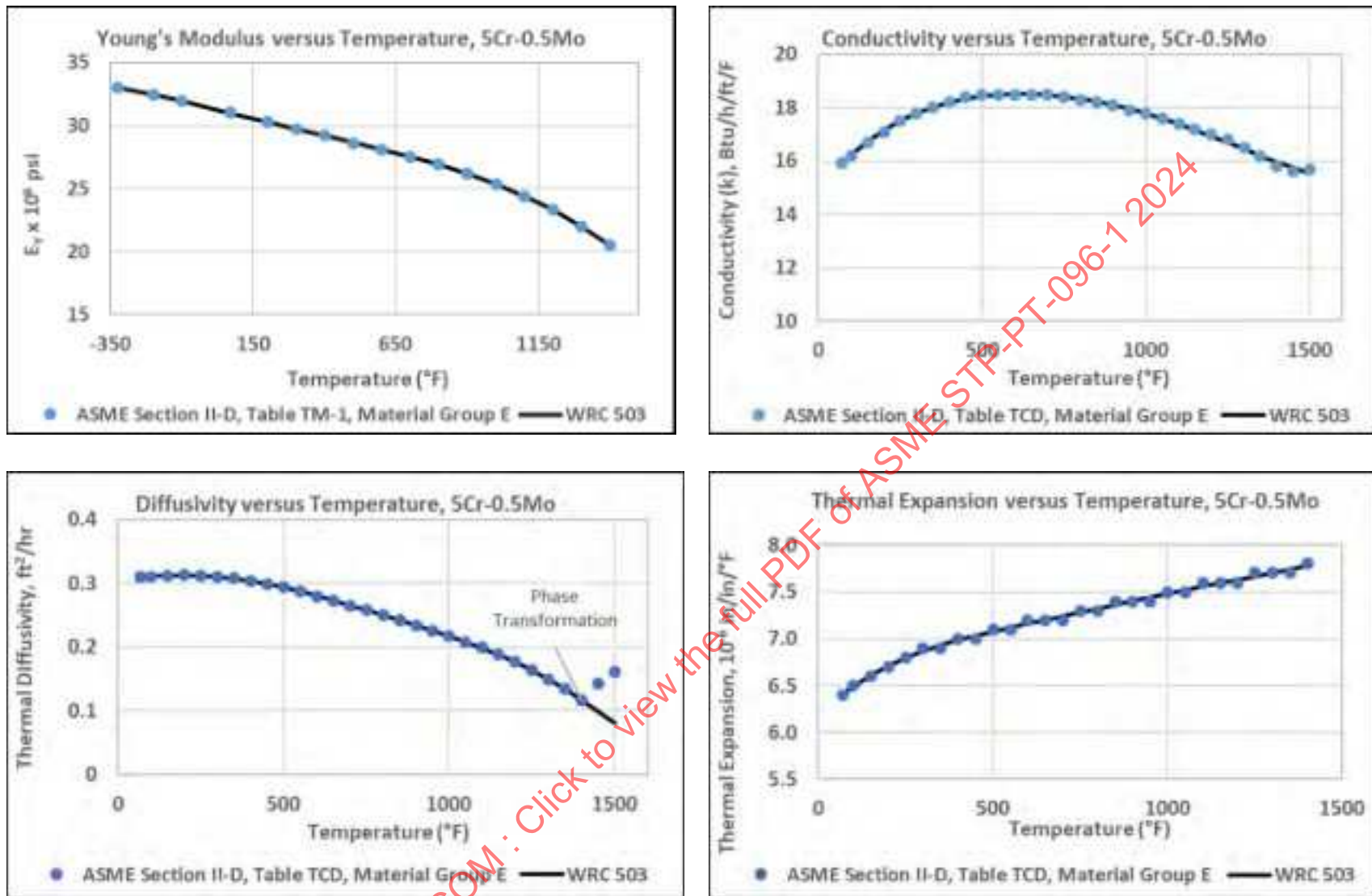
Figure 12-1: Grade 5 Modulus ( E_y ), Thermal Conductivity ( k ), Thermal Diffusivity (TD), & Thermal Expansion ( \alpha ) With Temperature
