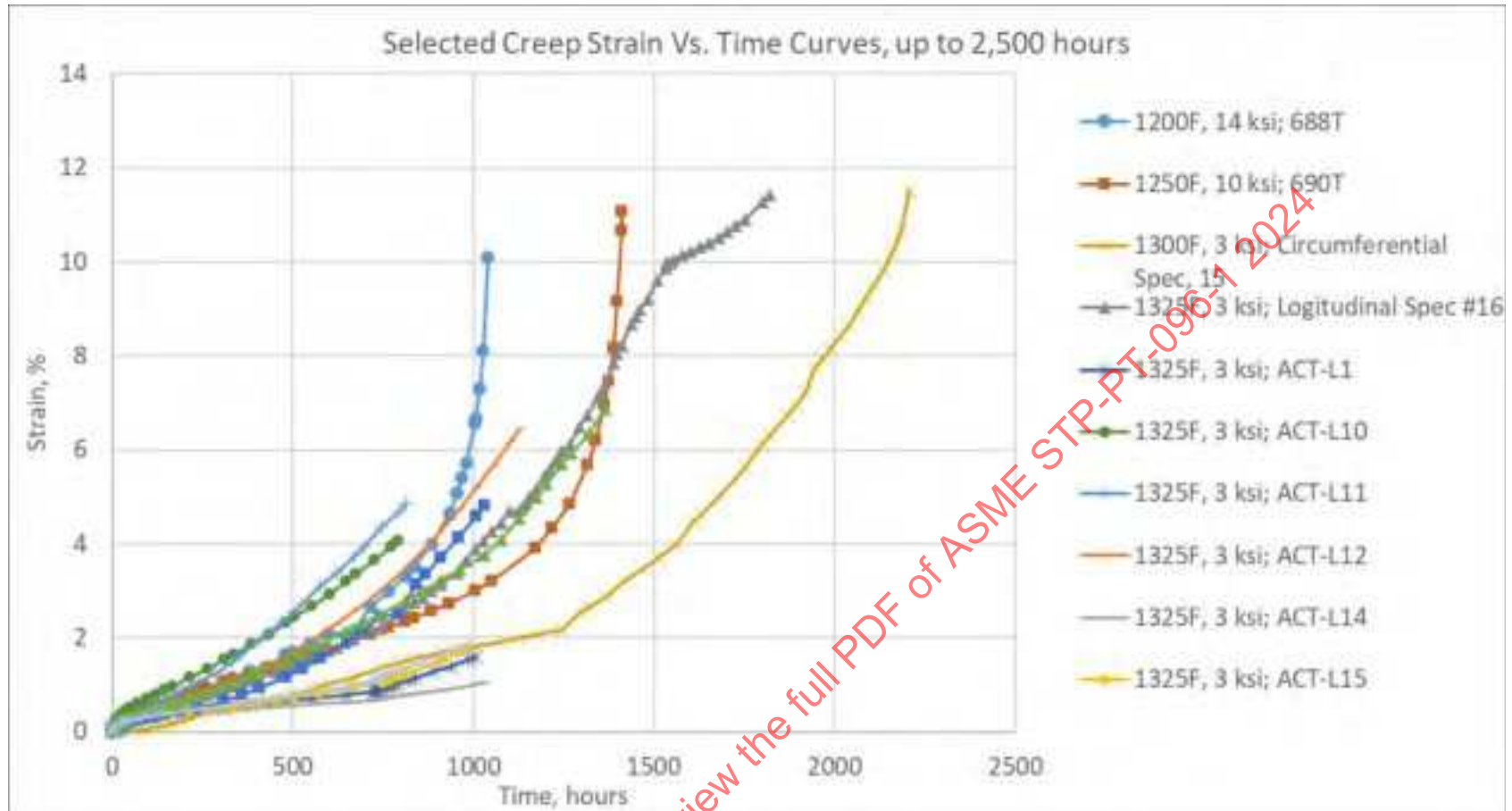
Figure 14-15: Short-Term Strain Vs. Time Data, up to 2,500 Hour Test Durations (Grade 9)
