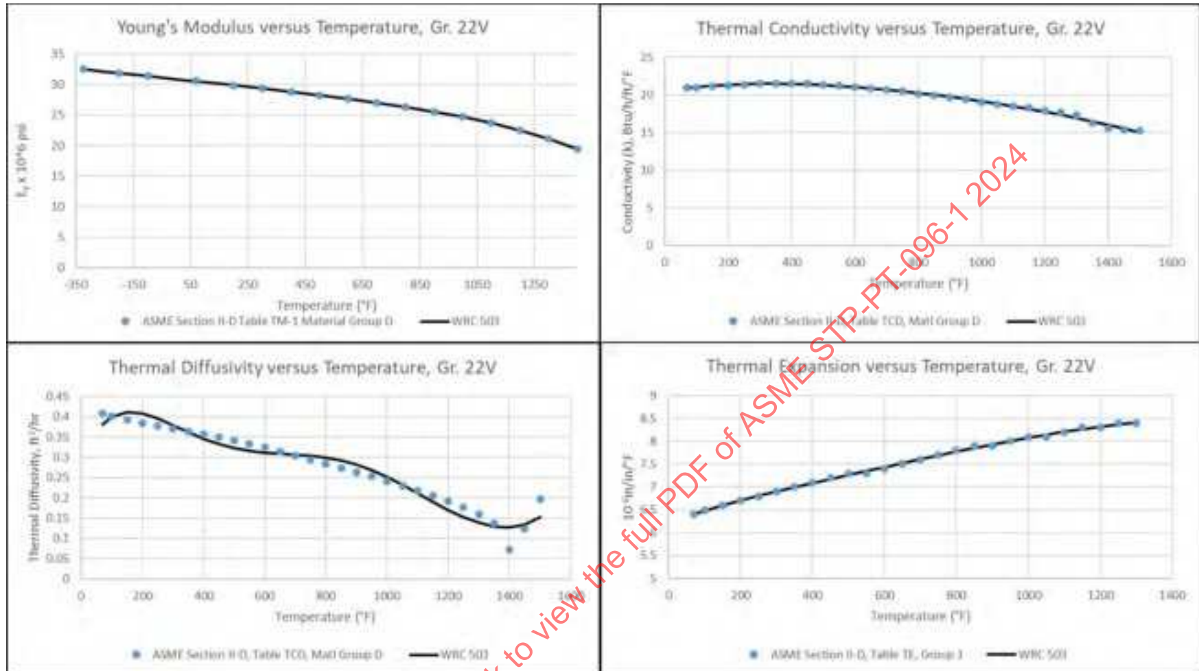
Figure 11-1: Grade 22V Modulus ( E_y ), Thermal Conductivity ( k ), Thermal Diffusivity (TD), & Thermal Expansion ( \alpha ) With Temperature
