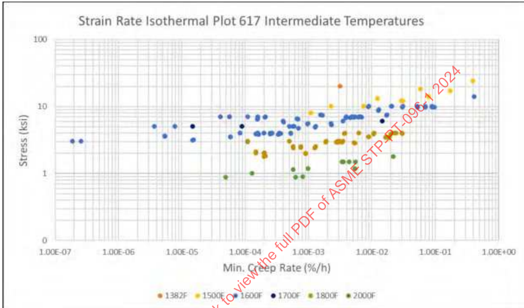
Figure 19-11: Alloy 617 Creep Strain Rate (MCR) Isotherm Curves, Intermediate Temperatures
