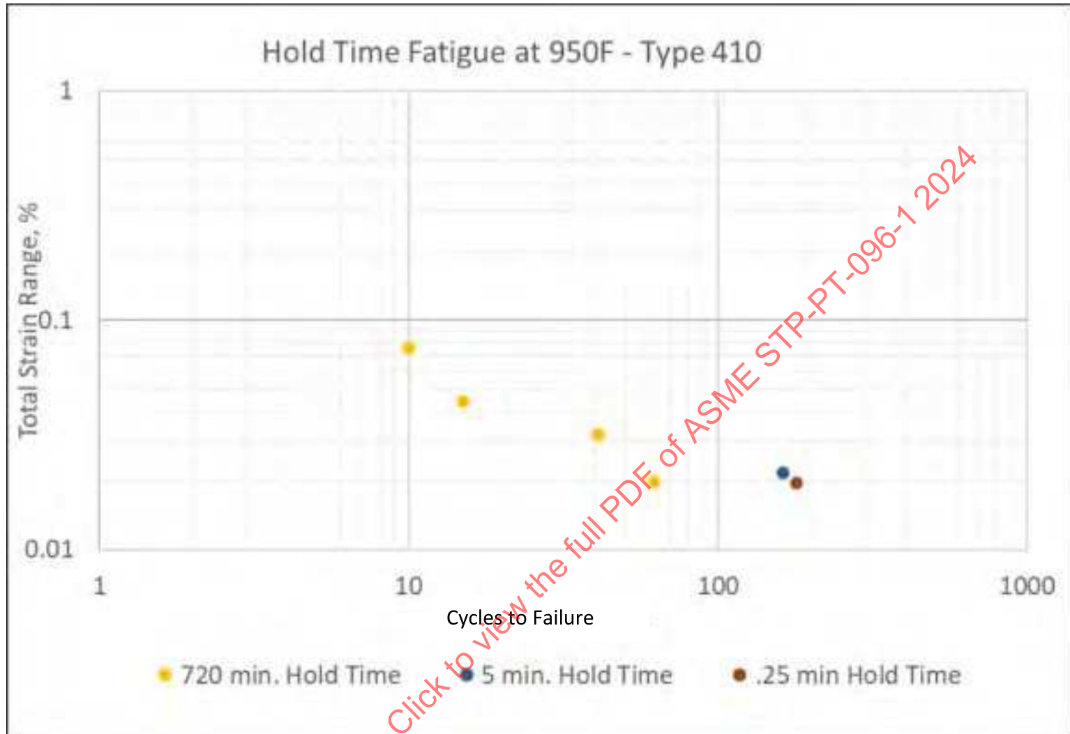
Figure 25-23: Type 410/12Cr Hold Time Data (Creep Fatigue) for Type 410/12Cr, Temperature of 950°F
