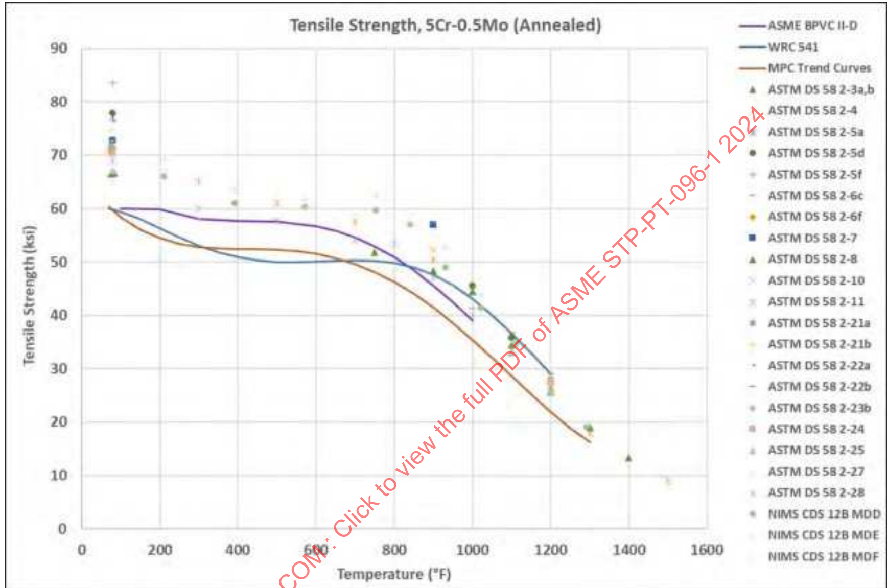
Figure 12-3: Grade 5 (Annealed) Strength Vs. Temperature, By Data Source, Including Trend Curves
