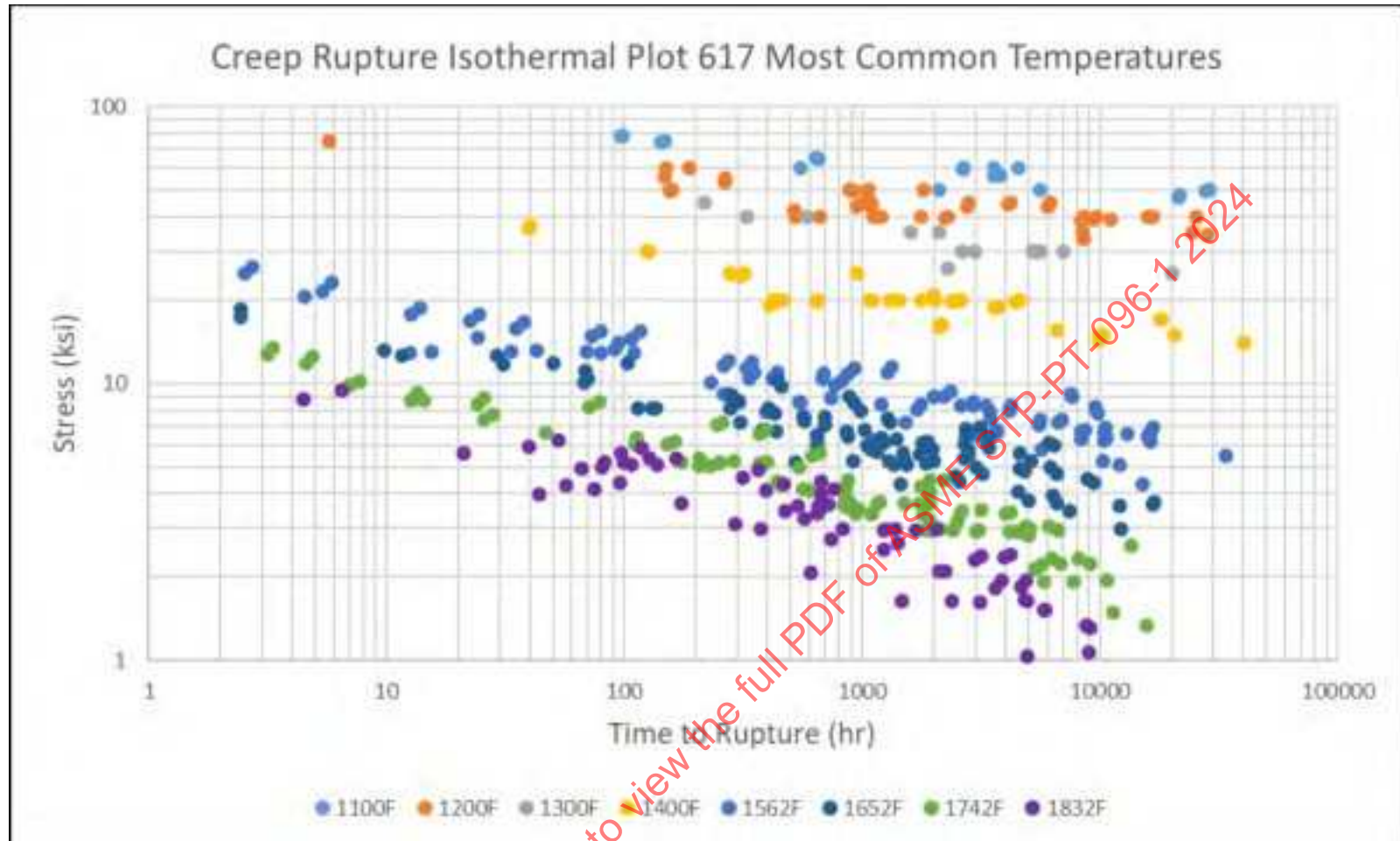
Figure 19-8: Alloy 617 Creep Rupture Isotherm Curves, Most Common Temperatures
