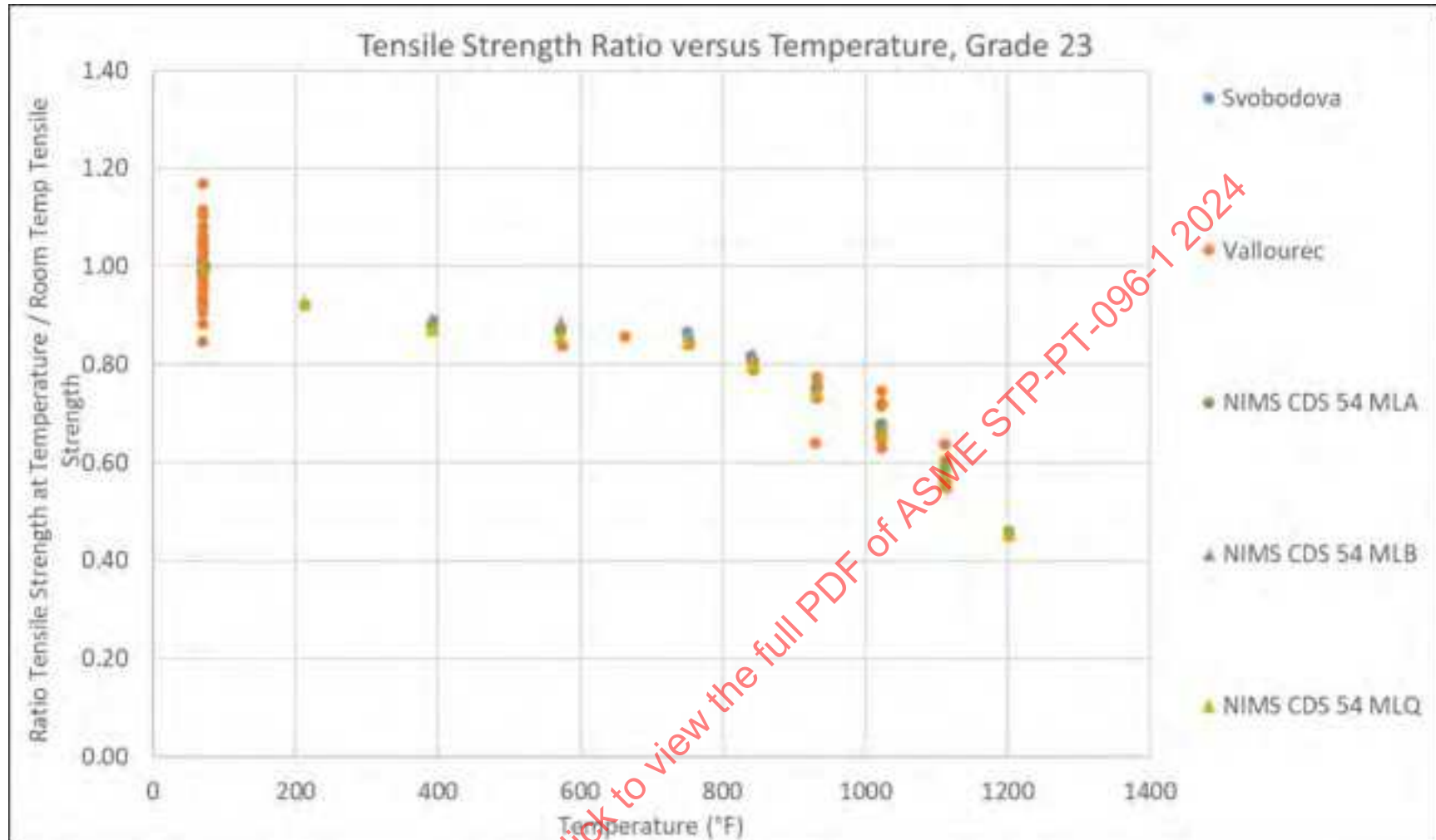
Figure 23-5: Grade 23 Tensile Strength Ratios Vs. Temperature (Calculated on a Heat-By-Heat Basis, By Data Source)
