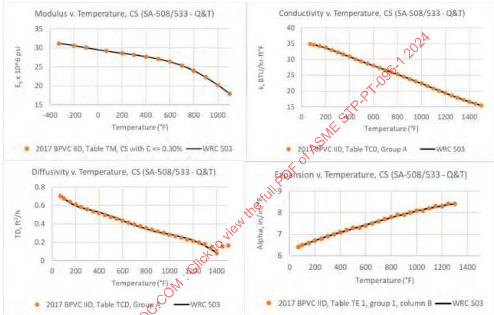
Figure 6-1: CS (SA-508 & SA-533) Modulus ( E_y ), Thermal Conductivity ( k ), Thermal Diffusivity (TD), & Thermal Expansion ( \alpha ) With Temperature
