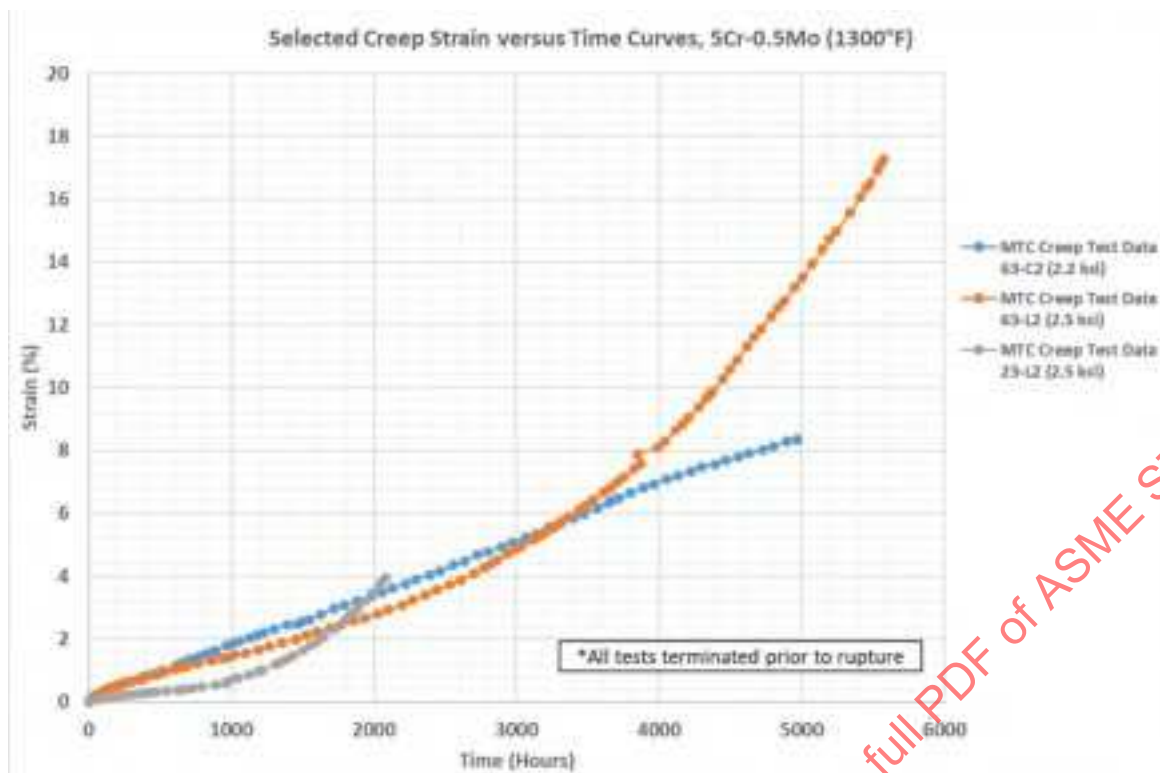
Figure 12-20: Selected Strain Vs. Time Data (Grade 5 at 1300°F), All Tests Terminated Prior to Rupture
