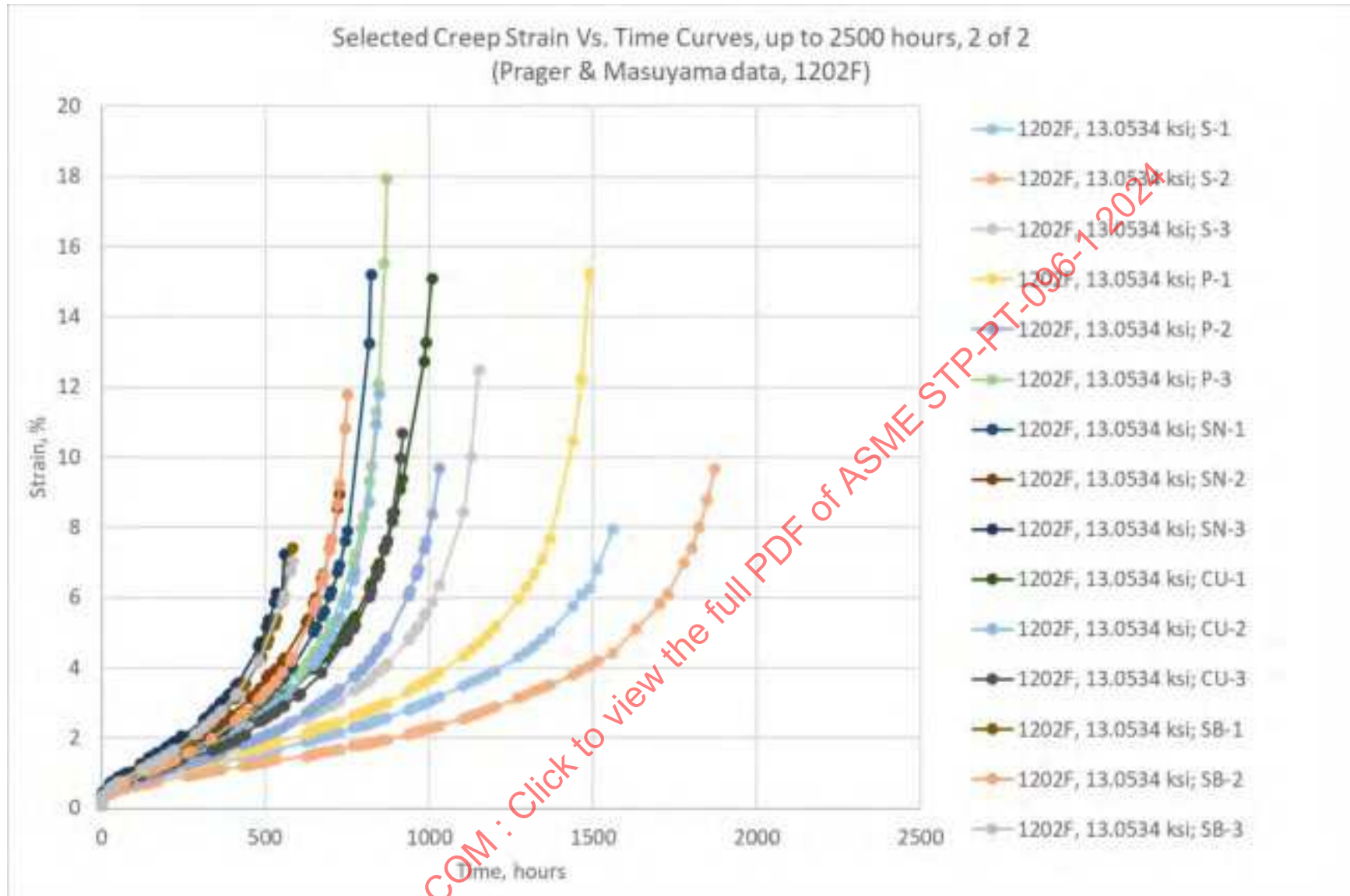
Figure 4-16: Short-Term Strain Vs. Time Data, Up to 2,500 Hour Test Durations (Grade 91), 2 of 2
