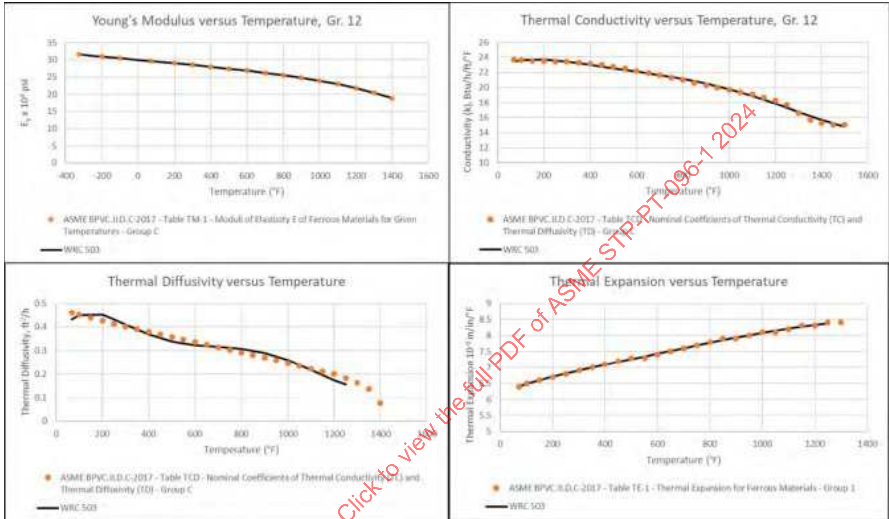
Figure 22-1: Grade 12 Modulus ( E_y ), Thermal Conductivity ( k ), Thermal Diffusivity (TD), & Thermal Expansion ( \alpha ) With Temperature
