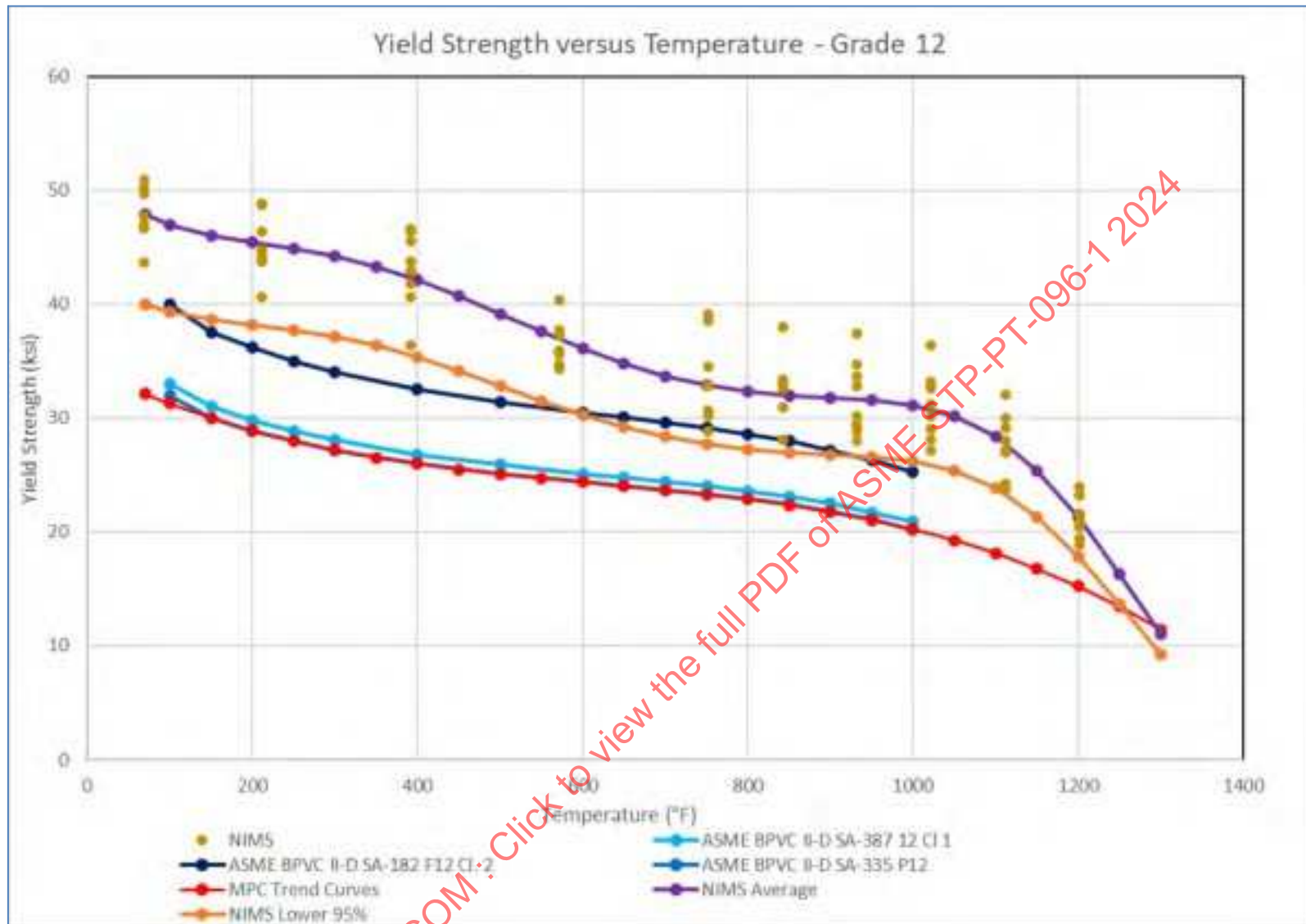
Figure 22-2: Grade 12 Yield Strength Vs. Temperature, By Data Source, Including Trend Curves
