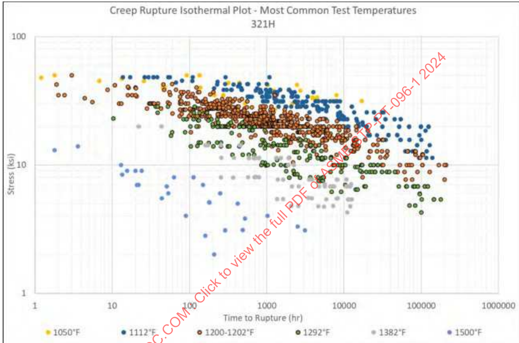
Figure 26-8: 321H Creep Rupture Isotherm Curves, Temperatures With High Concentration of Data Points
