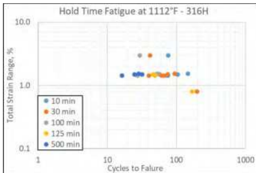
Figure 17-21: Hold Time Data (Creep Fatigue) for 316H, Temperature of 1112°F
