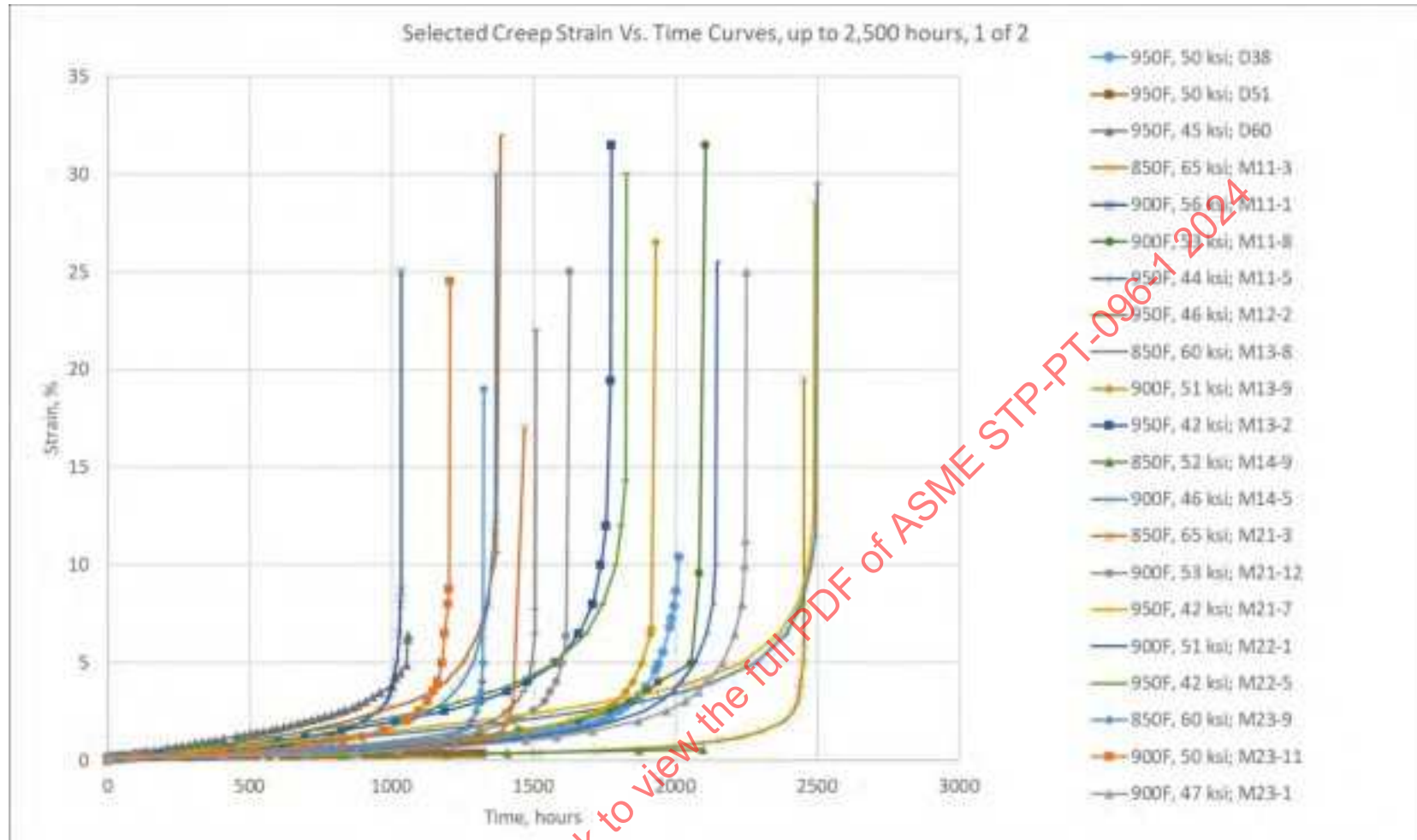
Figure 11-16: Medium-Term Strain Vs. Time Data, 1,000 to 2,500 Hour Test Durations (Grade 22V), 1 of 2
