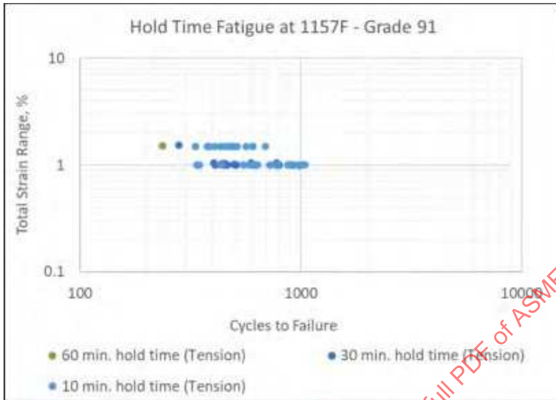
Figure 4-24: Grade 91 Hold Time Data (Creep Fatigue) For Grade 91, Temperature of 1157°F
