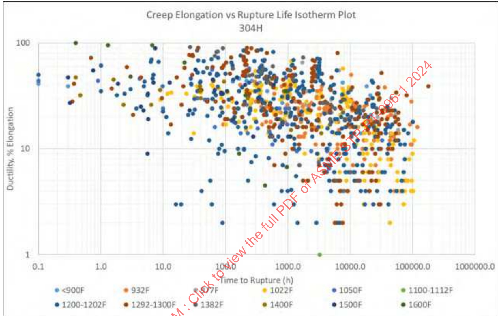
Figure 16-11: 304H Creep Ductility (% Elongation) Vs. Rupture Time Isotherms
