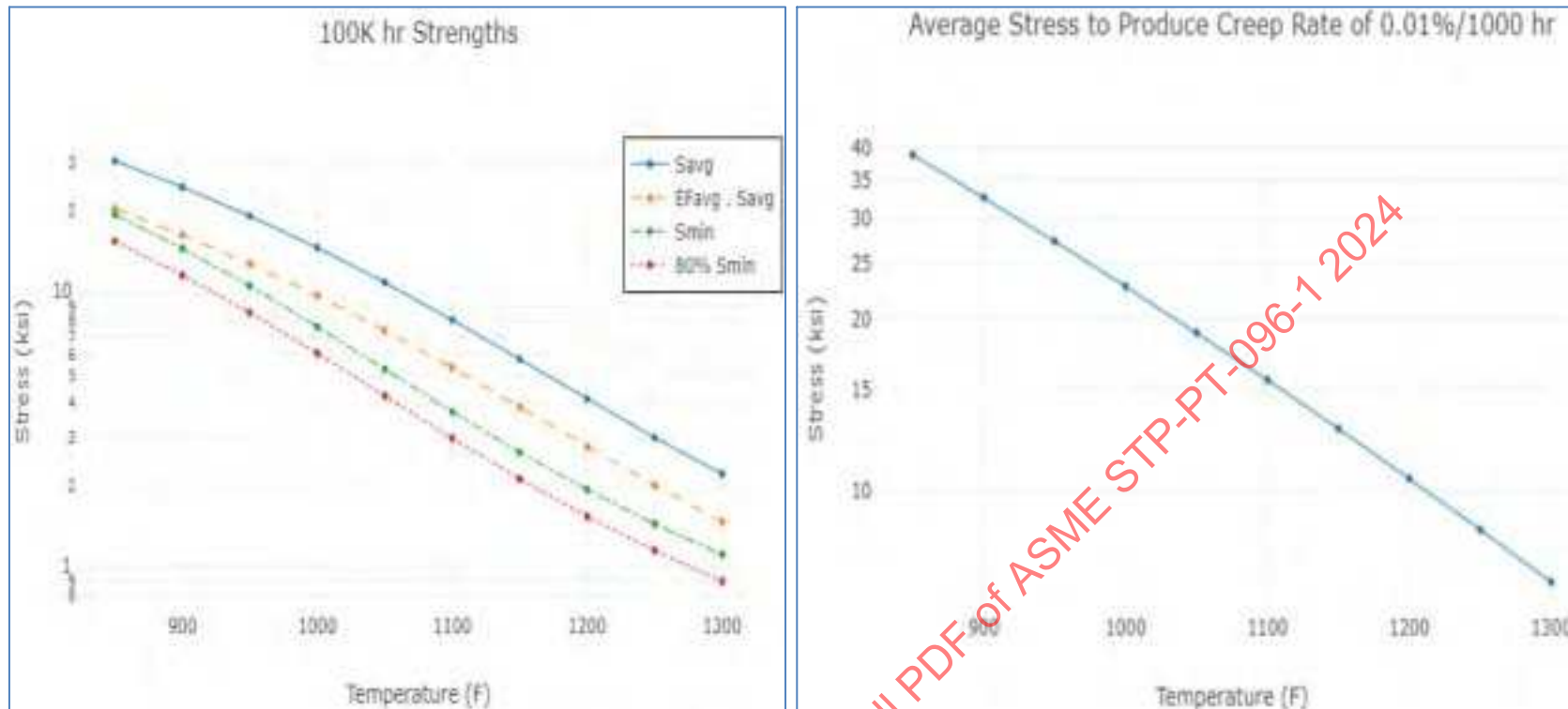
Figure 16-12: Calculated Allowable Stresses Based on Rupture and Creep Strain Rate and ASME II-D Appendix 1 Criteria (304H)
