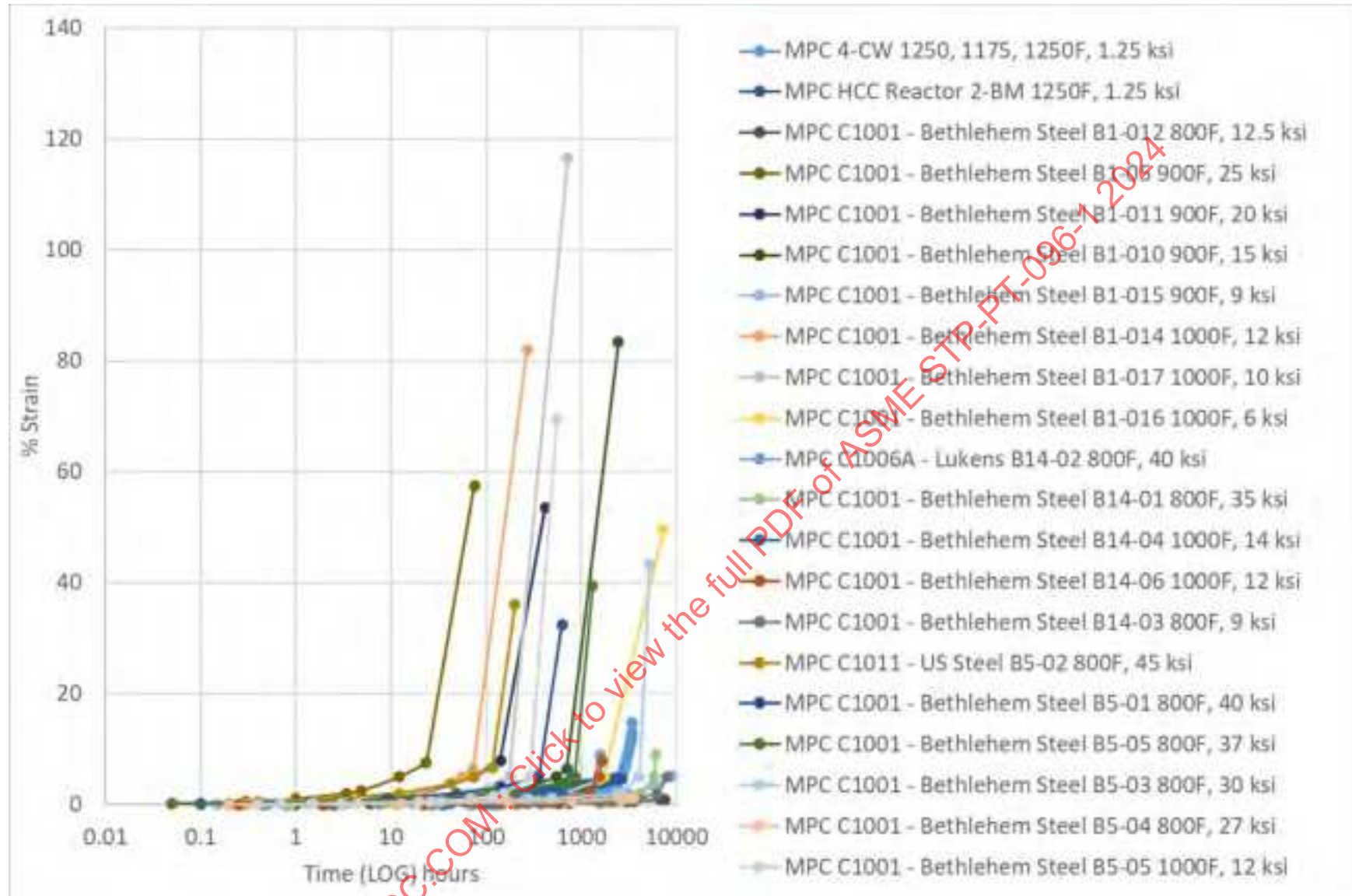
Figure 5-22: Strain Vs. Time Data, up to 2,500 Hour Test Durations – CS (516/299), 7 of 7
