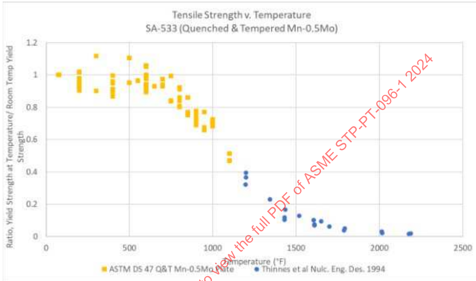
Figure 7-4: SA-533 (Q&T Mn-0.5Mo) Tensile Strength Ratios Vs. Temperature (Calculated on a Heat-By-Heat Basis, By Data Source)
