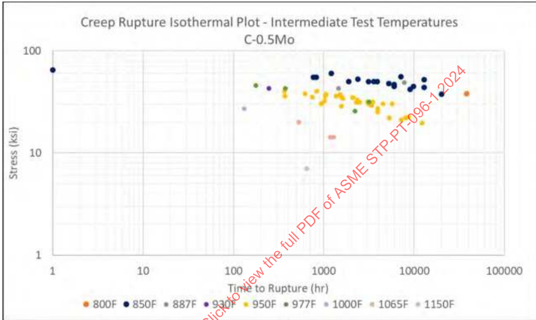
Figure 8-9: C-1/2Mo Creep Rupture Isotherm Curves for Additional and Intermediate Temperatures
