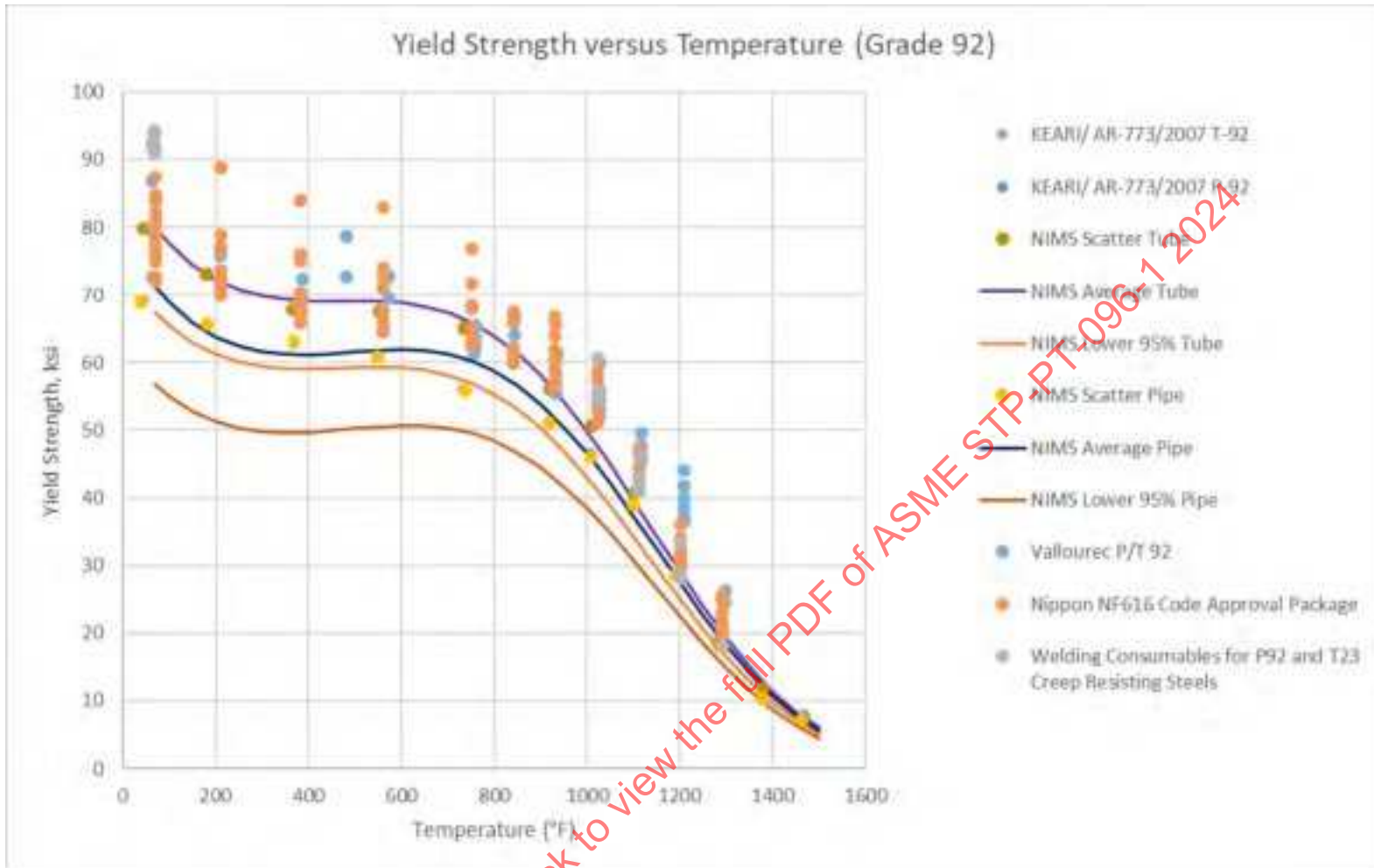
Figure 15-2: Grade 92 Yield Strength Vs. Temperature, By Data Source, Including Trend Curves
