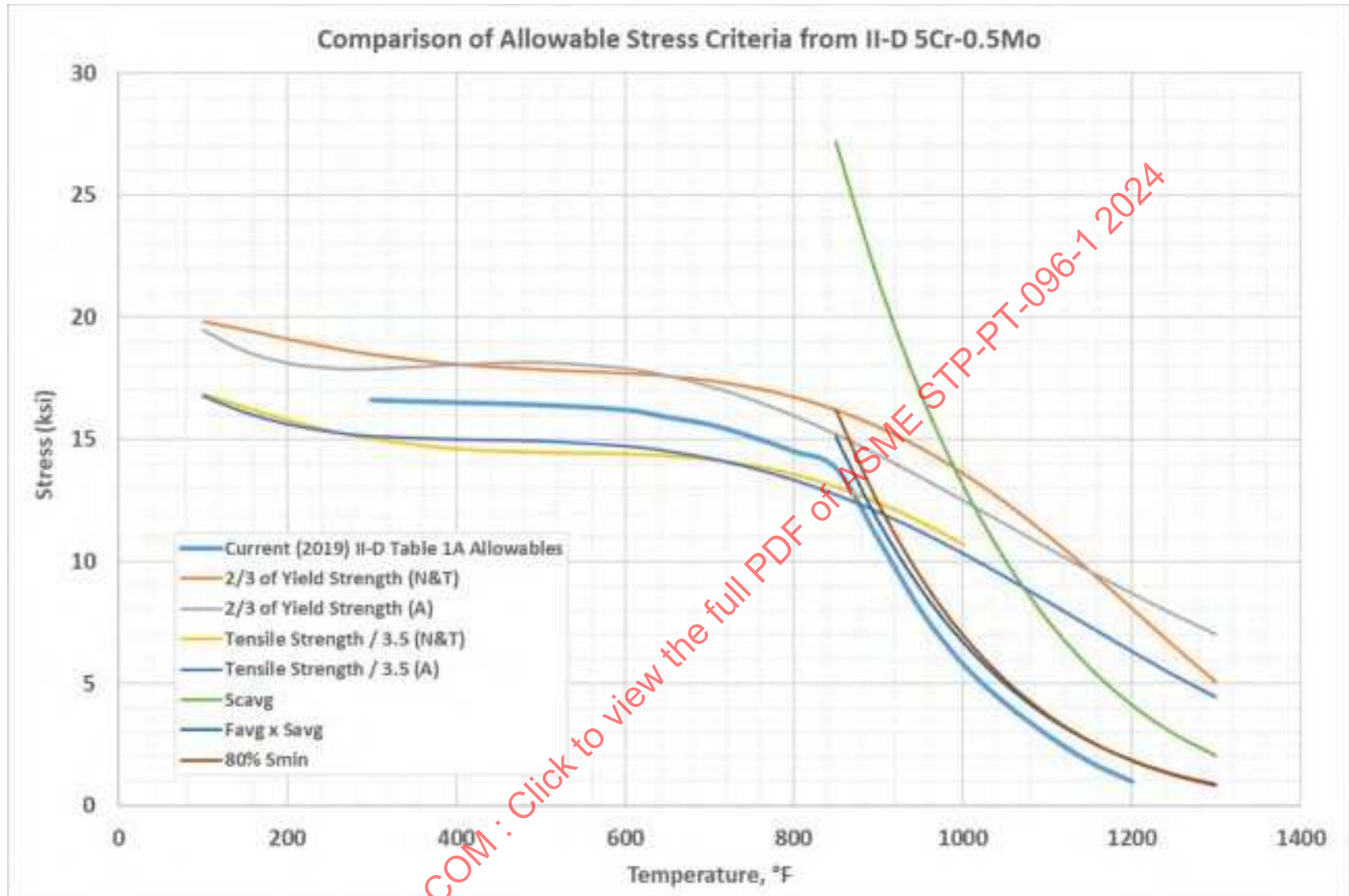
Figure 12-19: Comparison of Current Grade 5 Allowable Stresses Vs. ASME II-D Appendix 1 Criteria Applied to Data
