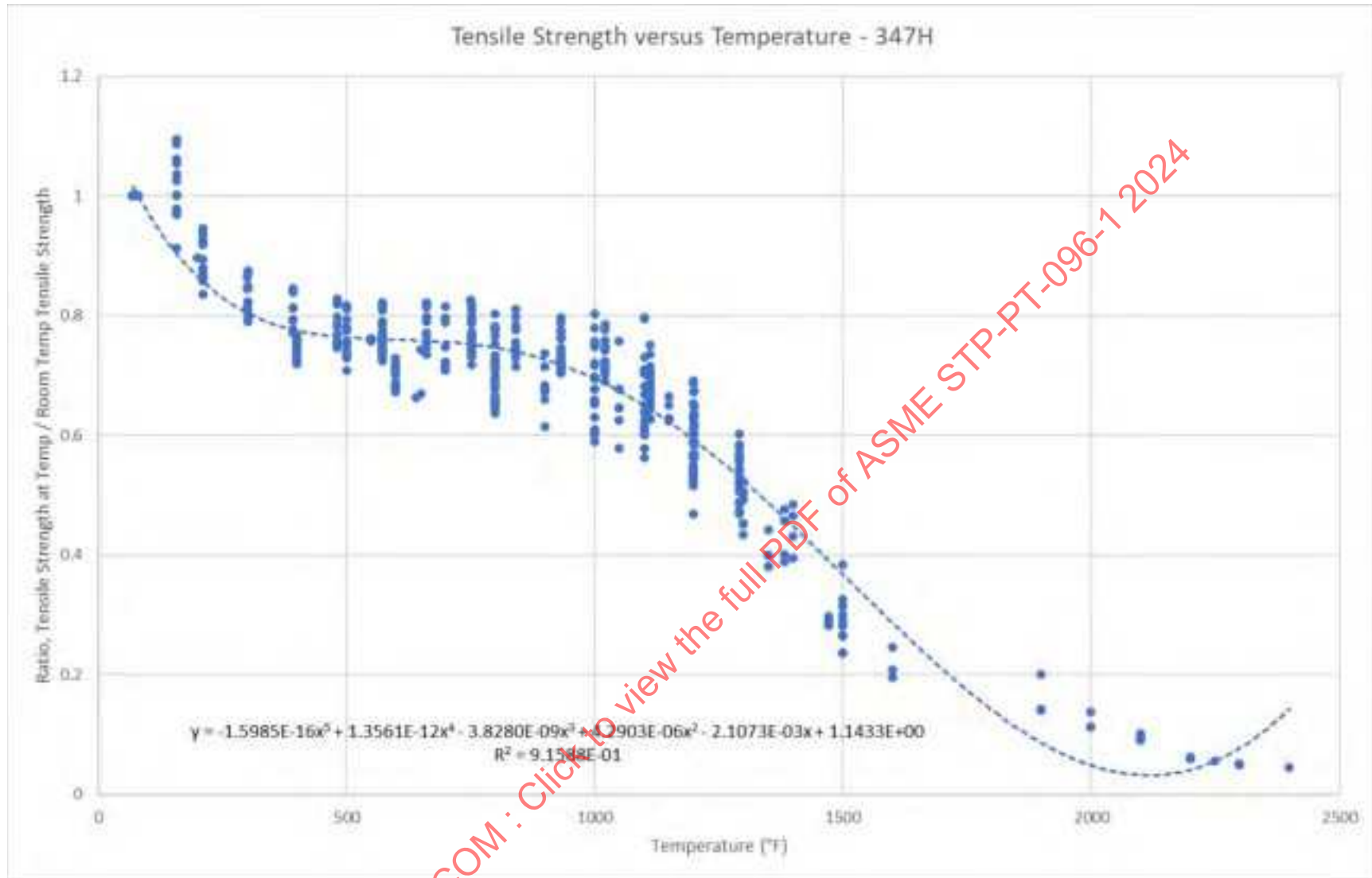
Figure 18-7: 347H Tensile Strength Ratios Vs. Temperature, All Combined Data, With Polynomial Regression
