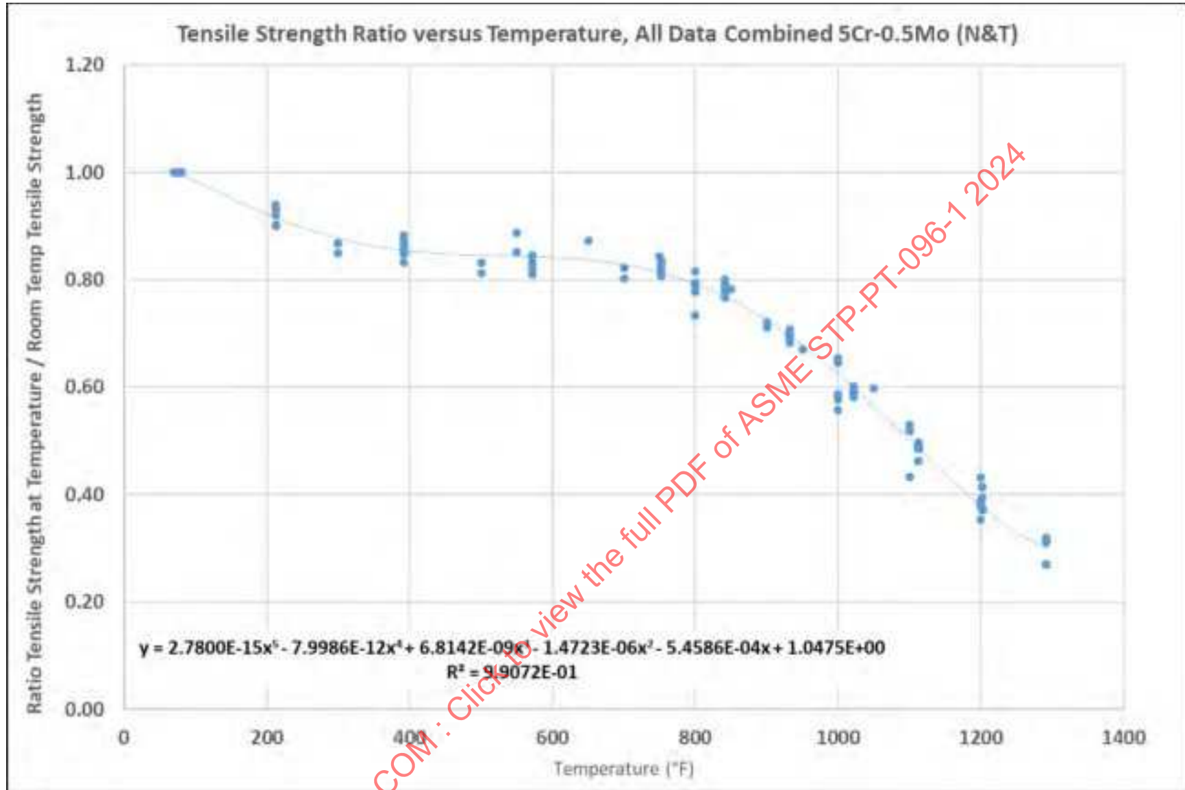
Figure 12-13: Grade 5 (N&T) Tensile Strength Ratios Vs. Temperature, All Combined Data, With Polynomial Regression
