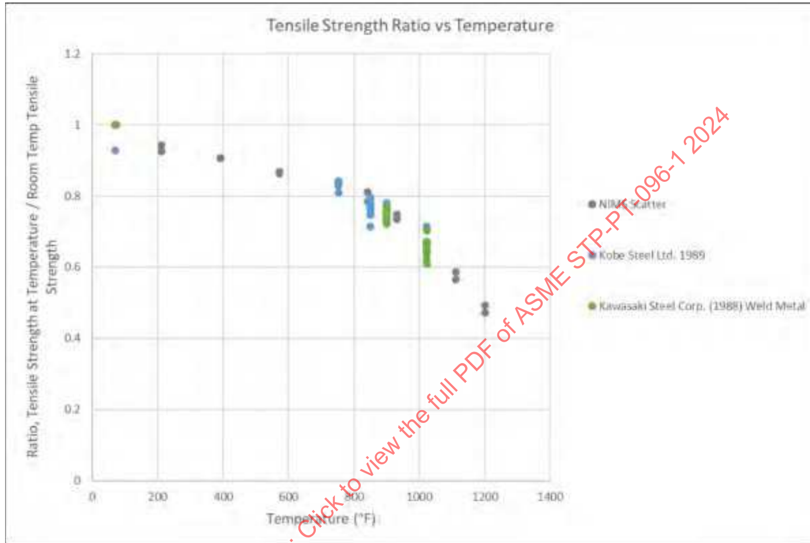
Figure 11-5: Grade 22V Tensile Strength Ratios Vs. Temperature (Calculated on a Heat-By-Heat Basis, By Data Source)
