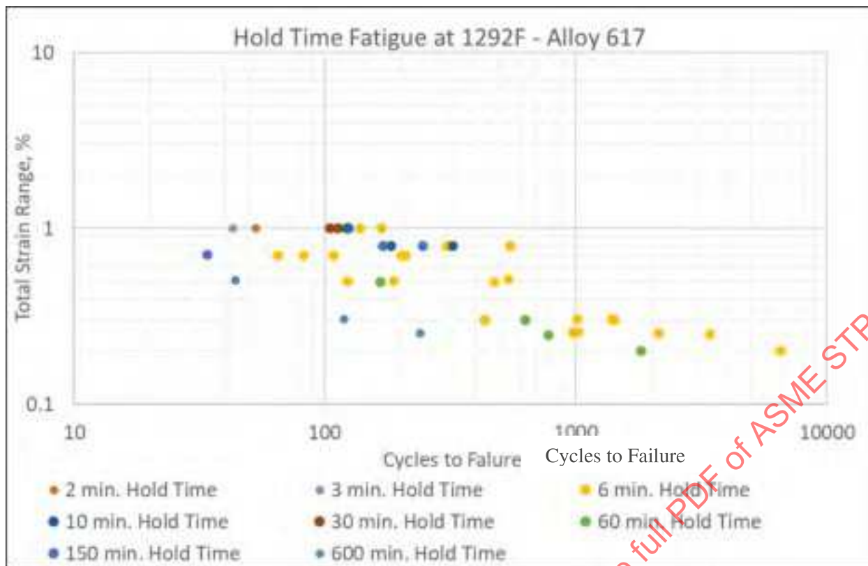
Figure 19-19: Alloy 617 Hold Time Data (Creep Fatigue) for Alloy 617, Temperature of 1292°F
