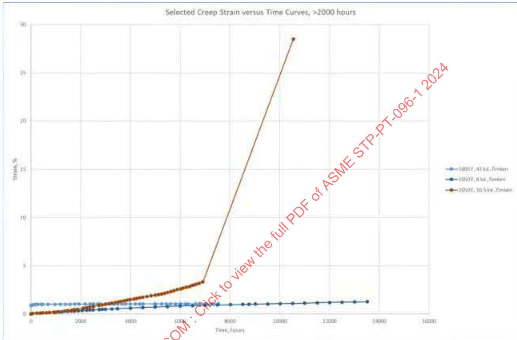
Figure 18-16: Creep Strain Vs. Data, in Excess of 2,000 Hour Test Durations (374H)
