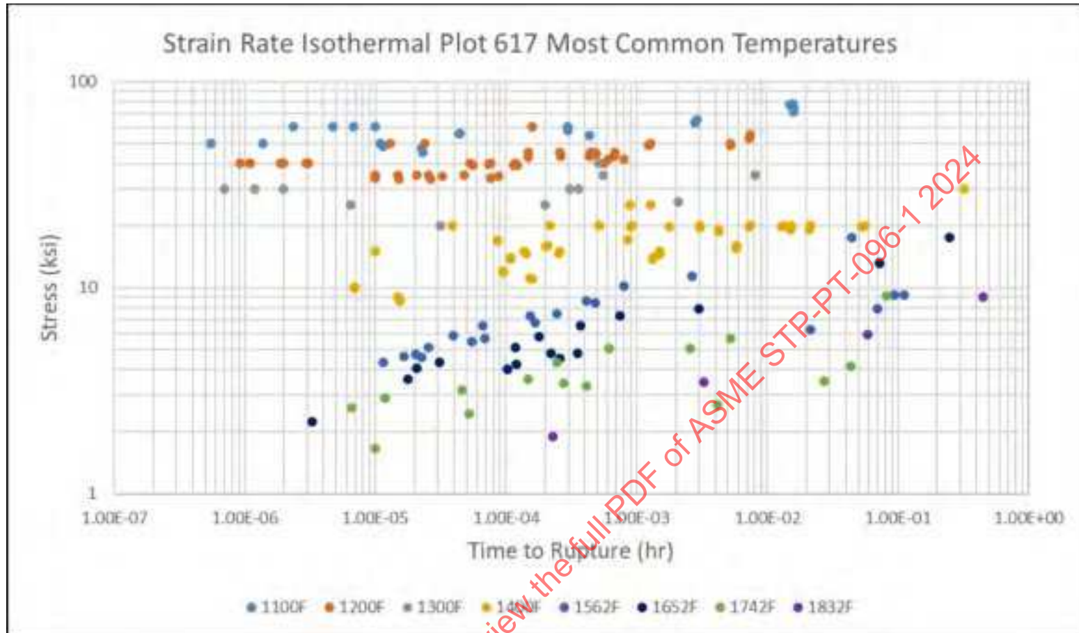
Figure 19-10: Alloy 617 Creep Strain Rate (MCR) Isotherm Curves, Most Common Temperatures
