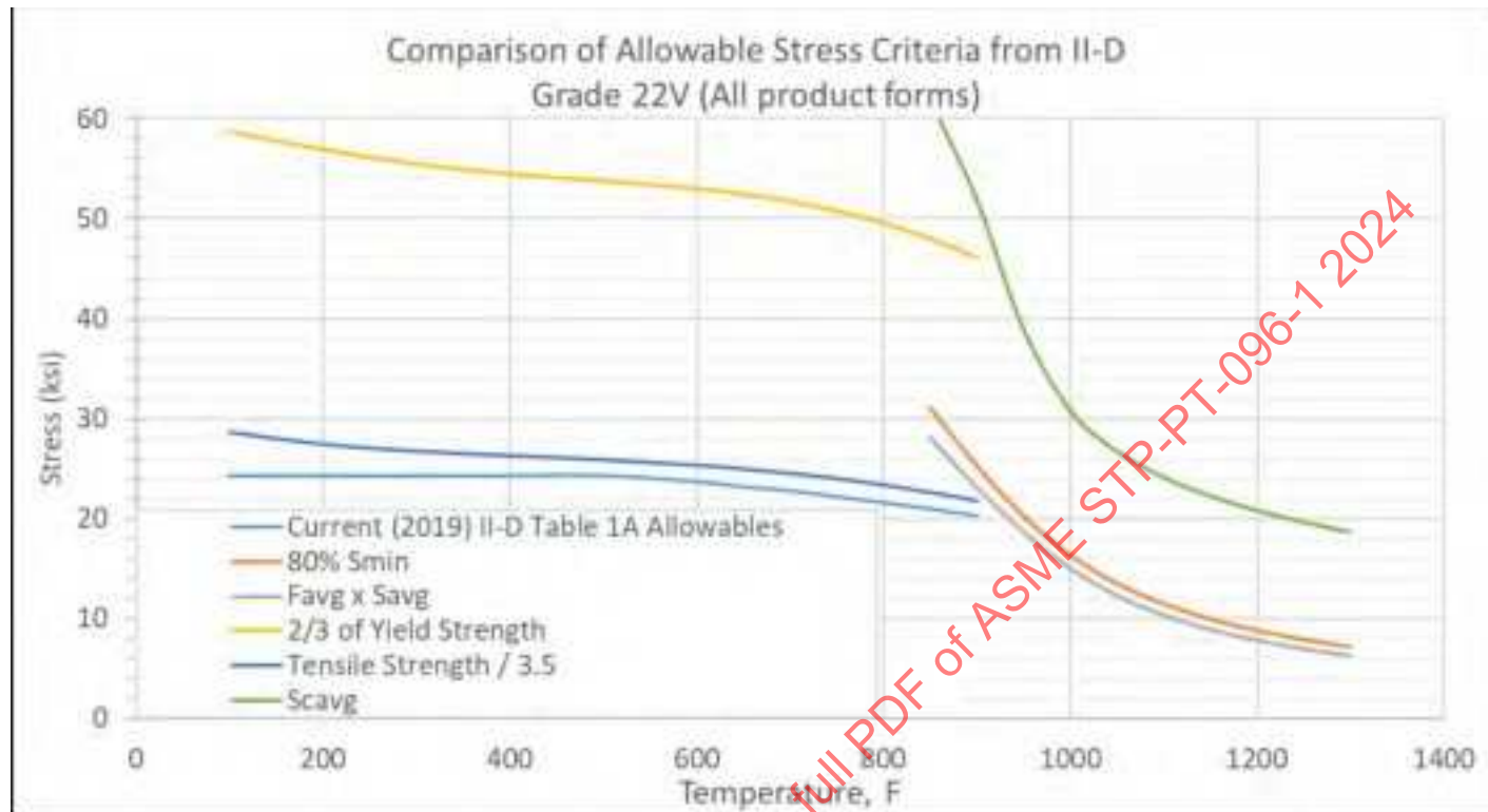
Figure 11-13: Comparison of Current Grade 22V Allowable Stresses (All Product Forms) Vs. ASME II-D Appendix 1 Criteria Applied to Data
