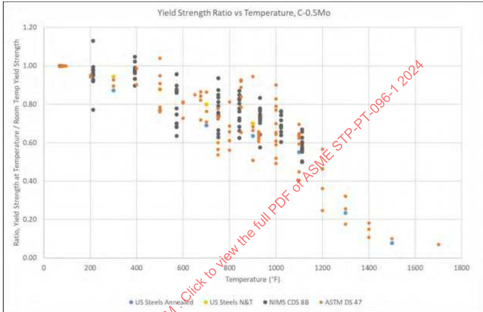
Figure 8-4: C-1/2Mo Yield Strength Ratios Vs. Temperature (Calculated on a Heat-By-Heat Basis, By Data Source)
