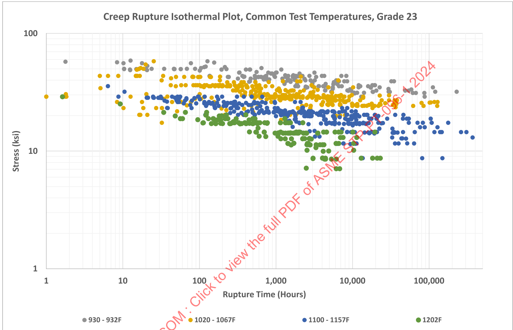
Figure 23-8: Grade 23 Creep Rupture Isotherm Curves
