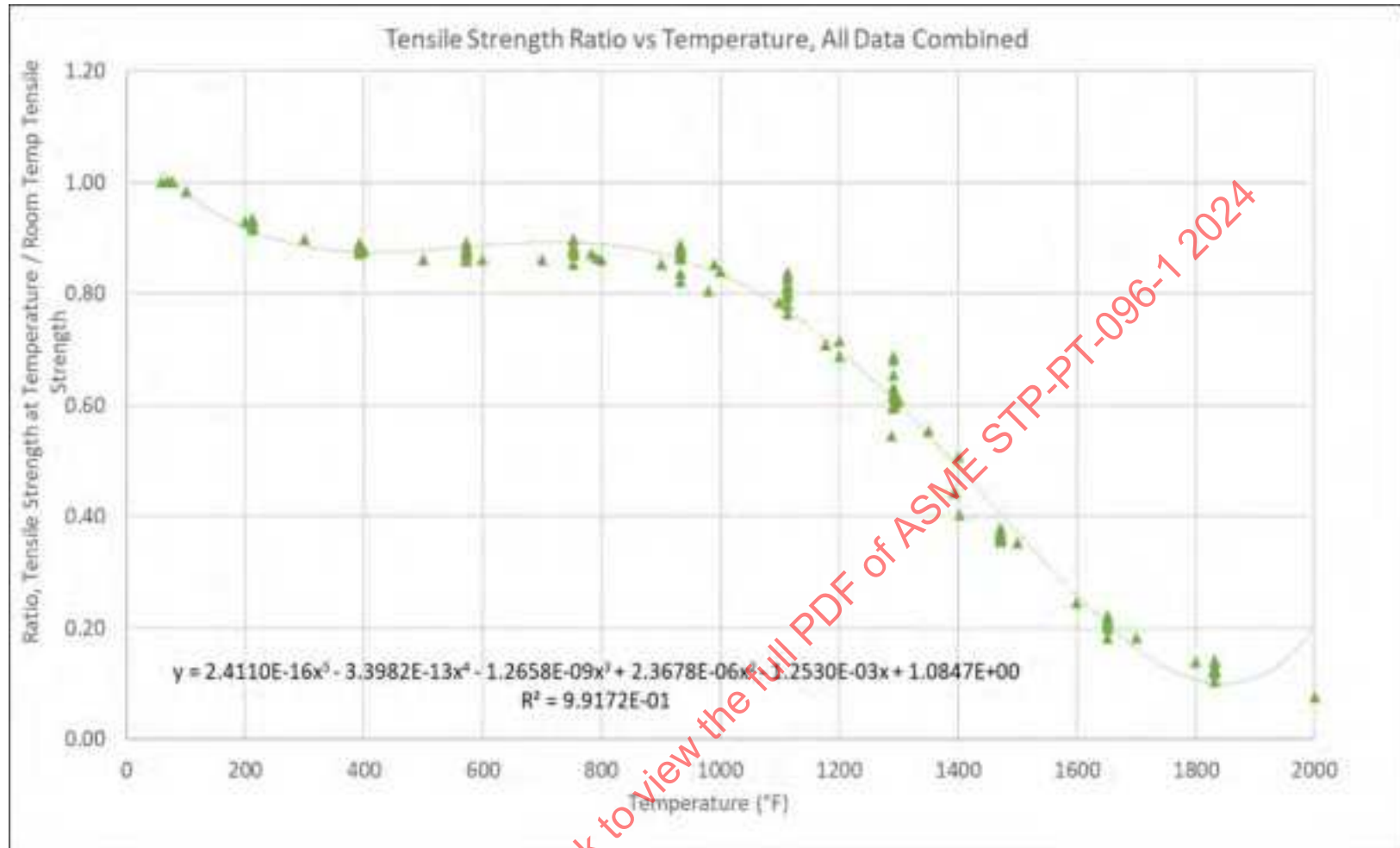
Figure 21-7: Alloy 800H Tensile Strength Ratios Vs. Temperature, All Combined Data, With Polynomial Regression
