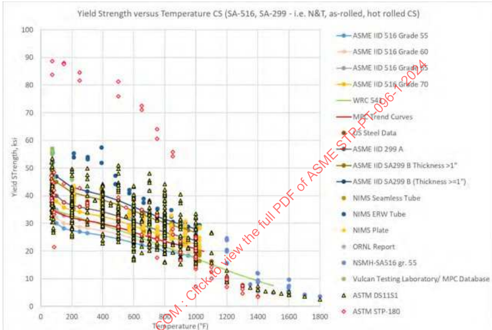
Figure 5-2: CS (516/299) Yield Strength Vs. Temperature, By Data Source, Including Trend Curves
