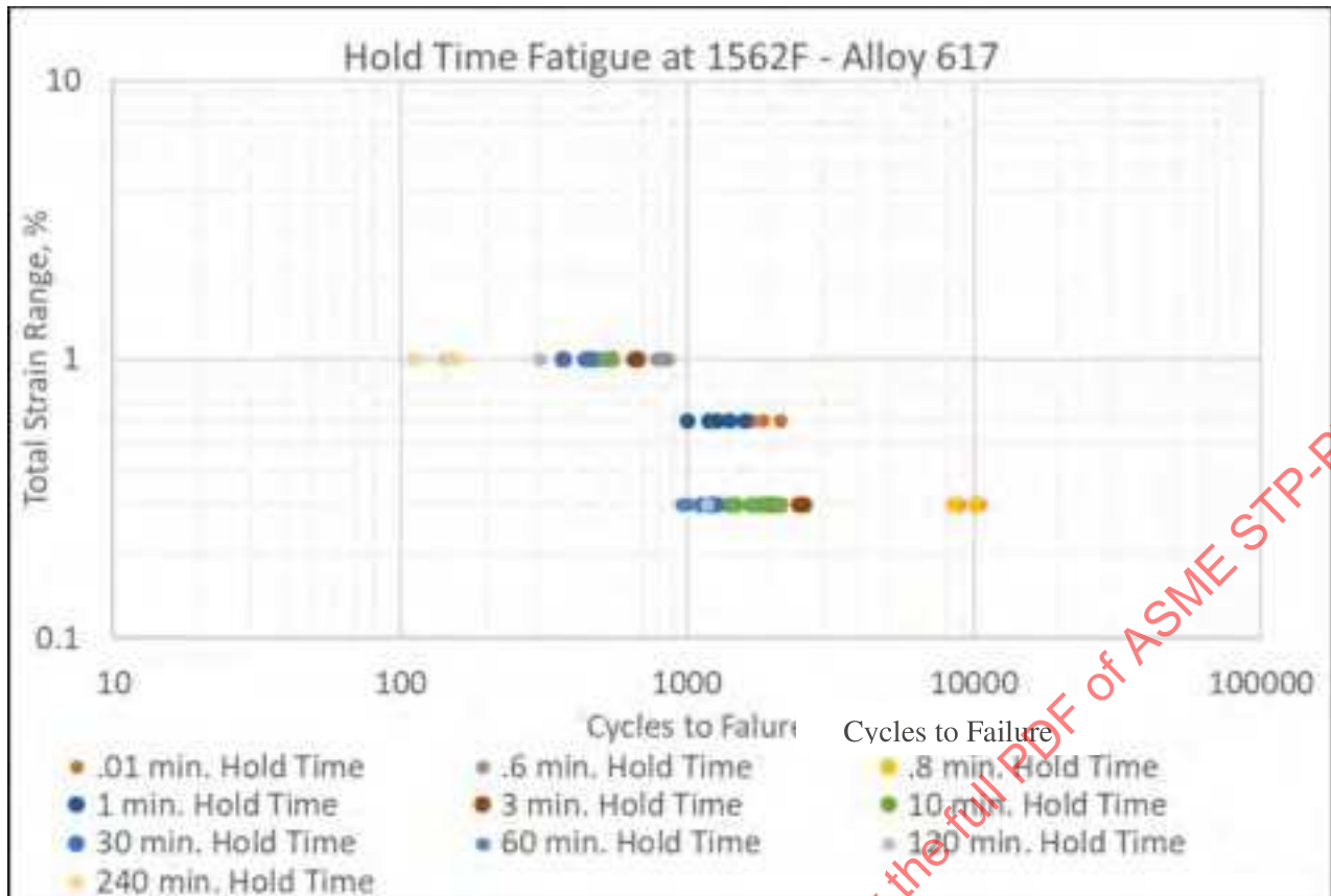
Figure 19-20: Alloy 617 Hold Time Data (Creep Fatigue) for Alloy 617, Temperature of 1562°F
