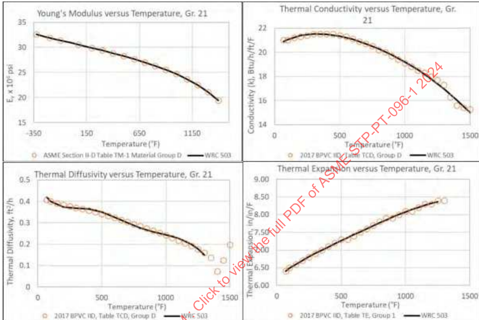
Figure 24-1: 3Cr Modulus ( E_y ), Thermal Conductivity ( k ), Thermal Diffusivity (TD), & Thermal Expansion ( \alpha ) With Temperature
