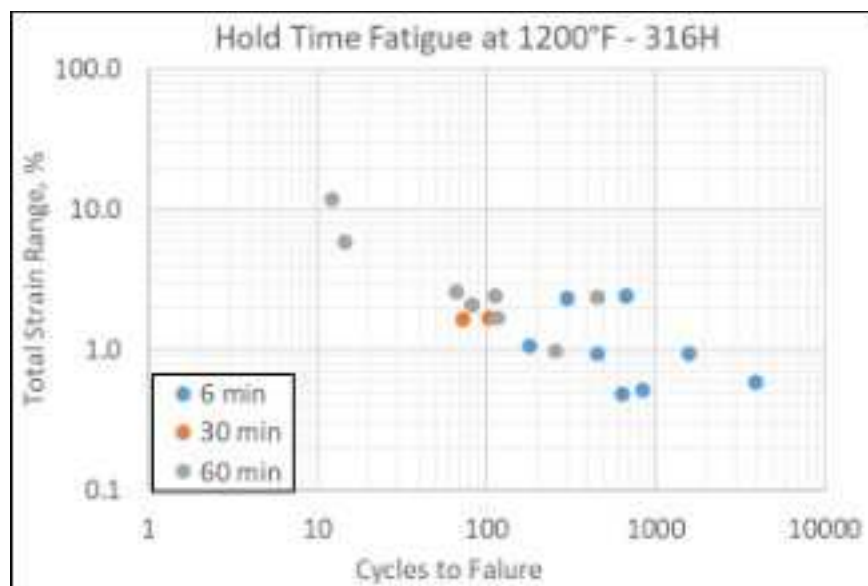
Figure 17-22: Hold Time Data (Creep Fatigue) for 316H, Temperature of 1200°F
