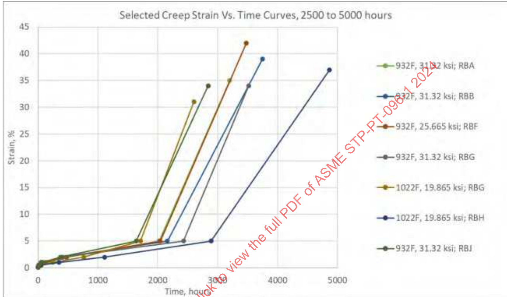
Figure 25-17: Medium-Term Strain Vs. Time Data, 2,500 to 5,000 Hour Test Durations (Type 410/12Cr)
