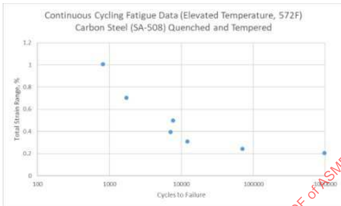
Figure 6-15: CS (SA-508) Continuous Cycling Fatigue, Elevated Temperature Data
