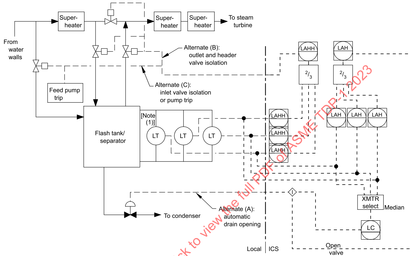
Figure 3.1.2-2 Typical Flash Tank/Separators Arrangement: ICS
