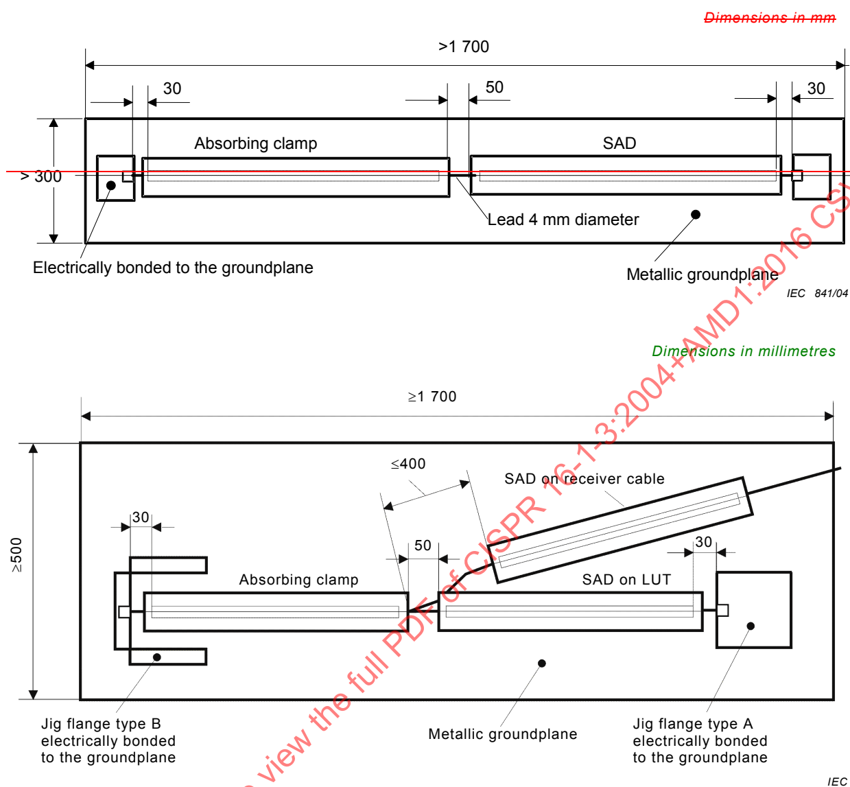
Figure B.4 – Top view of the jig
