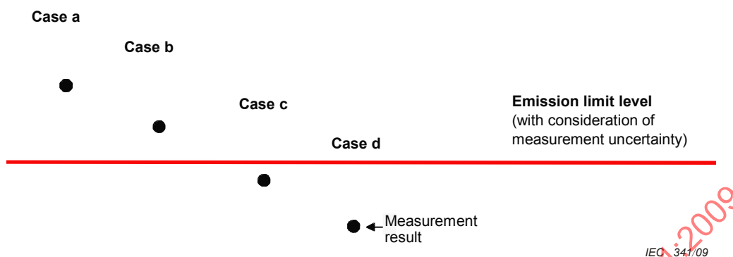
Figure 9 – Graphical representation of four cases in the compliance determination process with consideration of measurement uncertainty during limits setting.
