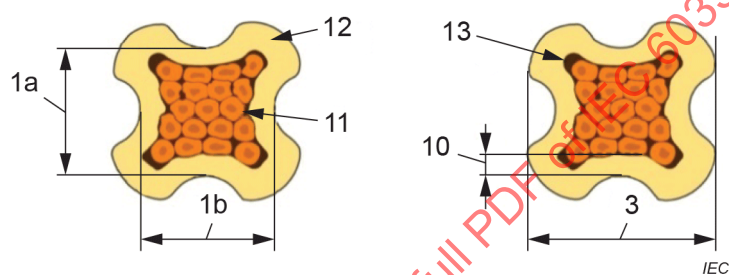
Figure A.23 – Dimensions on the microsection for closed tube and crimped cable lugs
