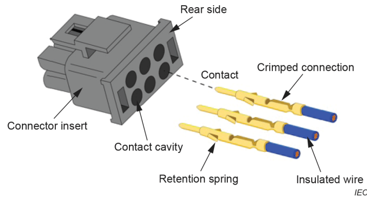
Figure A.37 – Insertion of crimped contacts into contact cavities
