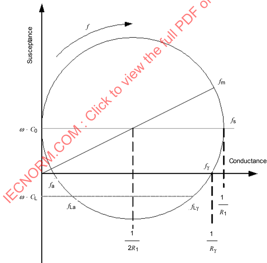
Figure 1 – Admittance of a quartz crystal unit
