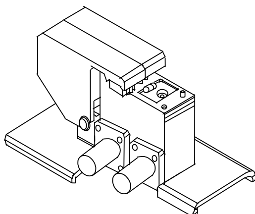
Figure 3 – Transmission \pi -network test fixture: Three-dimensional projection for the test fixture
