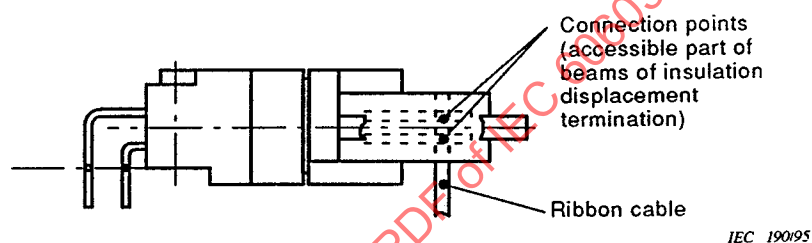
Figure 35 – Insulation displacement
