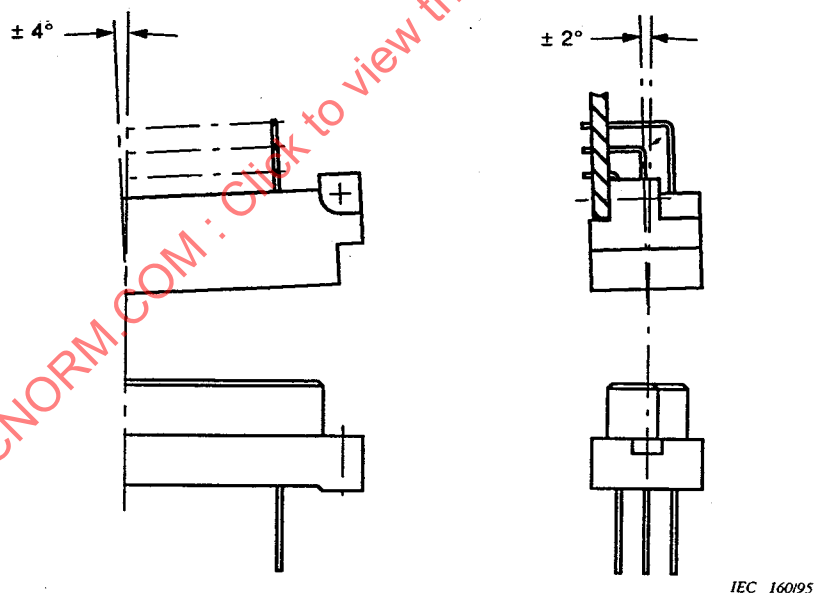
Figure 4 – Inclination
