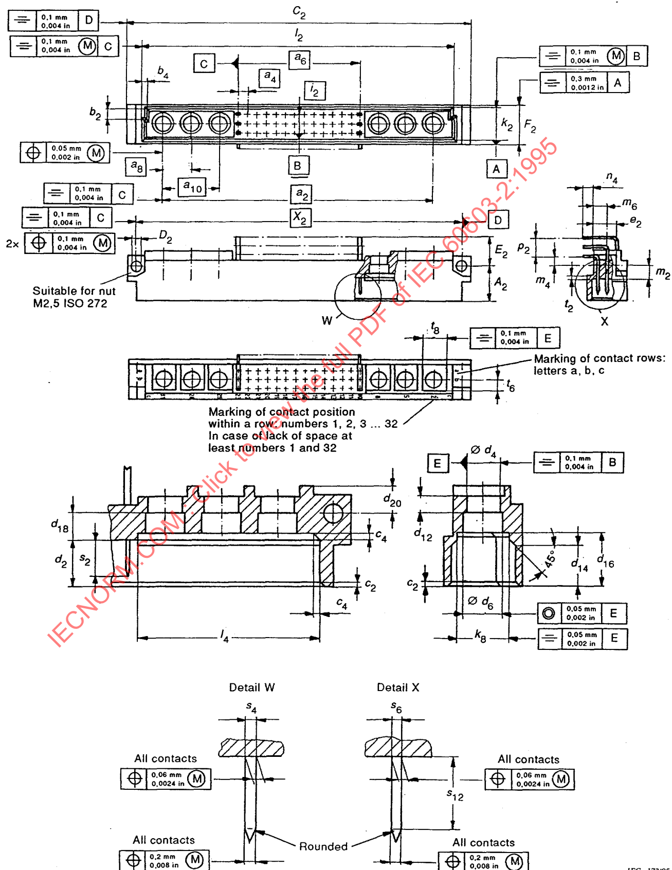
Figure 16 - Style M
