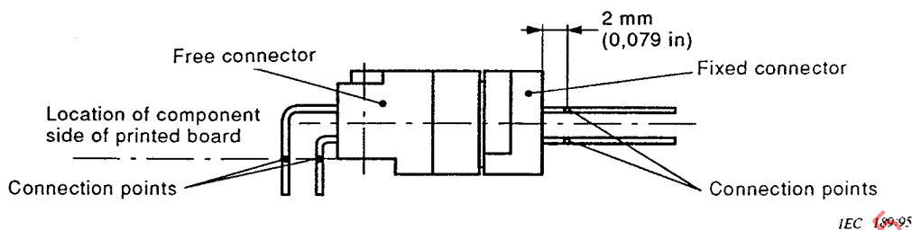
Figure 34 – Solder and wrapped connections
