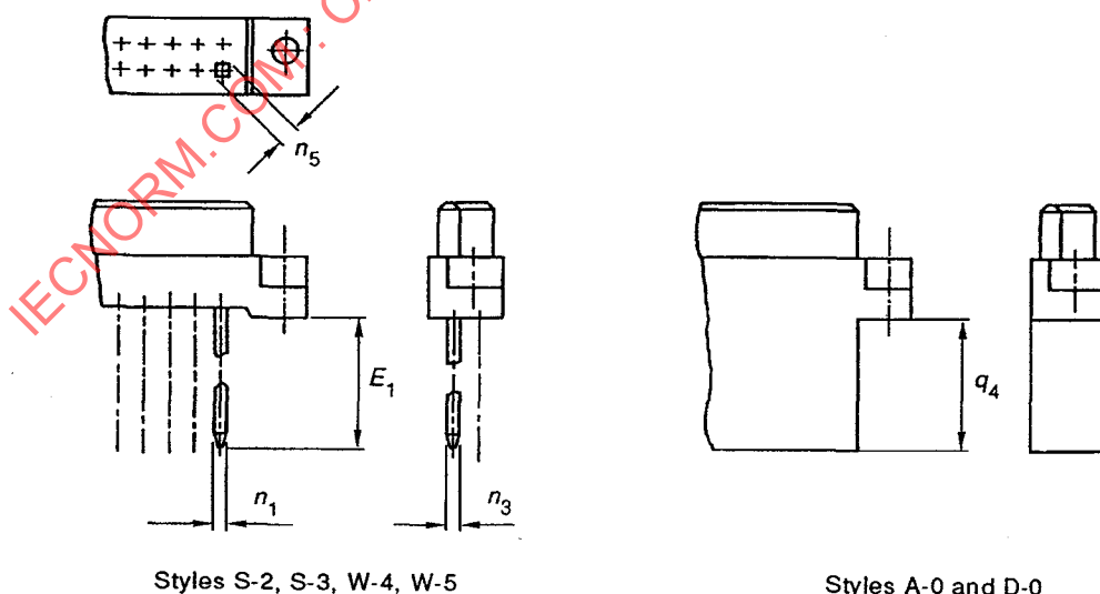
Figure 6 – Terminations
