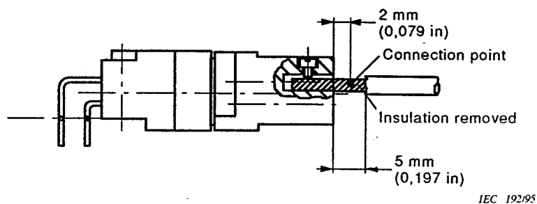
Figure 37 – Screw terminal
