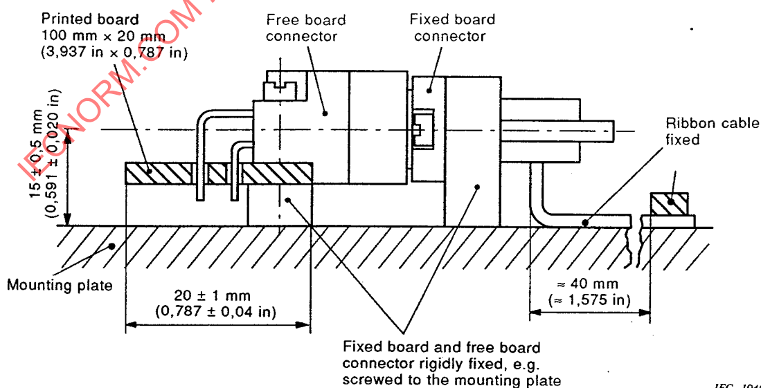
Figure 39 – Arrangement for connectors with ribbon cable (insulation displacement)
