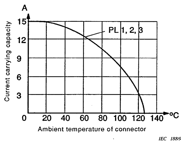
Figure 33 – Style H
