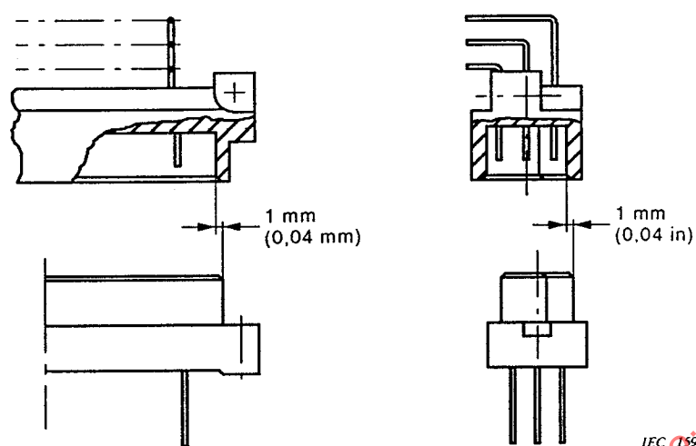
Figure 3 – Perpendicular to plug-in direction
