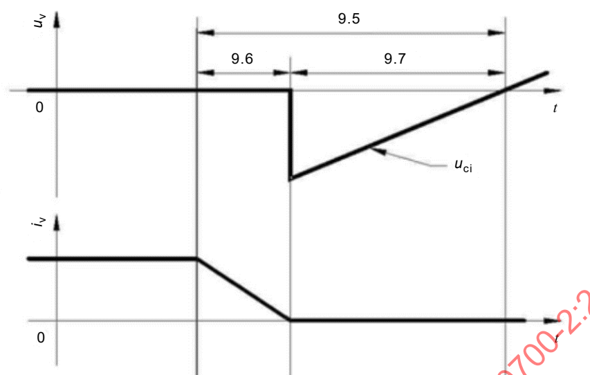
a) Valve idealized
