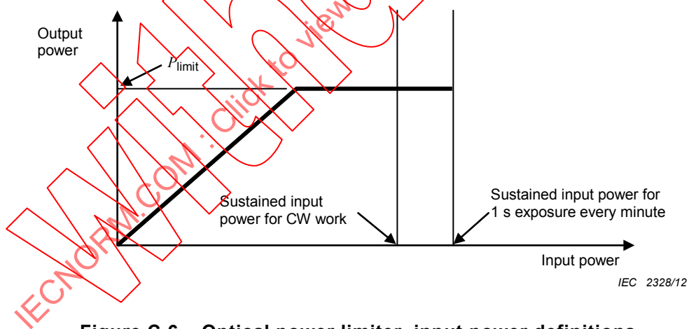
Figure C.6 – Optical power limiter, input power definitions
