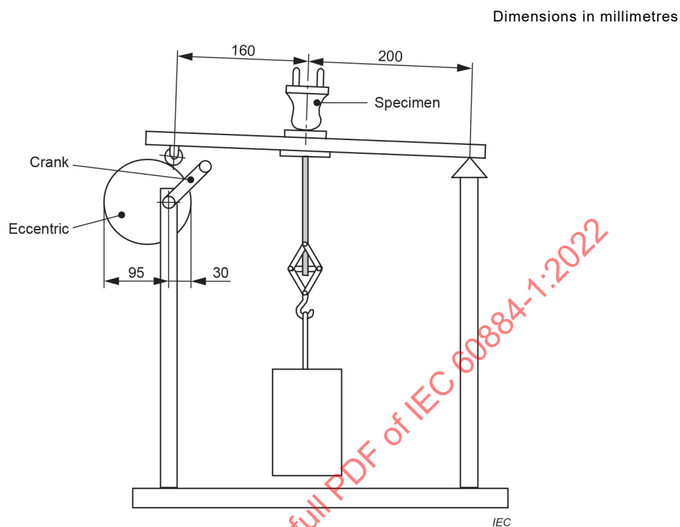
Figure 27 – Apparatus for testing cord retention
