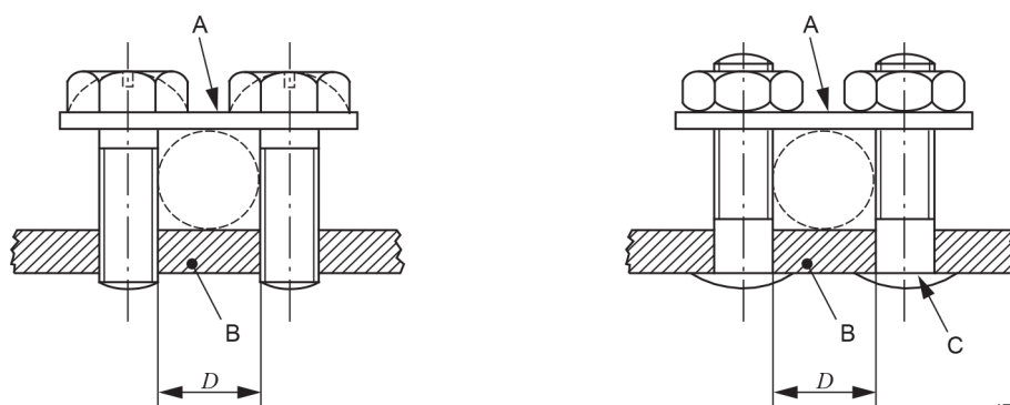
Figure 10 – Screw head terminals and stud terminals
