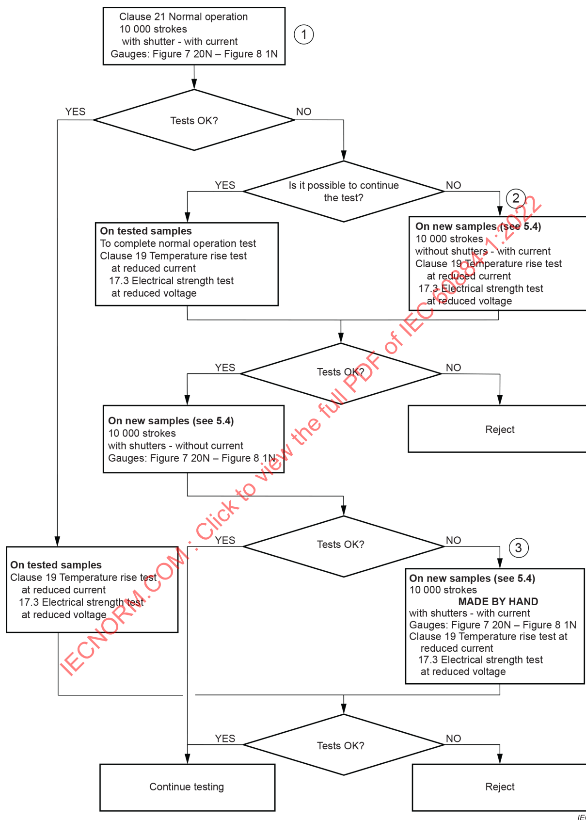
Figure 24 – Test procedures for normal operation for socket-outlets with shutters (see Clause 21)
