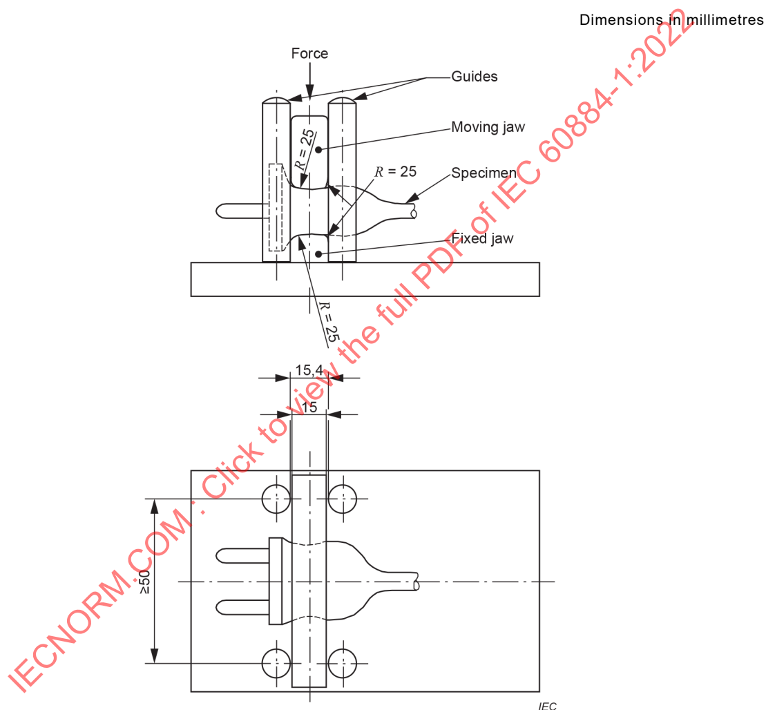
Figure 41 – Apparatus for compression test for the verification of resistance to heat specification of 25.5
