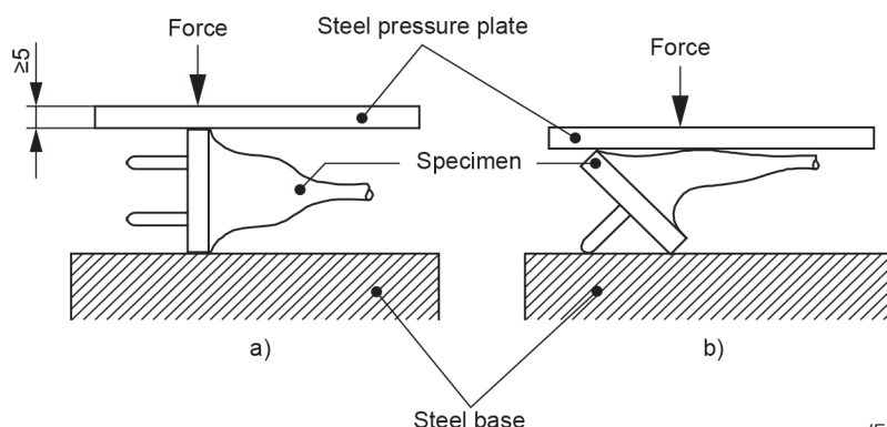
Figure 6 – Arrangement for compression test
