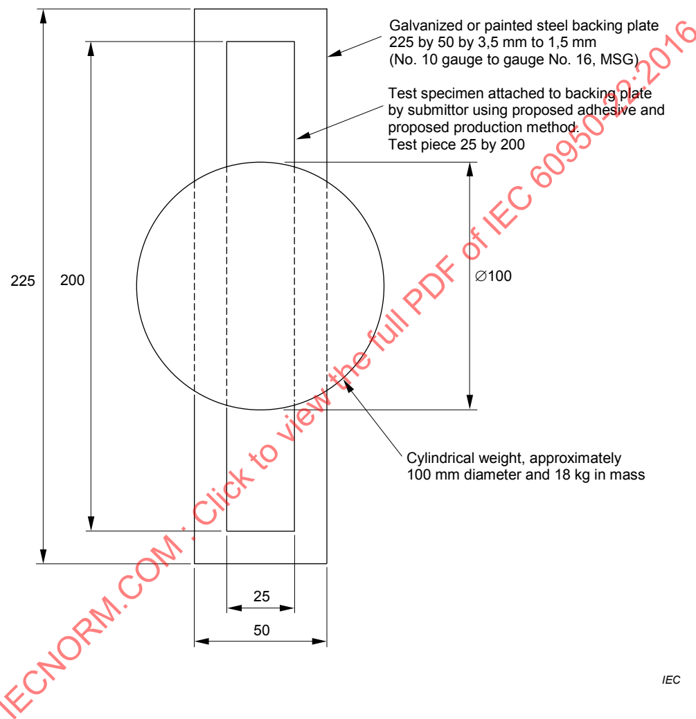
Figure D.1 – Gasket test
