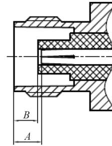
h) The interface of TNC series socket connector
