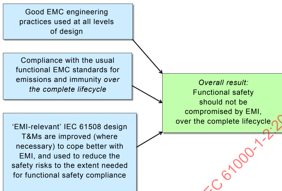
Figure B 1 –General principles recommended for design to achieve electromagnetic resilience for a complete safety-related system (where the "rugged high-specification electromagnetic mitigation approach" is not used)
