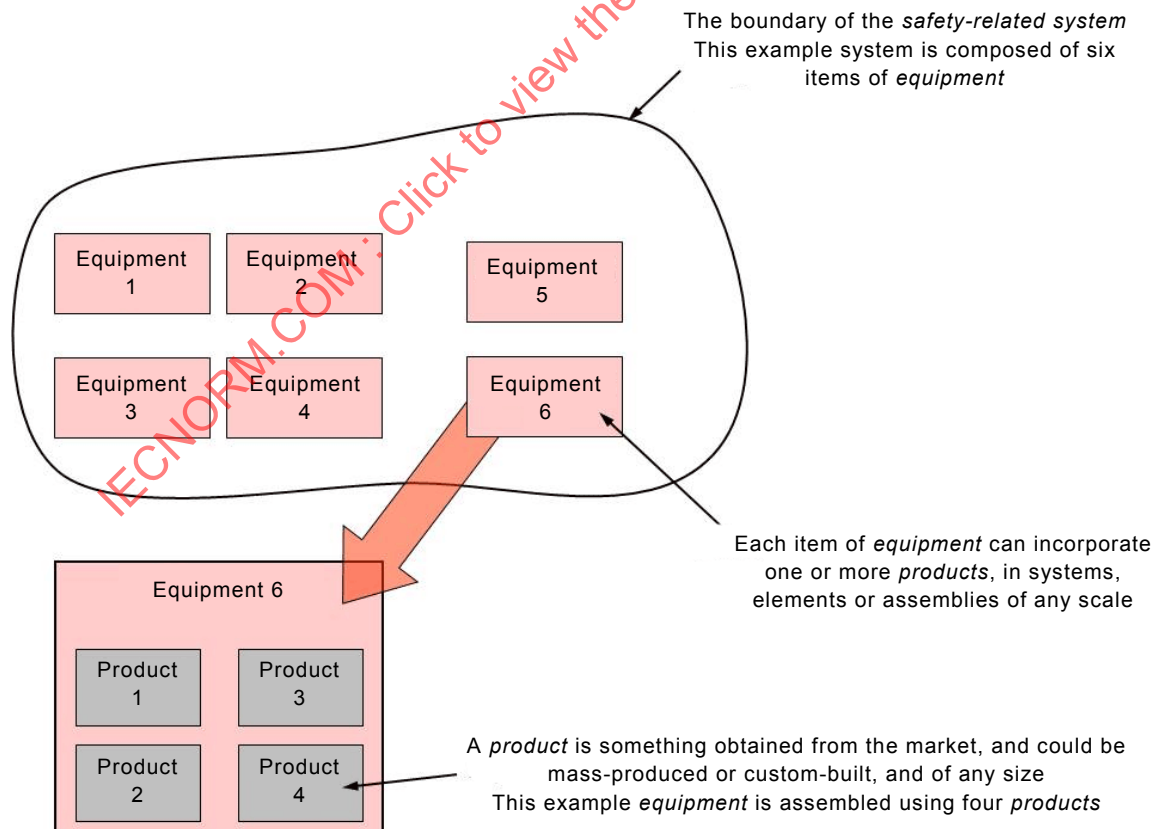
Figure D.1 – Relationships between the safety-related system, equipment and products
