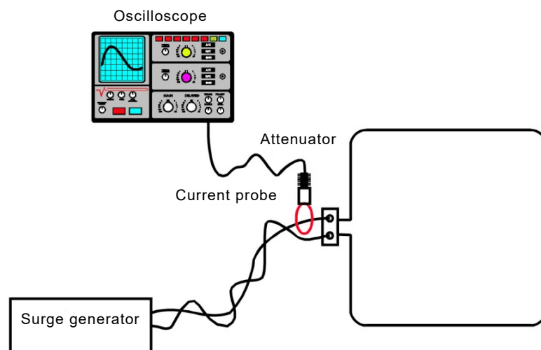
Figure 3 – Example of a current measurement of standard induction coils
