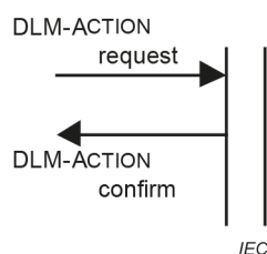
Figure 5 – Sequence of primitives for the DLM action service
