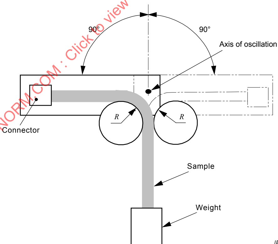
Figure 2 – Repeated bending test for cable/connector assembly
