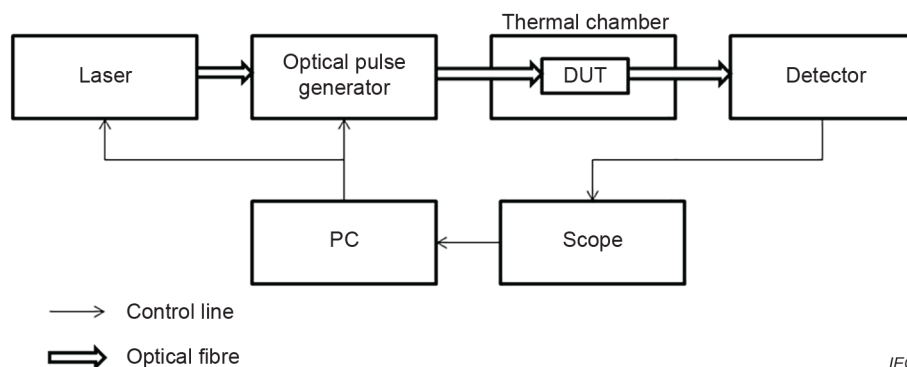
Figure E.4 – Response time testing set-up
