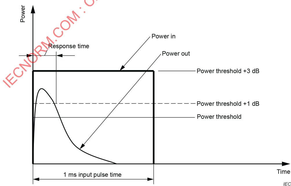
Figure E.3 – Response time curve of an optical fuse
