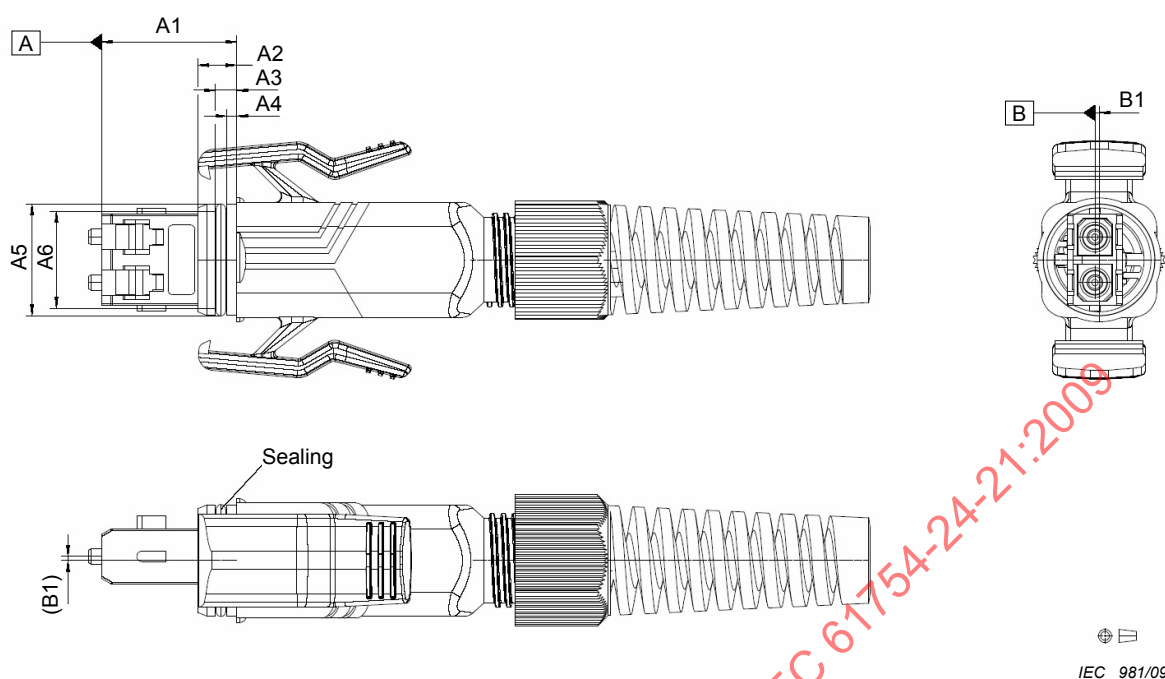
Figure 1 – Free connector (male)
