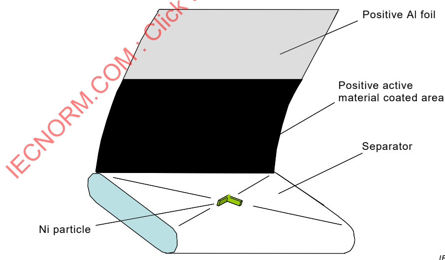
Figure A.7 – Nickel particle insertion position between positive and negative (active material) coated area of prismatic cell
