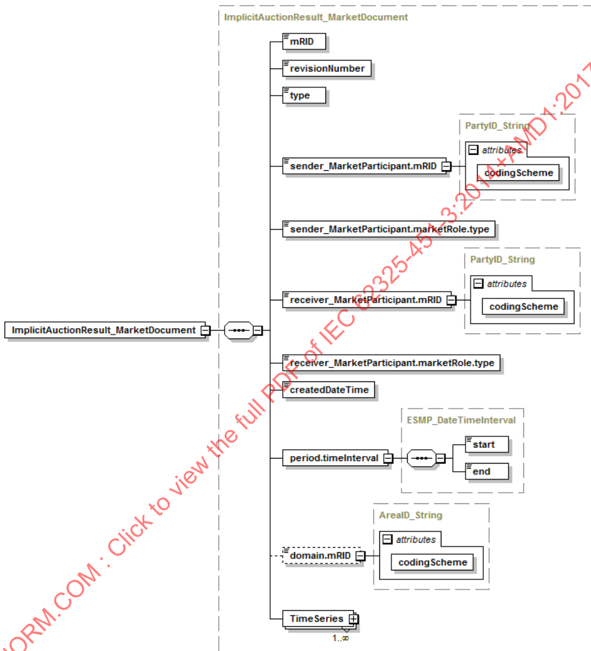
Figure 35 – Structure du schéma XML ImplicitAuctionResult_MarketDocument – 1/2
