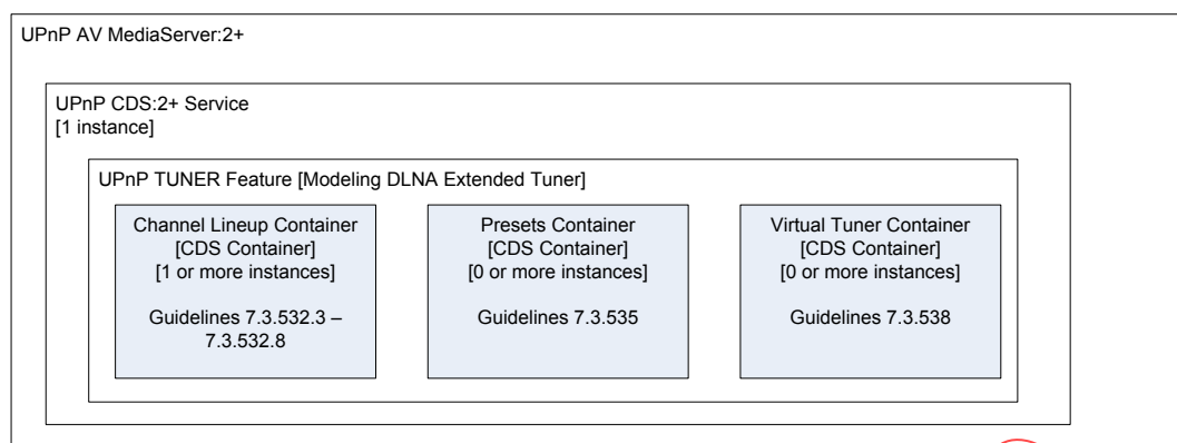
Figure 31 – Extended Tuner and its containers
