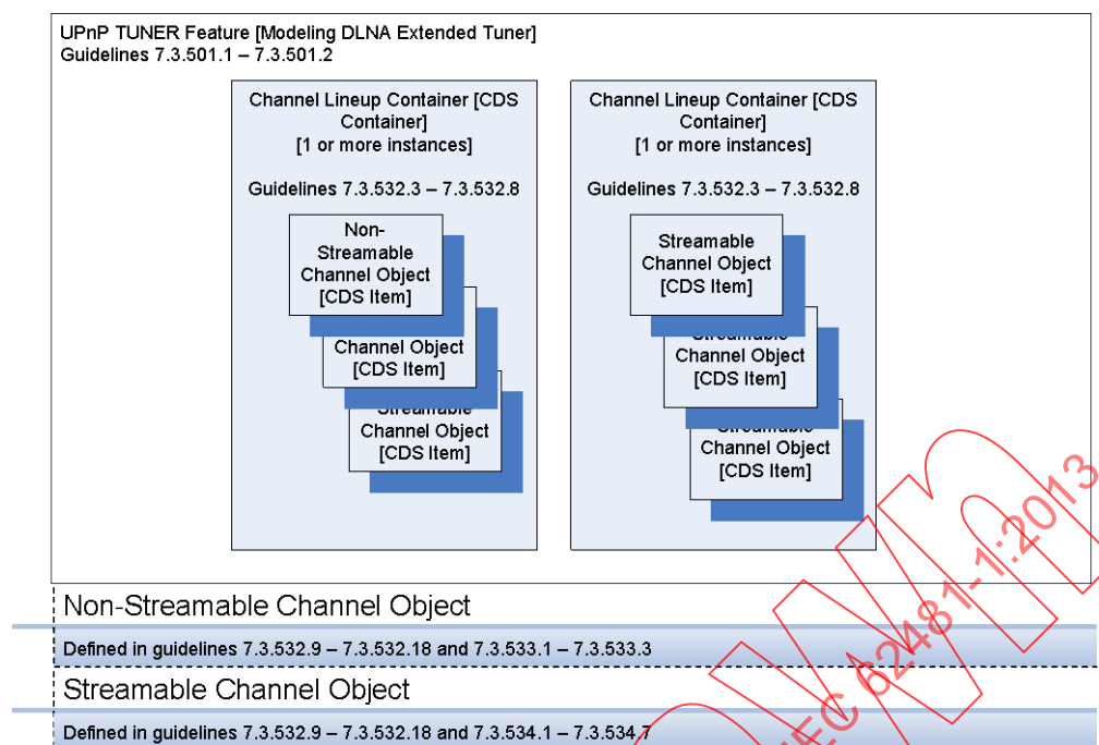
Figure 32 – Modeling DLNA Extended Tuner
