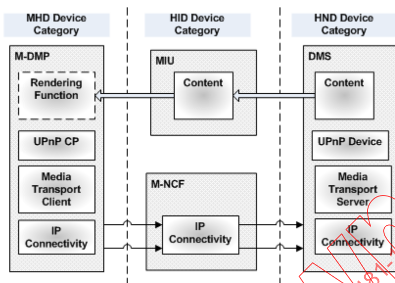
Figure 21 – 2-Box Pull System Usage interaction model between Device Categories
