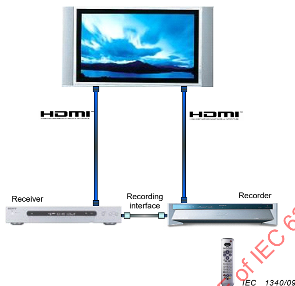
Figure A.1 – HD reception and recording device model – triggered by the recorder
