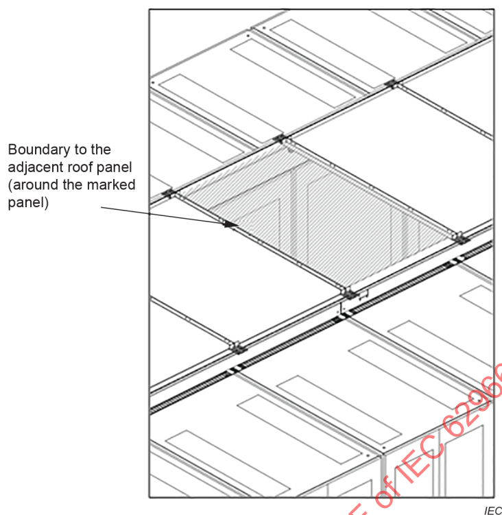
Figure 6 – Example of a connecting design to the roof
