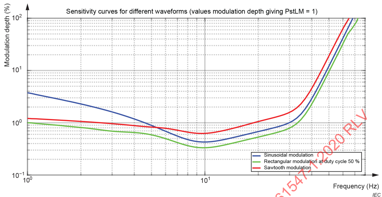
Figure A.3 – Flickermeter response to different waveshapes
