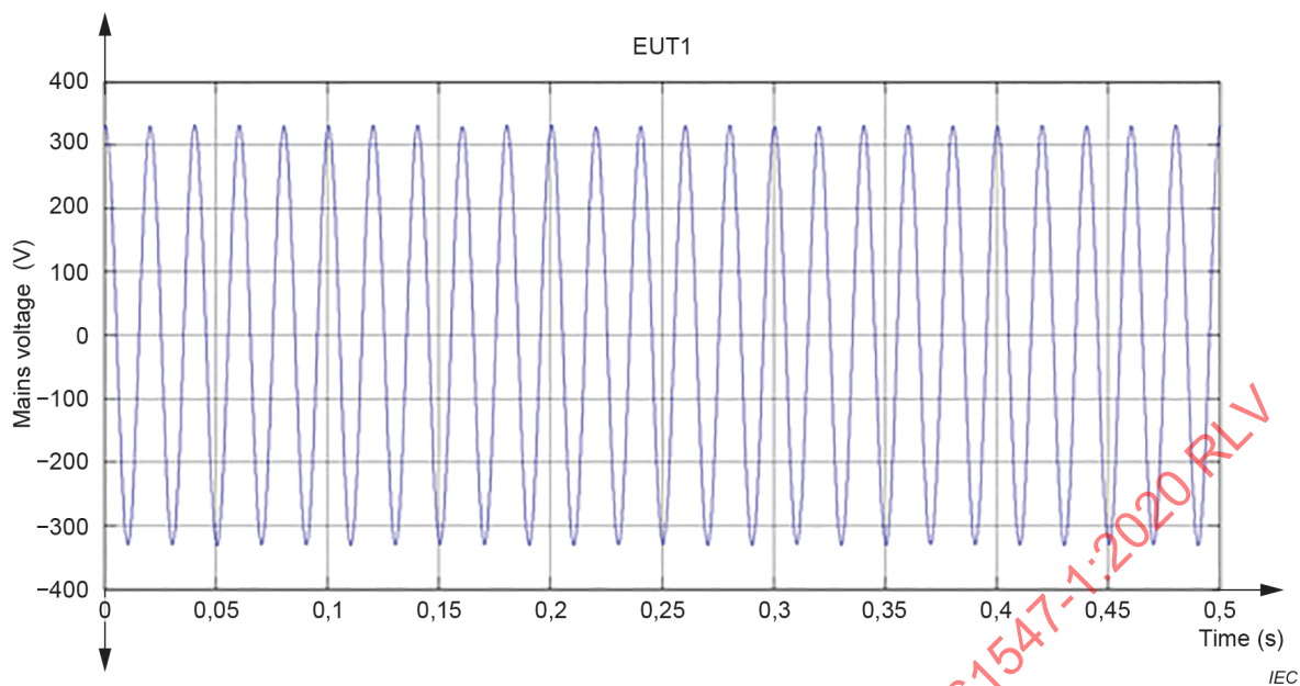
a) Mains signal with modulation d = 0,407\% at 13,5\text{ Hz} ( P_{\text{st}}^V = 1 )
