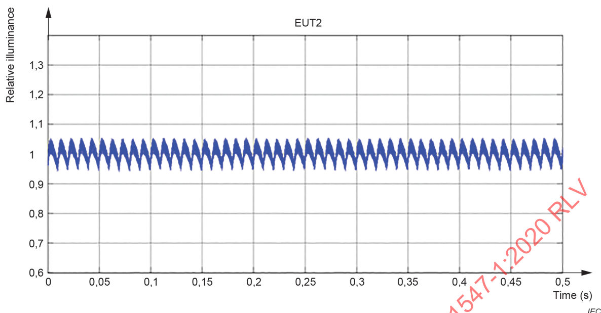
Figure C.4 – EUT2: relative illuminance – Mains voltage modulation d = 0,407 % at 13,5 Hz ( P_{st}^V = 1 )
