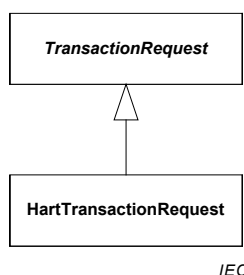
Figure 14 – HartTransactionRequest datatype
