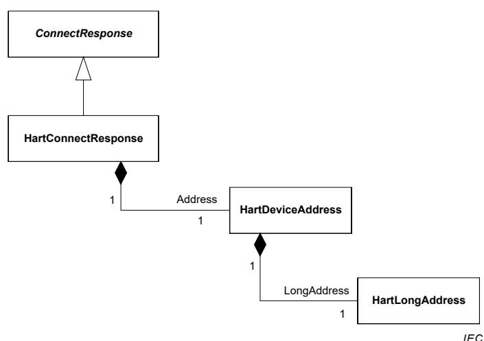
Figure 11 – HartConnectResponse datatype
