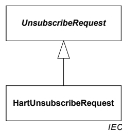
Figure 19 – HartUnsubscribeRequest datatype
