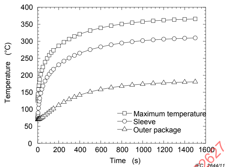
Figure 8 – Thermal simulation of fixed optical attenuator (input power: 2 W)
