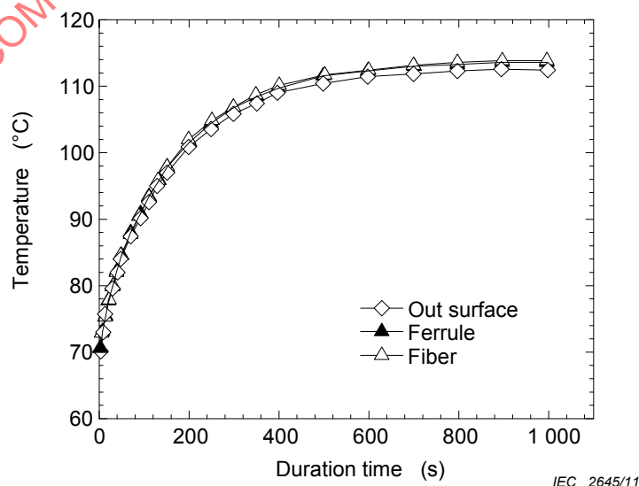
Figure 9 – Thermal simulation of optical isolator (forward direction, input power: 5 W)
