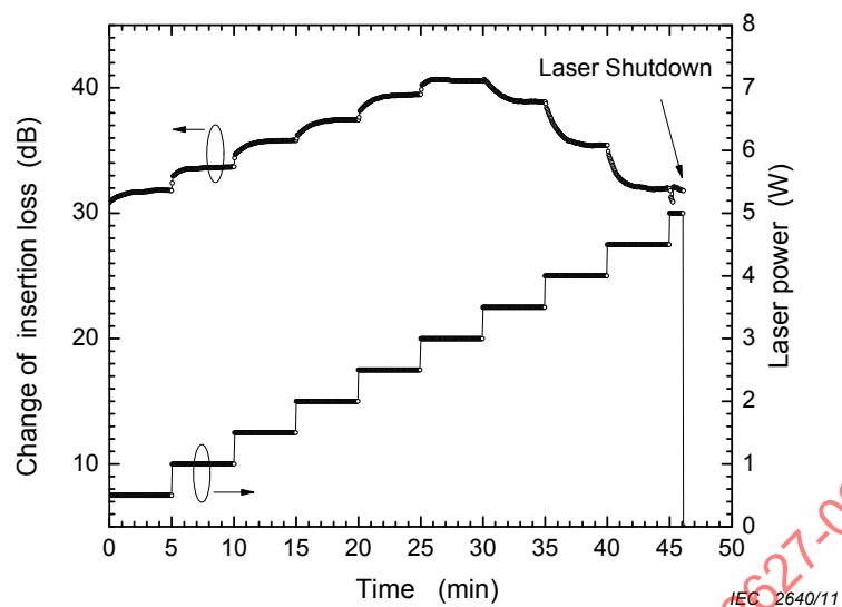
Figure 4(b) – PM2 monitor output for the measurement of IL
