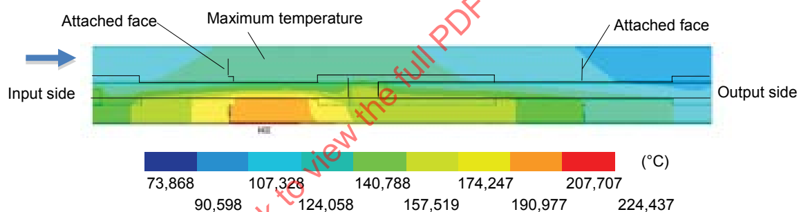
Figure 6 – Thermal distribution of fixed optical attenuator by thermal simulation (10 dB attenuator, input power: 1 W)
