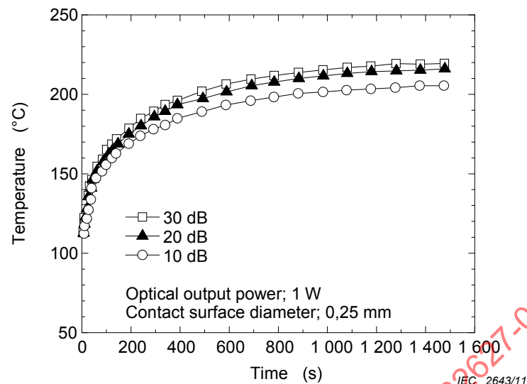
Figure 7 – Maximum internal temperature of fixed optical attenuator by thermal simulation (input power: 1 W)
