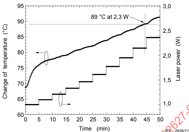
Figure 2(b) – Temperature sensor data for the surface temperature
