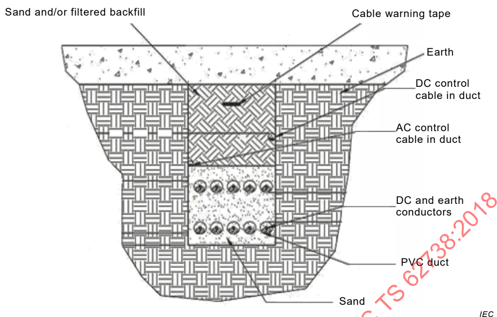
Figure 10 – Example trench diagram with cables in ducts
