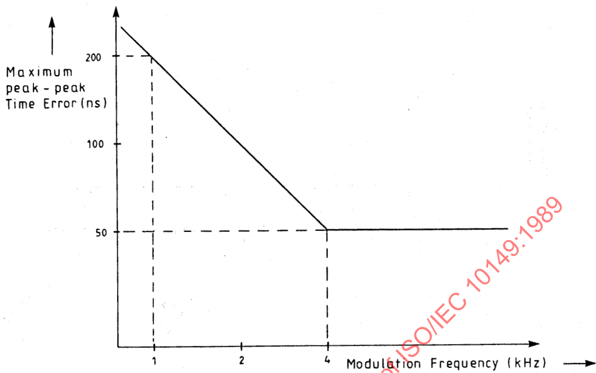
Figure 7 — Position jitter of the Channel bits versus the modulation frequency
